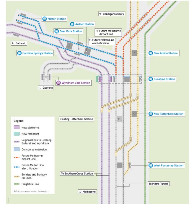
Melbourne Airport Rail Stage 1: West Footscray to Albion Rail Upgrade project alignment map
