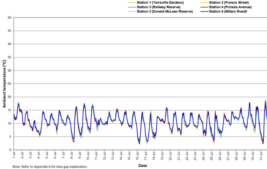
Figure 12: Ambient temperature (1 hour average) All AAQMS – July 2020
