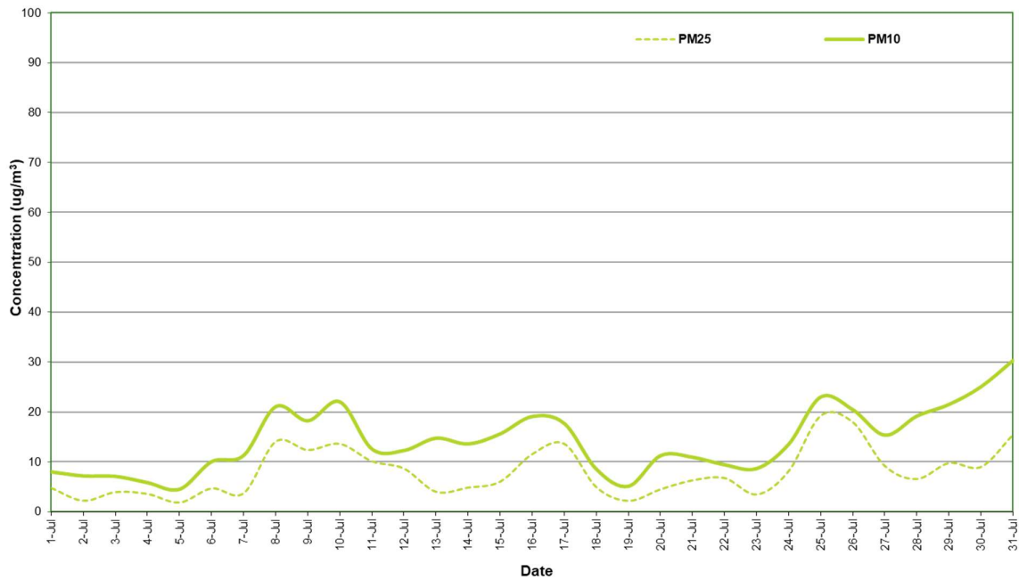
Figure 2: Station 1 PM 2.5 and PM 10 concentration (24 hour average) – July 2020
