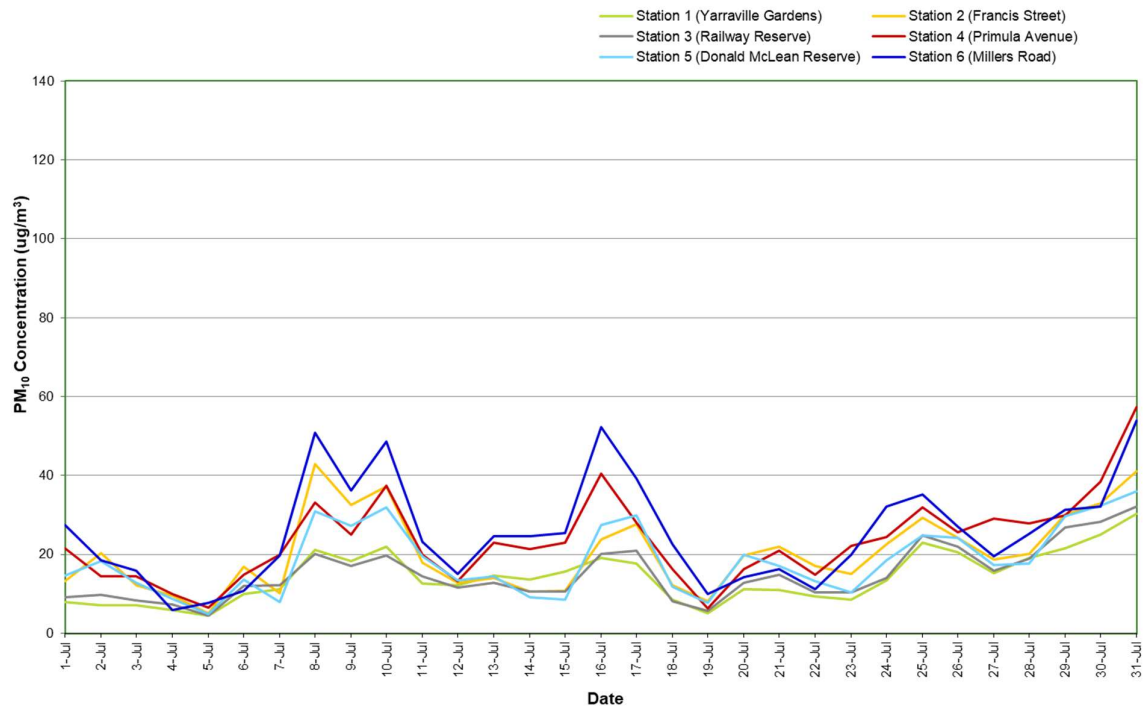
Figure 9: Combined PM 10 concentration (24 hour average) – July 2020
