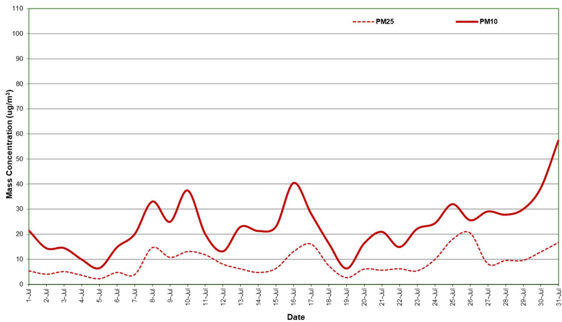
Figure 5: Station 4 PM 2.5 and PM 10 concentration (24 hour average) – July 2020
