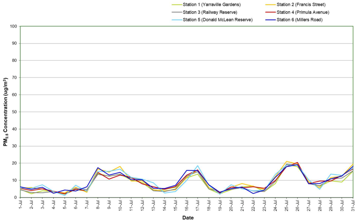
Figure 8: Combined PM 2.5 concentration (24 hour average) – July 2020
