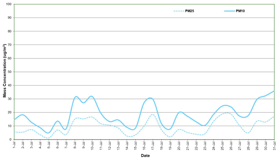
Figure 6: Station 5 PM 2.5 and PM 10 concentration (24 hour average) – July 2020
