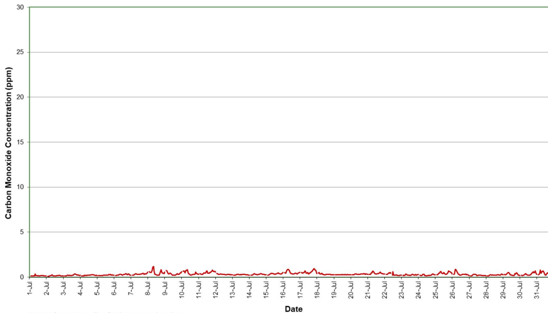
Figure 11: Station 4 CO concentration (1 hour average) – July 2020
