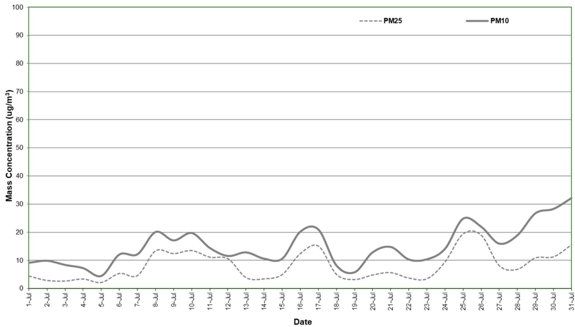
Figure 4: Station 3 PM 2.5 and PM 10 concentration (24 hour average) – July 2020
