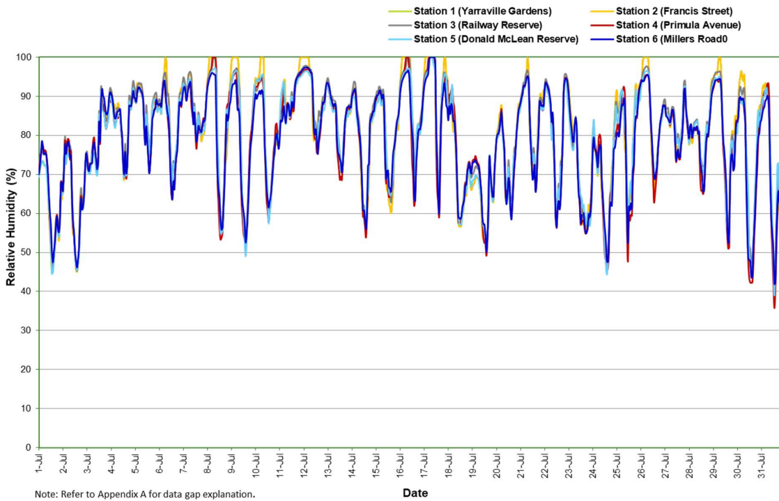
Figure 13: Relative humidity (1 hour average) All AAQMs – July 2020
