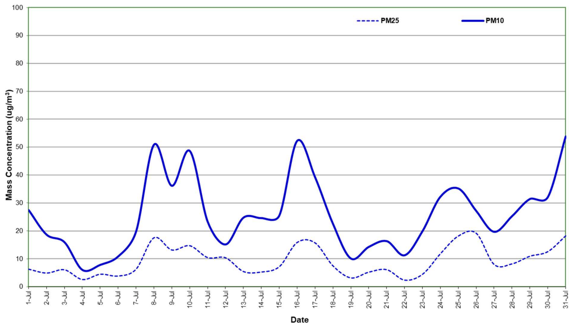
Figure 7: Station 6 PM 2.5 and PM 10 concentration (24 hour average) – July 2020
