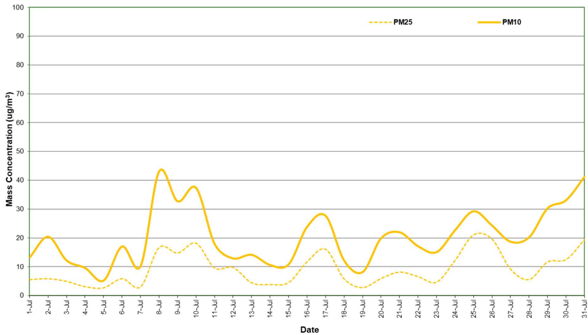
Figure 3: Station 2 PM 2.5 and PM 10 concentration (24 Hour Average) – July 2020
