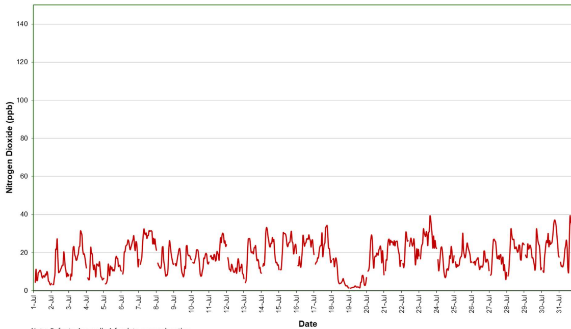
Figure 10: Station 4 NO 2 concentration (1 hour average) – July 2020
