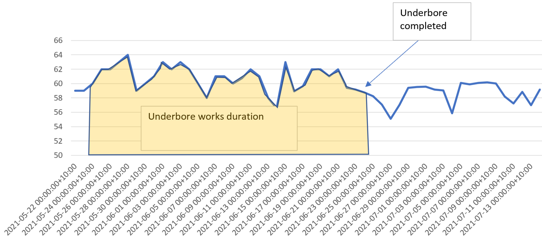
East Portal - precinct noise daily average levels during underbore works (mid May - 24/6)
