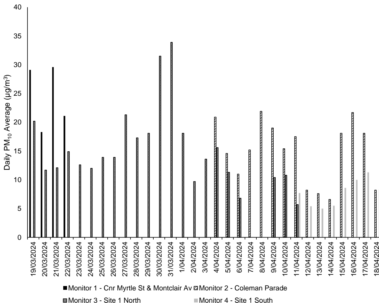
Figure 6: Burwood PM 10 daily averages
