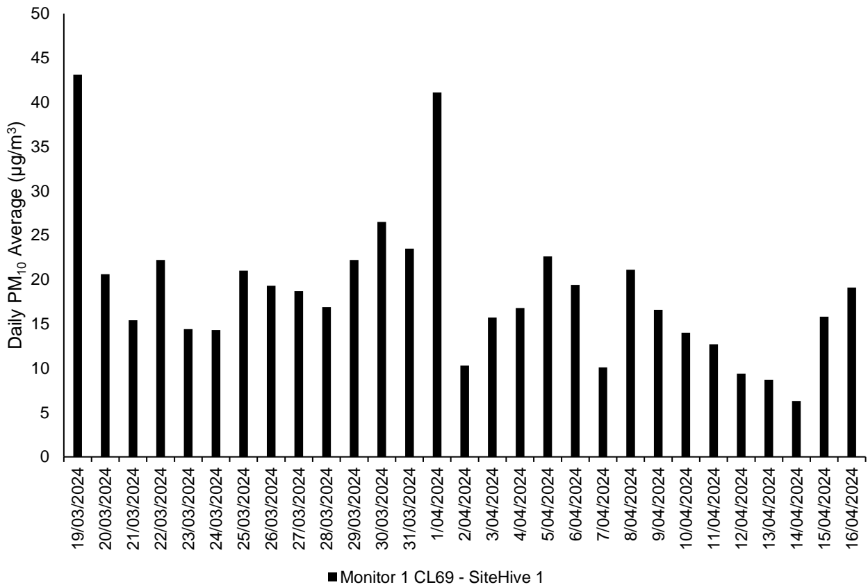
Figure 10: Clayton PM 10 daily averages
