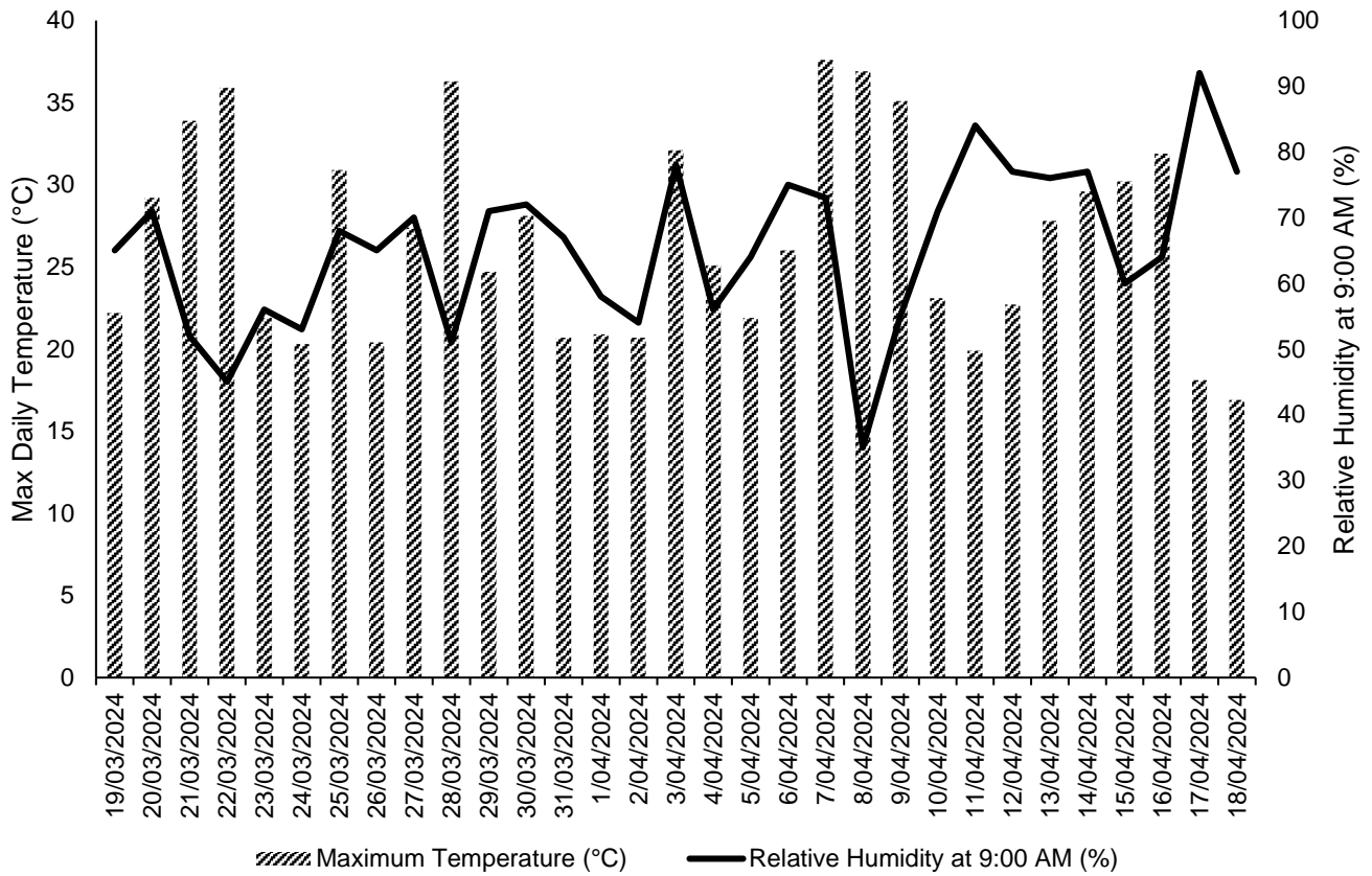
Figure 15: Daily relative humidity and temperature observations for Melbourne (Olympic Park), Victoria 19 March 2024 –18 April 2024. Data Source BOM.
