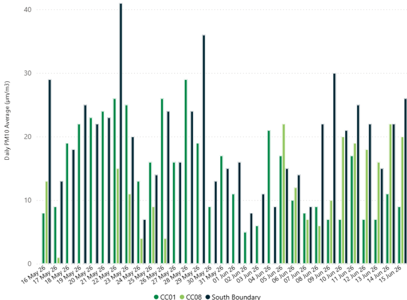
Figure 6: Daily Averages PM 10 Results at Clarinda TBM Launch Site
