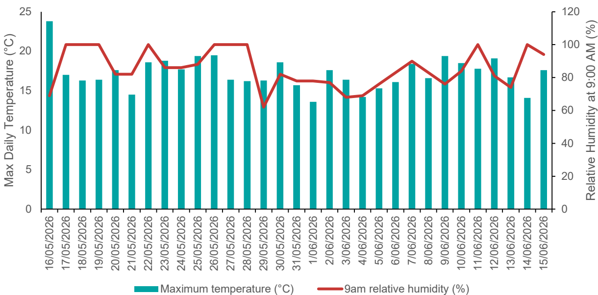
Figure 7: Daily relative humidity and temperature observations for Melbourne (Olympic Park), Victoria 16/05/2026 – 15/06/2026. Data Source BOM.
