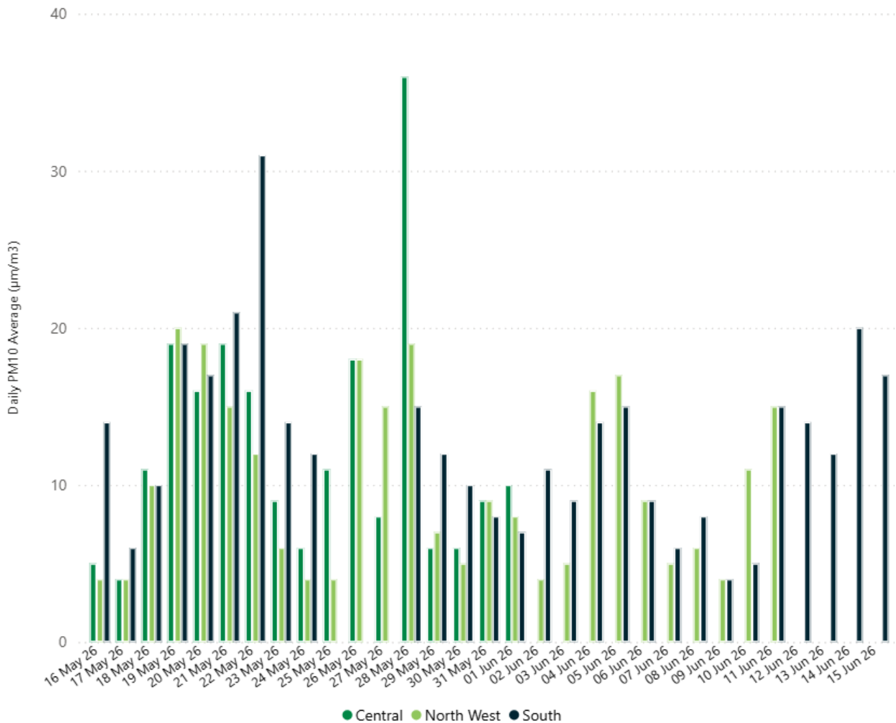
Figure 8: Daily Averages PM 10 Results at Clayton Site
