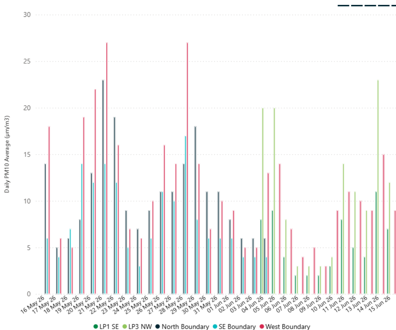
Figure 10: Daily Averages PM 10 Results at Monash
