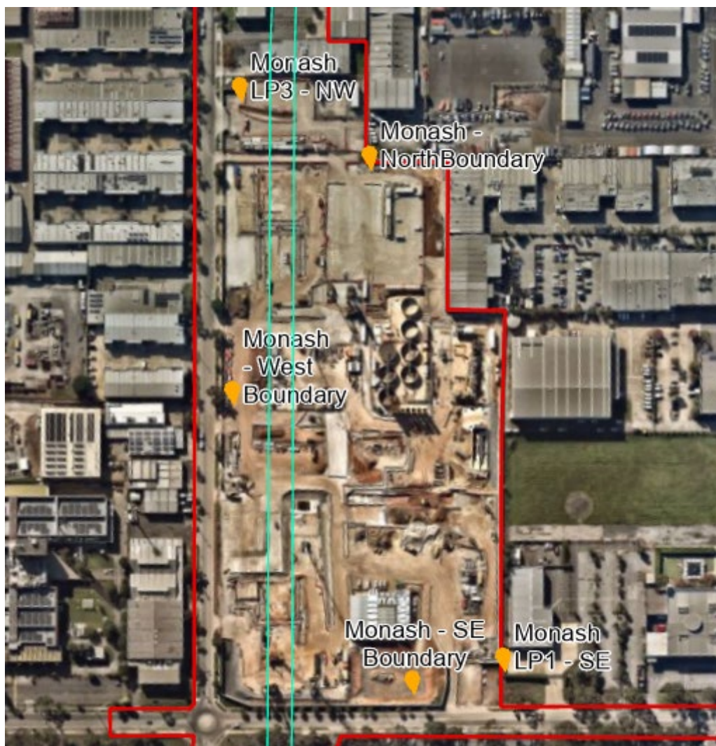
Figure 9: Monash air quality monitoring stations
