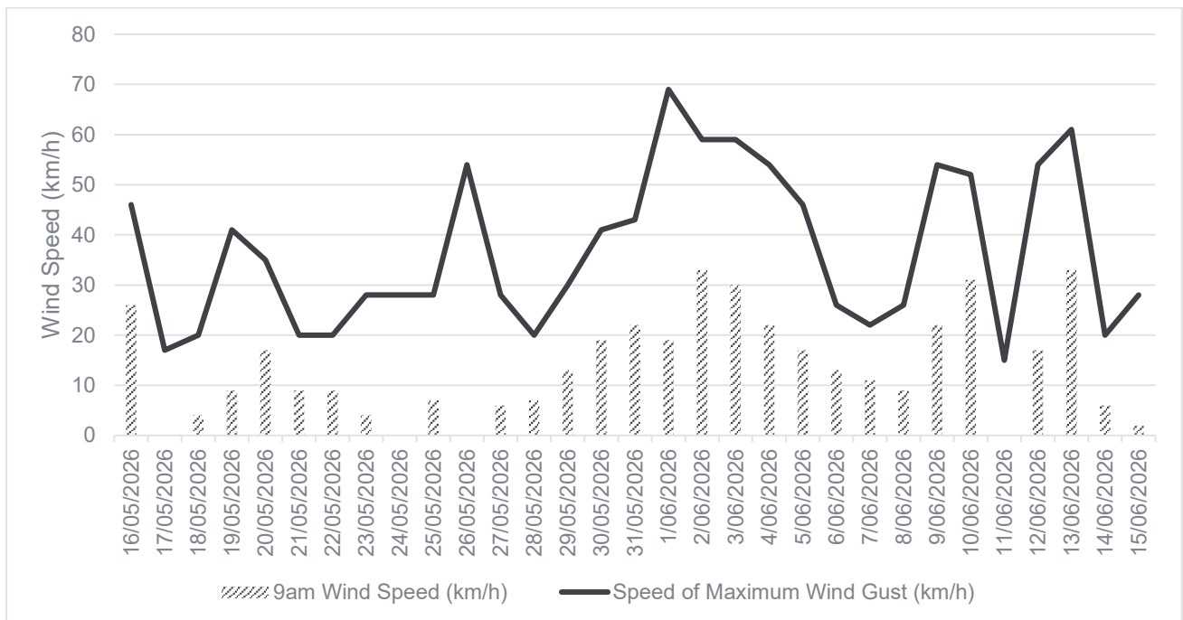
Figure 12: Daily wind speed observations for Moorabbin, Victoria
