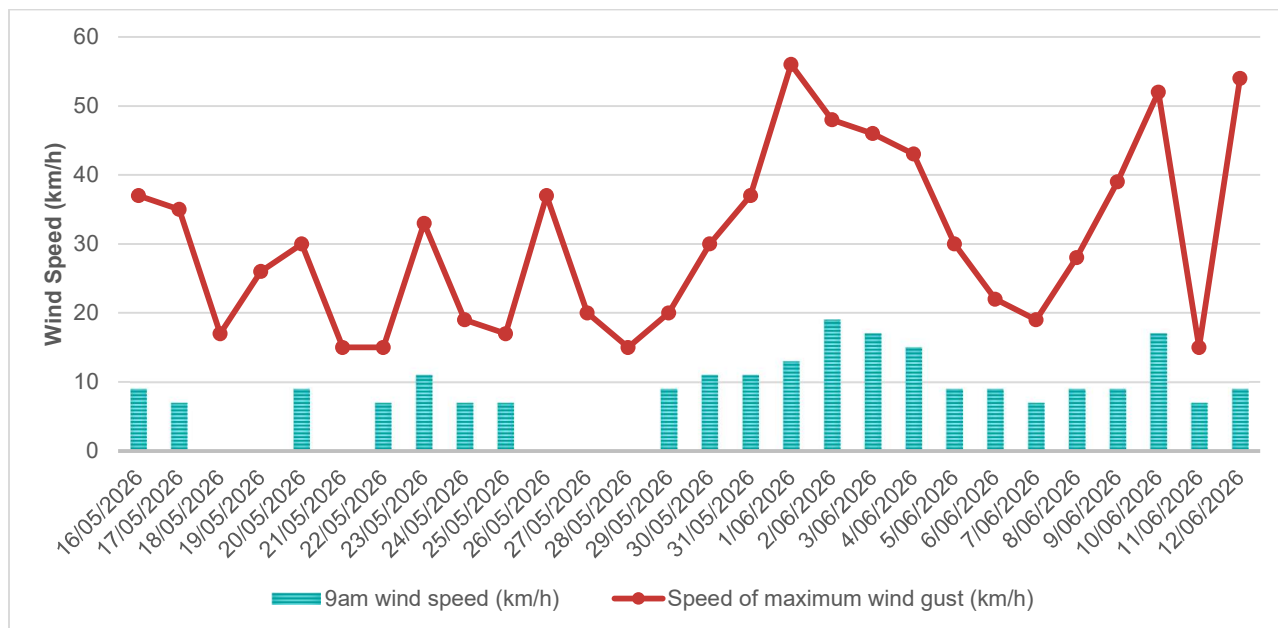
Figure 8. Daily wind speed observations for Melbourne (Olympic Park), Victoria 16/05/2026 – 15/06/2026. Data Source BOM.
