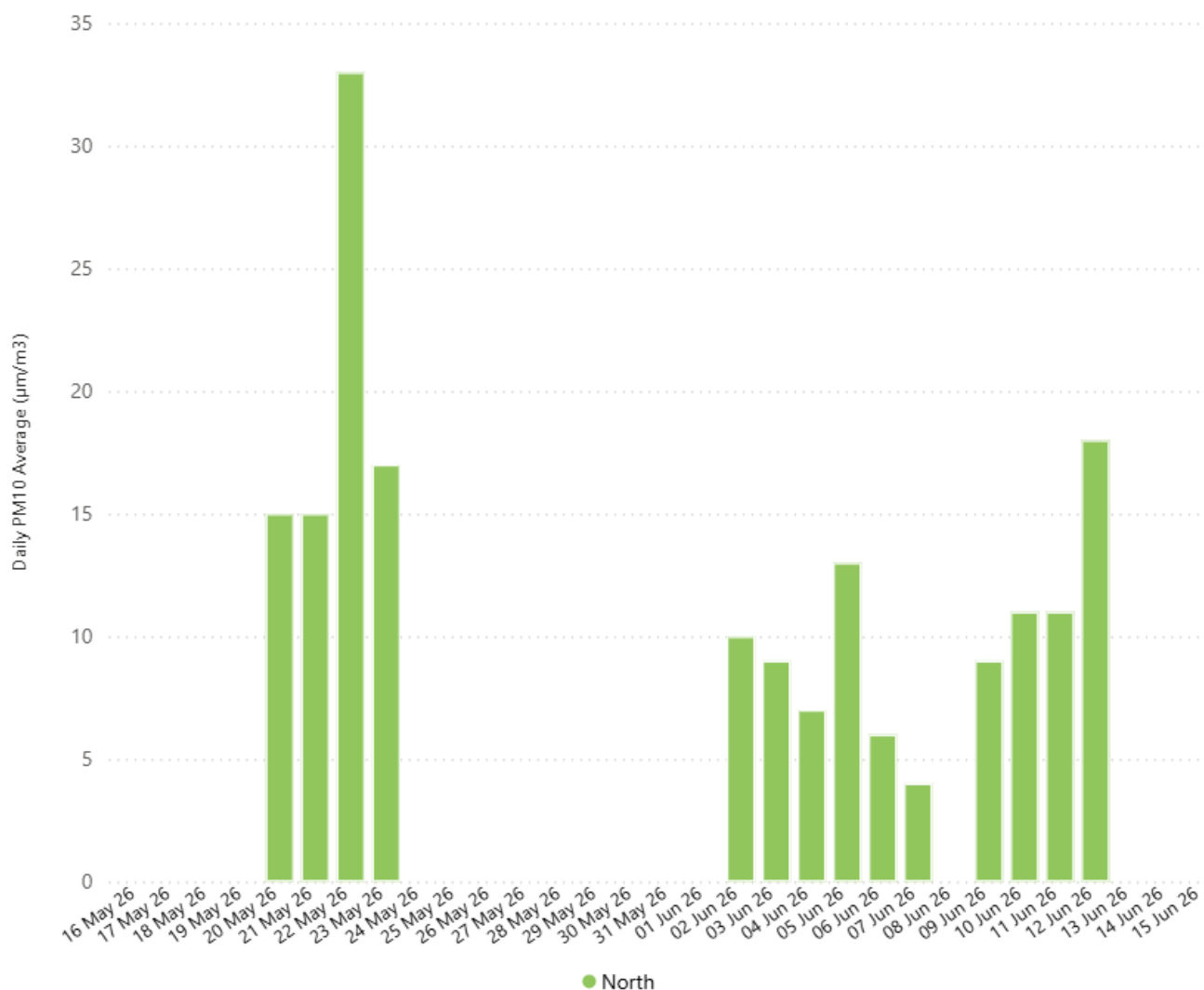
Figure 2: Daily Averages PM 10 Results at Cheltenham
