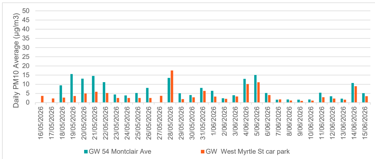
Figure 6. Glen Waverley PM 10 daily averages from 16 May to 15 June
