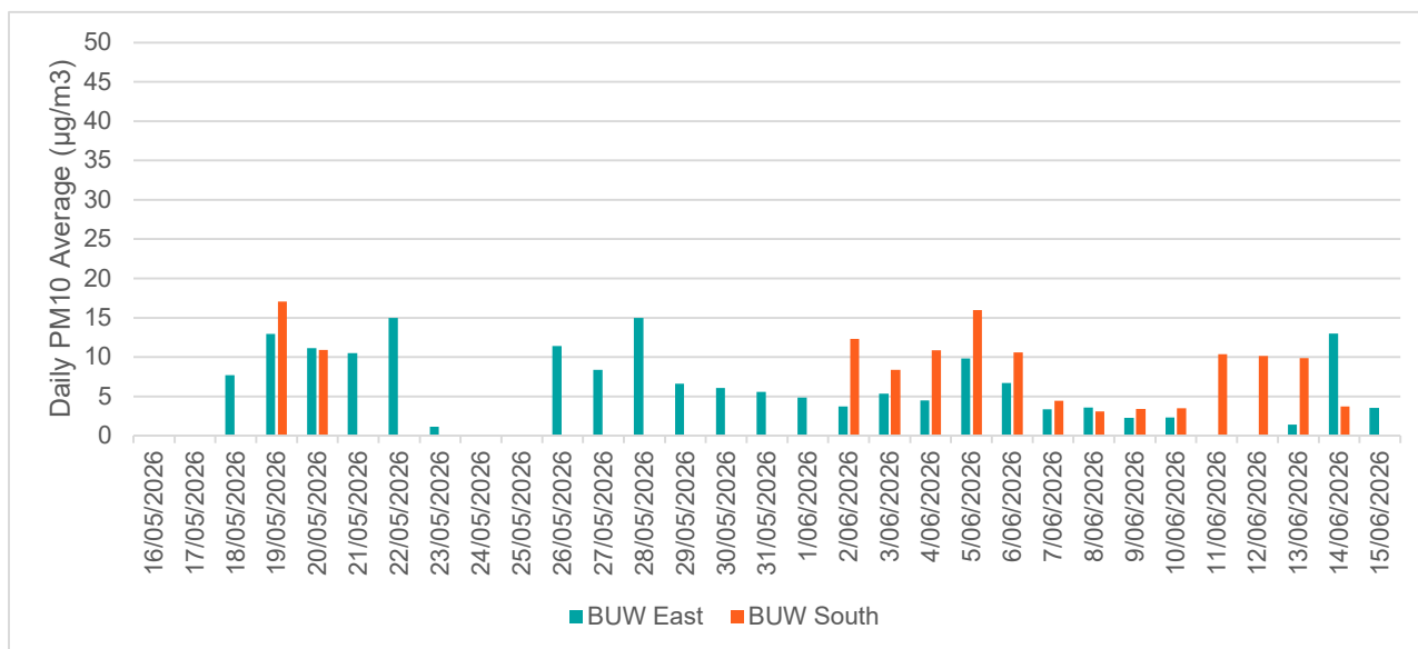
Figure 4. Burwood PM 10 daily averages from 16 May to 15 Jun
