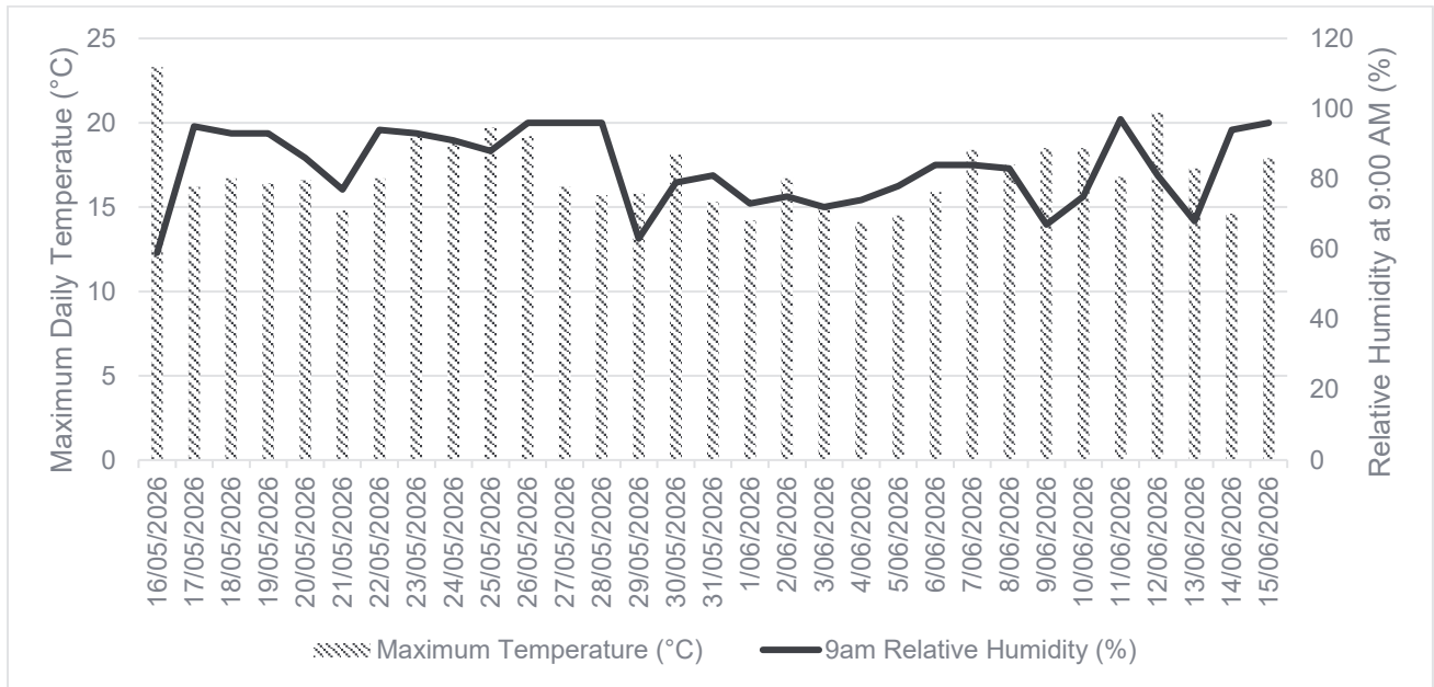
Figure 11: Daily relative humidity and temperature observations for Moorabbin, Victoria
