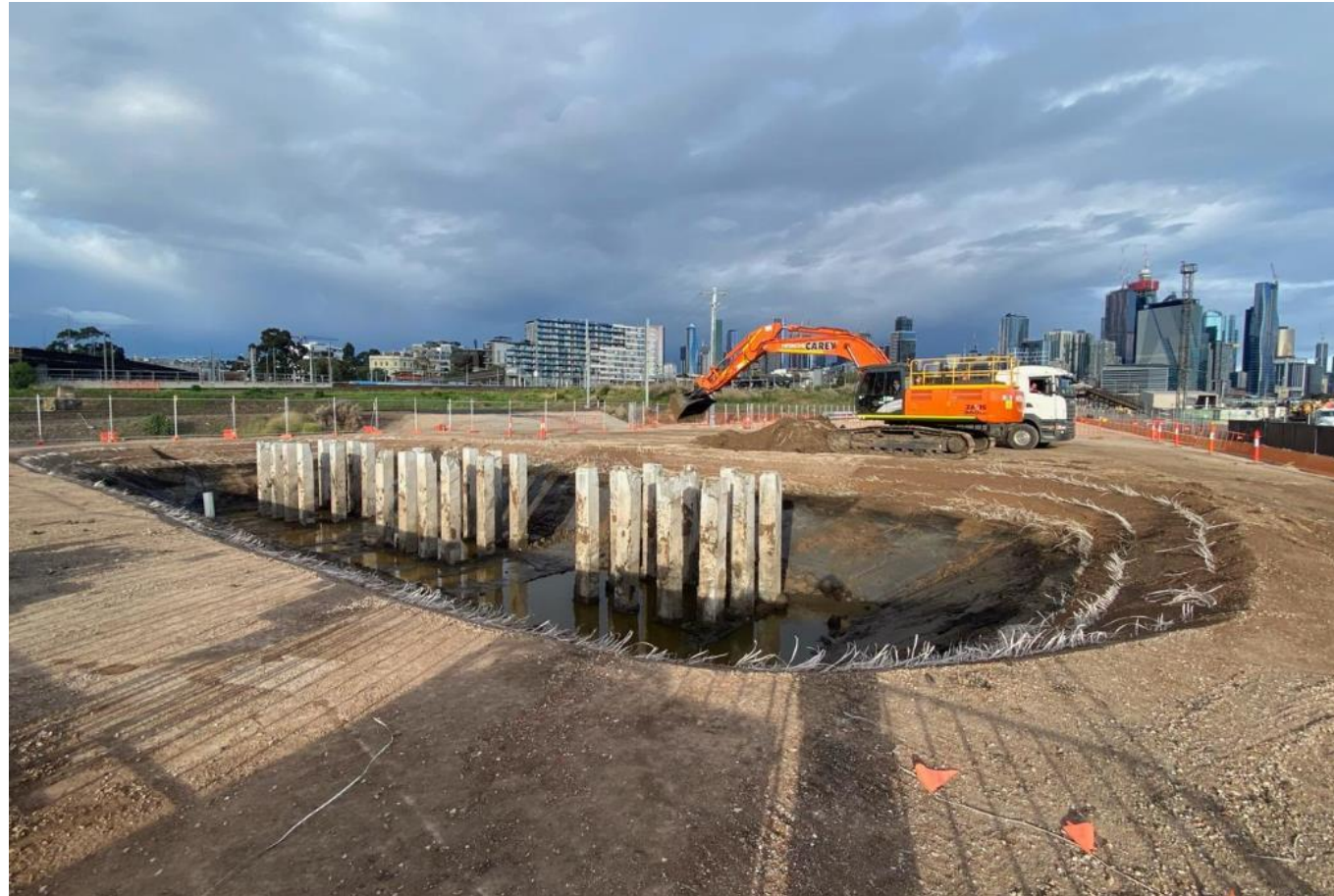
Pile cap excavation works - Wurundjeri Way Extension bridge
