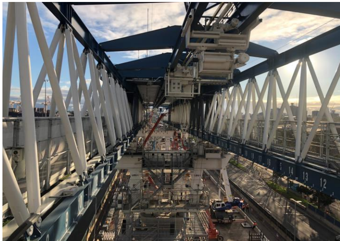
Successful installation of the Launching Gantry
