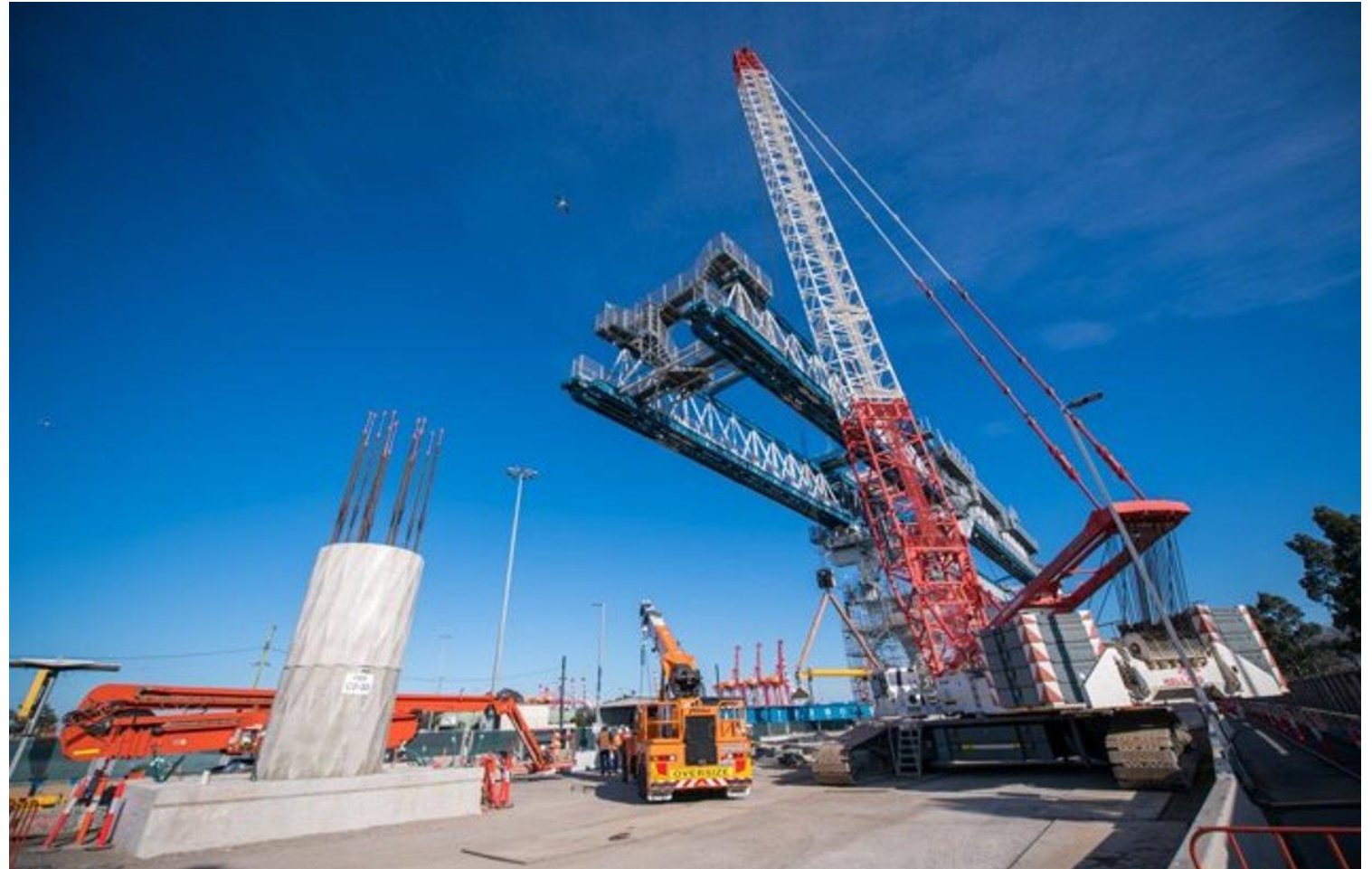
Footscray Road launching gantry
