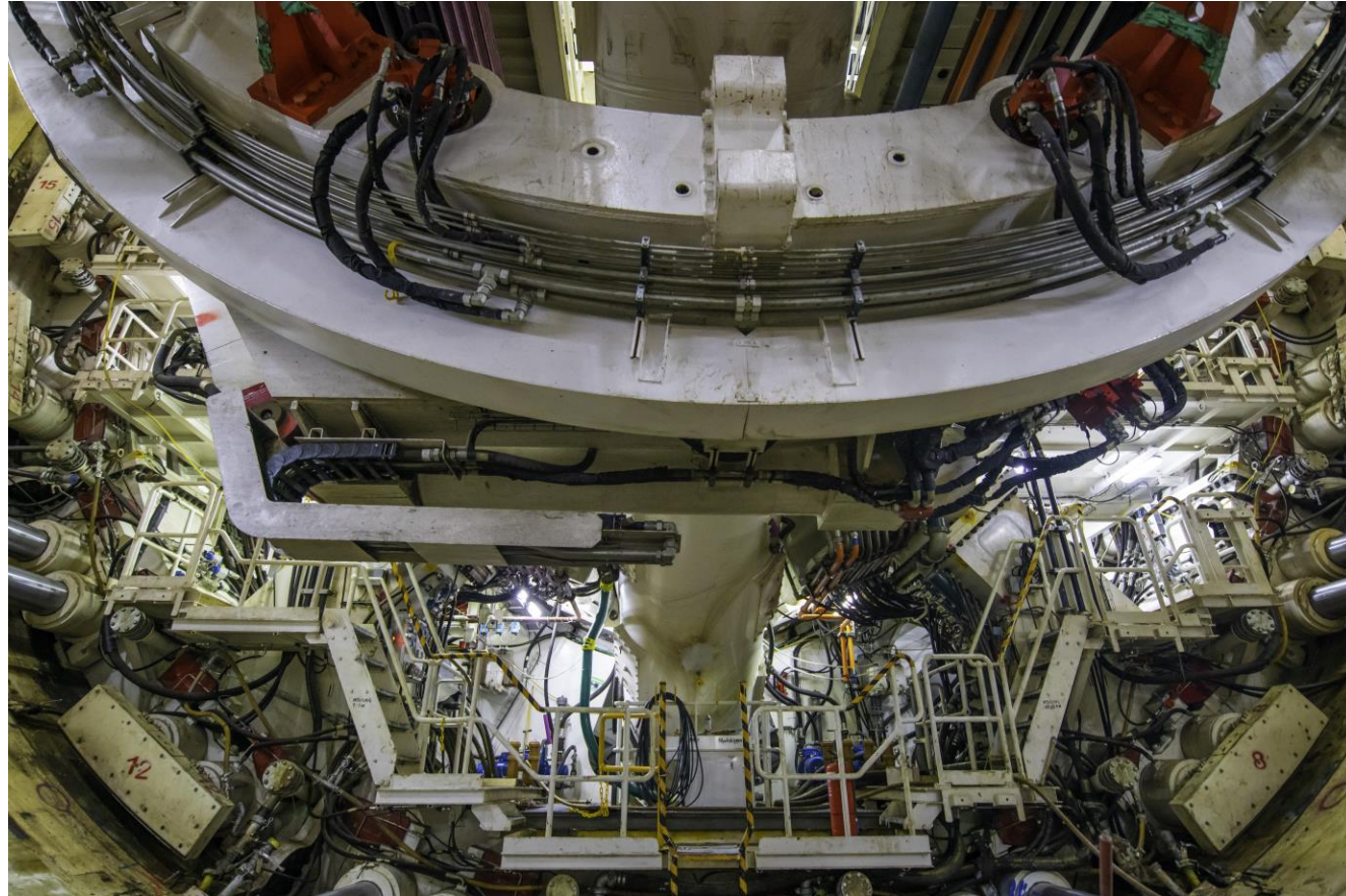
TBM segment erector
