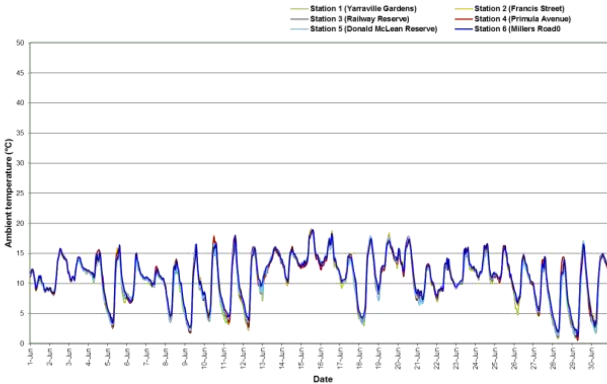
Figure 12: Ambient temperature (1 hour average) All AAQMS – June 2020
