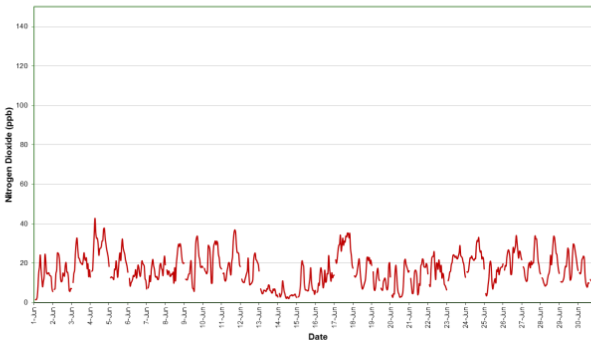
Figure 10: Station 4 NO 2 concentration (1 hour average) – June 2020
