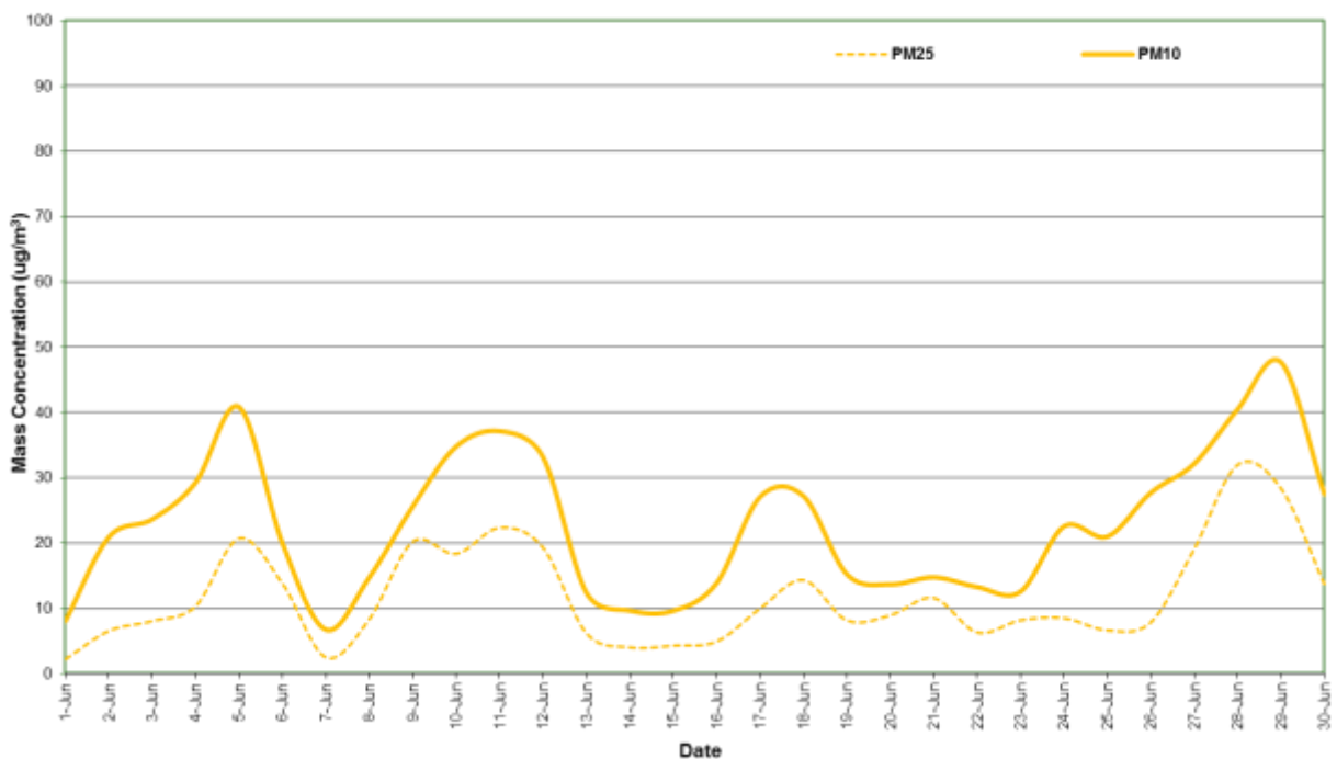
Figure 3: Station 2 PM 2.5 and PM 10 concentration (24 Hour Average) – June 2020
