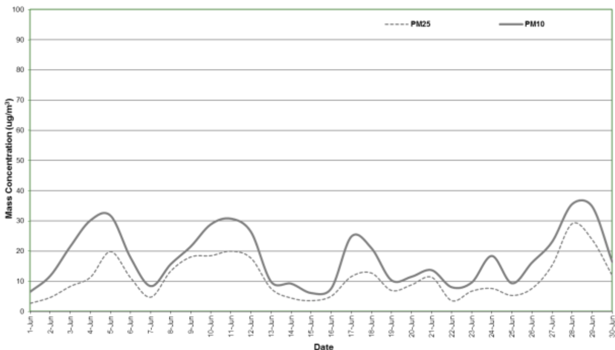
Figure 4: Station 3 PM 2.5 and PM 10 concentration (24 hour average) – June 2020
