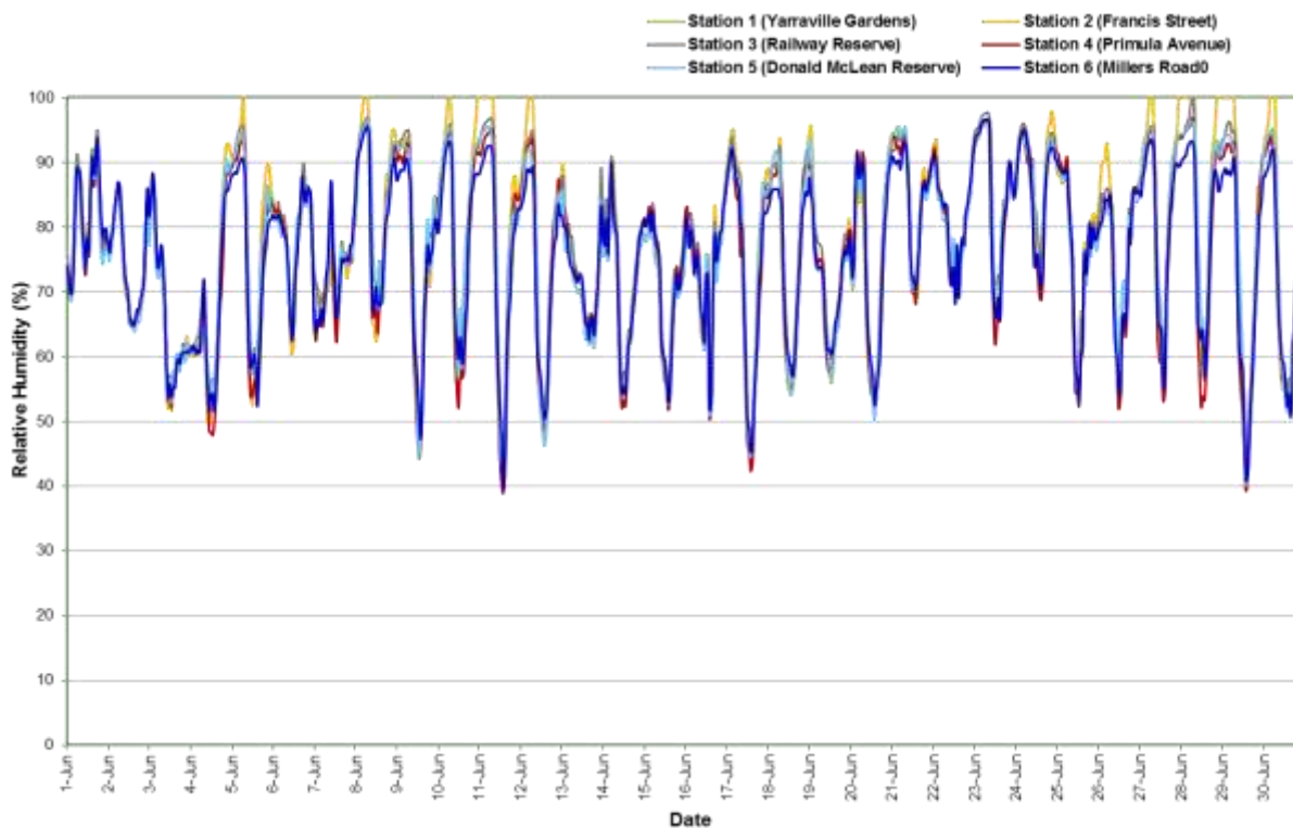
Figure 13: Relative humidity (1 hour average) All AAQMs – June 2020
