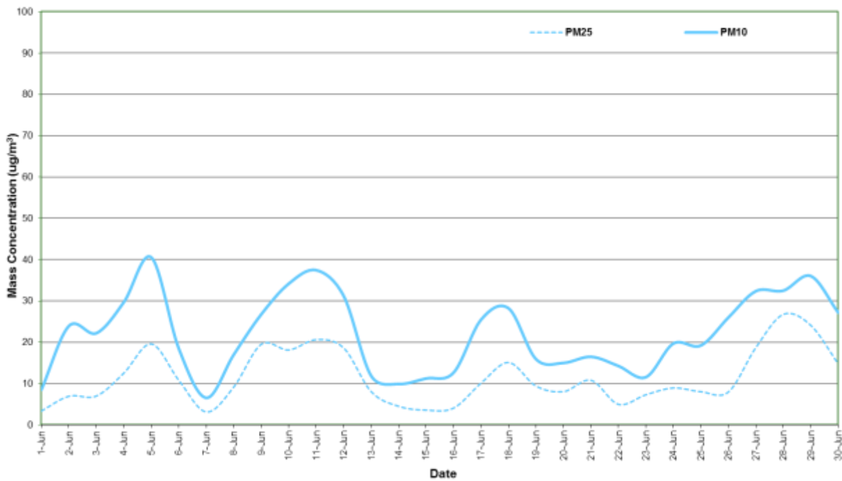
Figure 6: Station 5 PM 2.5 and PM 10 concentration (24 hour average) – June 2020
