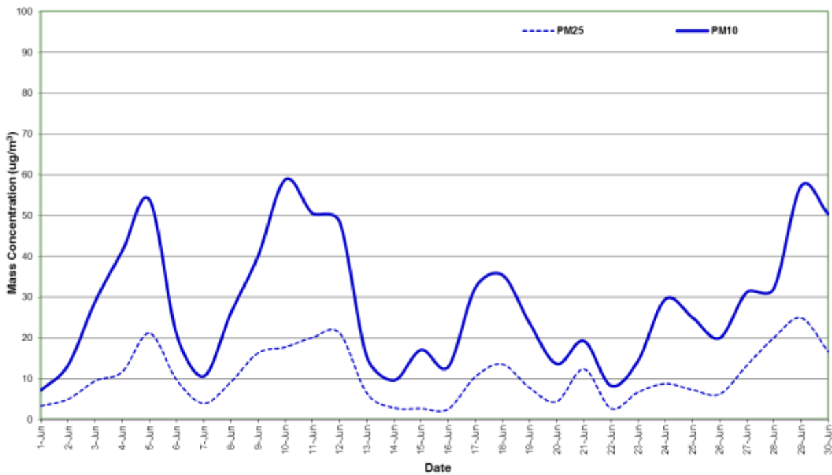
Figure 7: Station 6 PM 2.5 and PM 10 concentration (24 hour average) – June 2020
