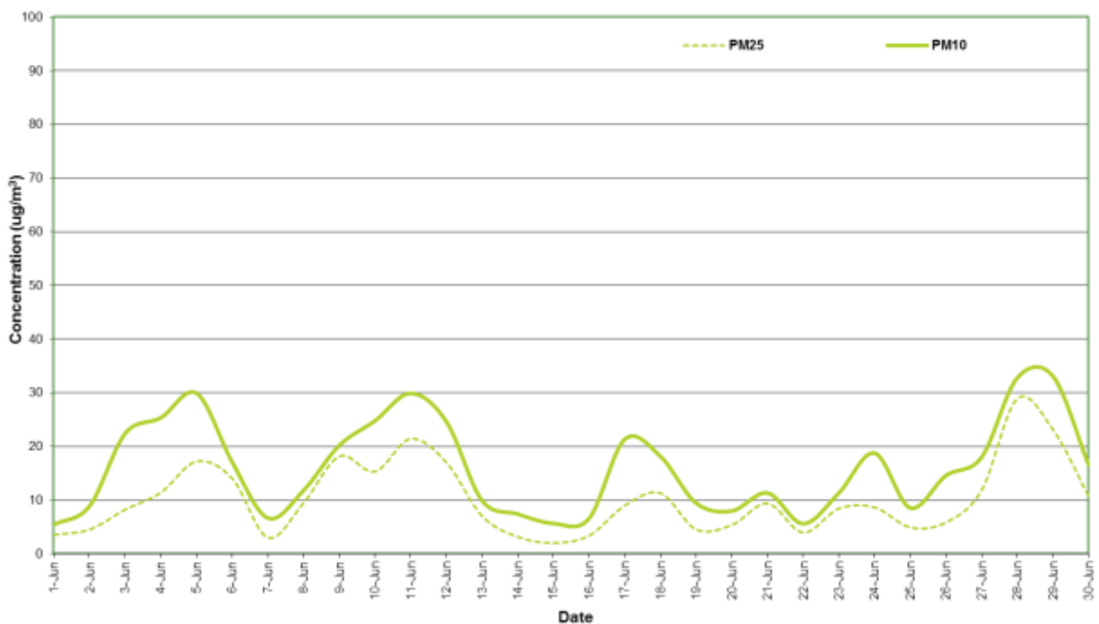
Figure 2: Station 1 PM 2.5 and PM 10 concentration (24 hour average) – June 2020
