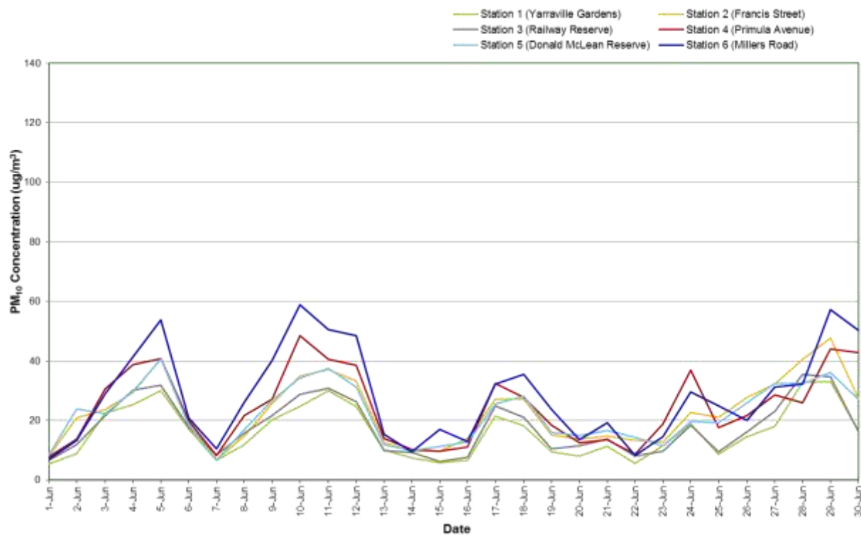
Figure 9: Combined PM 10 concentration (24 hour average) – June 2020
