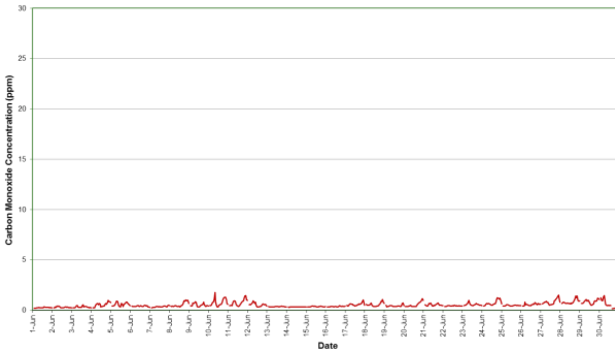
Figure 11: Station 4 CO concentration (1 hour average) – June 2020
