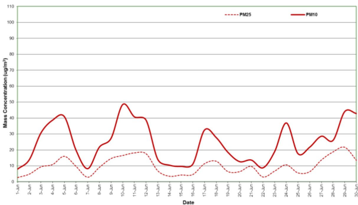
Figure 5: Station 4 PM 2.5 and PM 10 concentration (24 hour average) – June 2020
