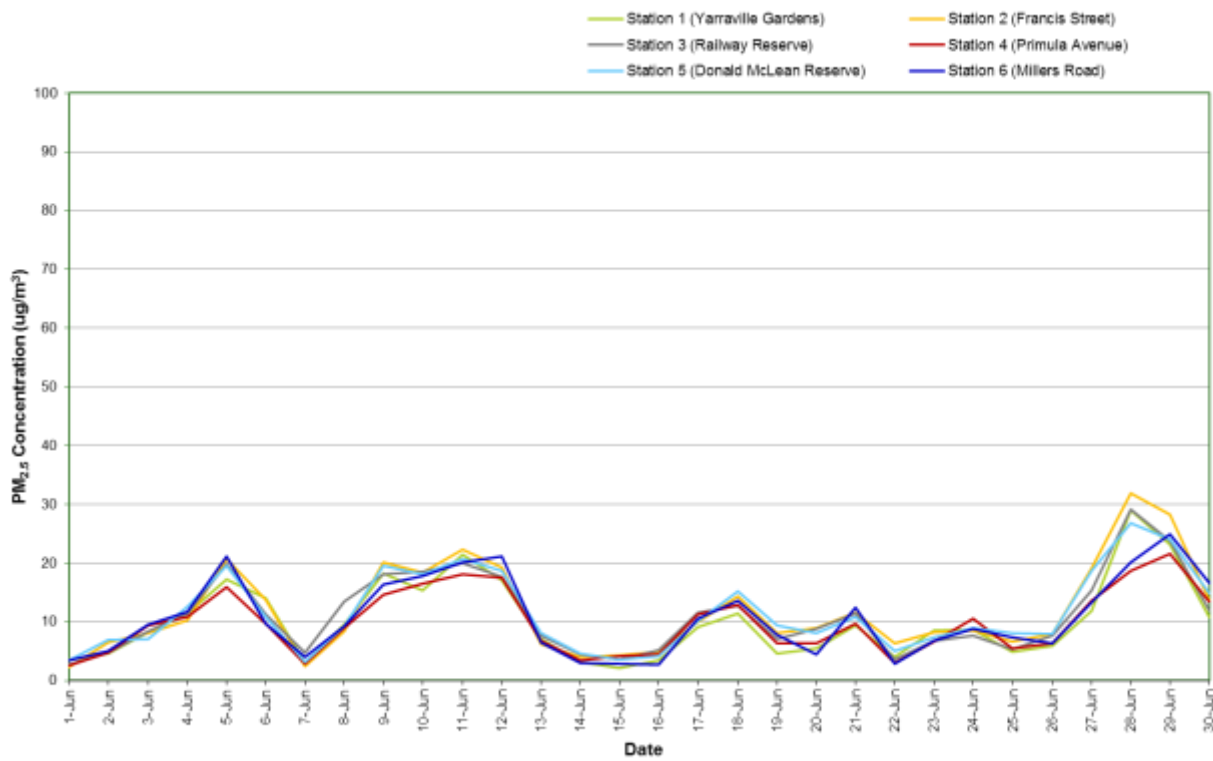
Figure 8: Combined PM 2.5 concentration (24 hour average) – June 2020
