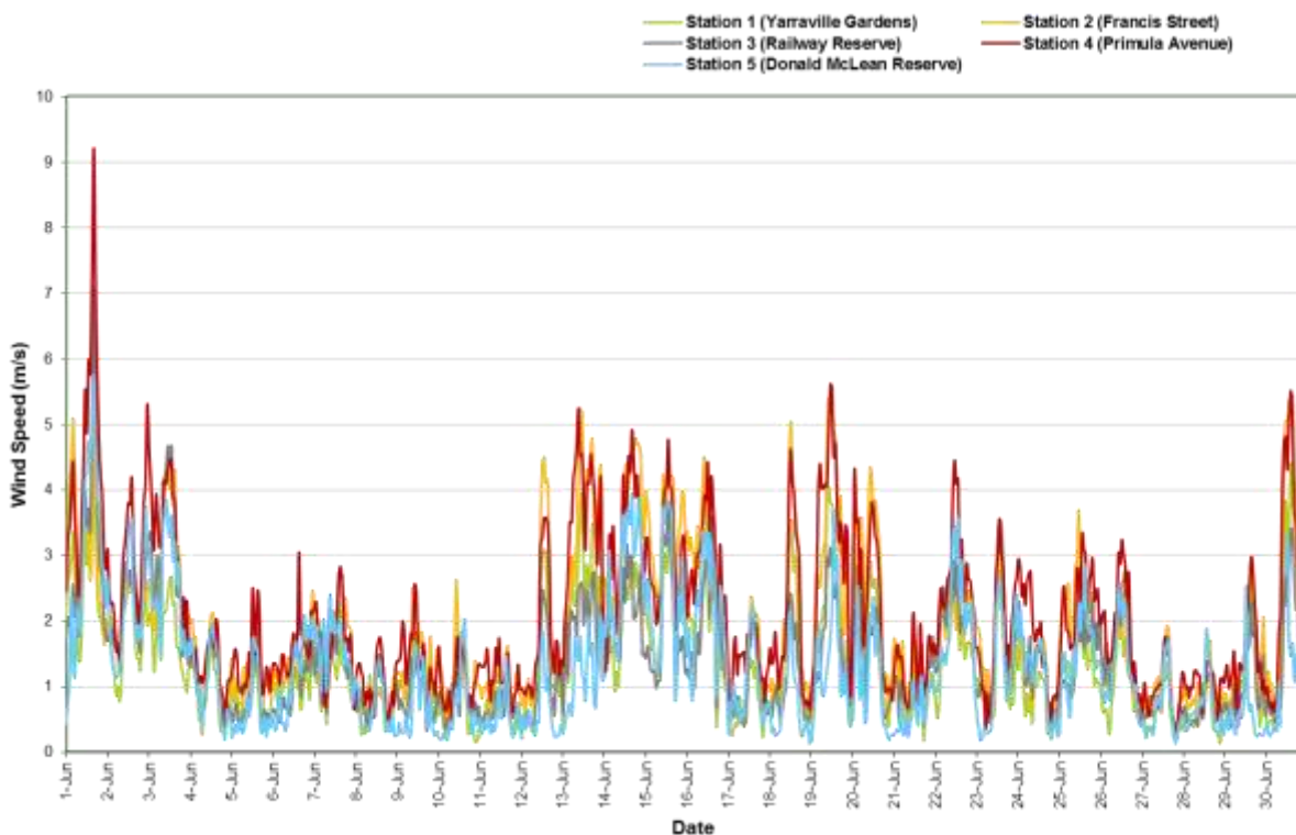
Figure 15: Wind speed (1 hour average) All AAQMs – June 2020
