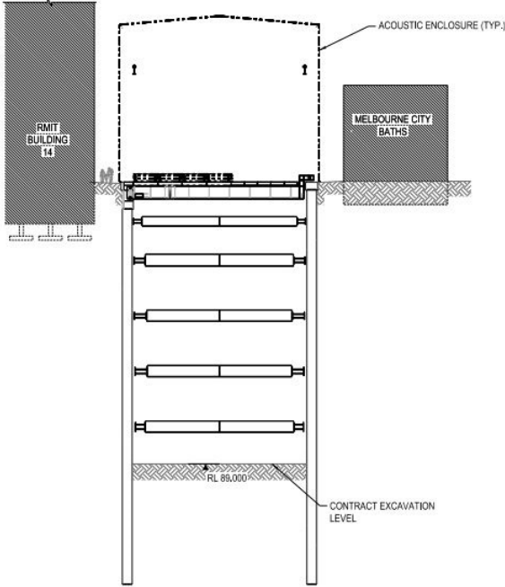
CROSS SECTION ON GRID LINE CNN+5m LOOKING WEST
