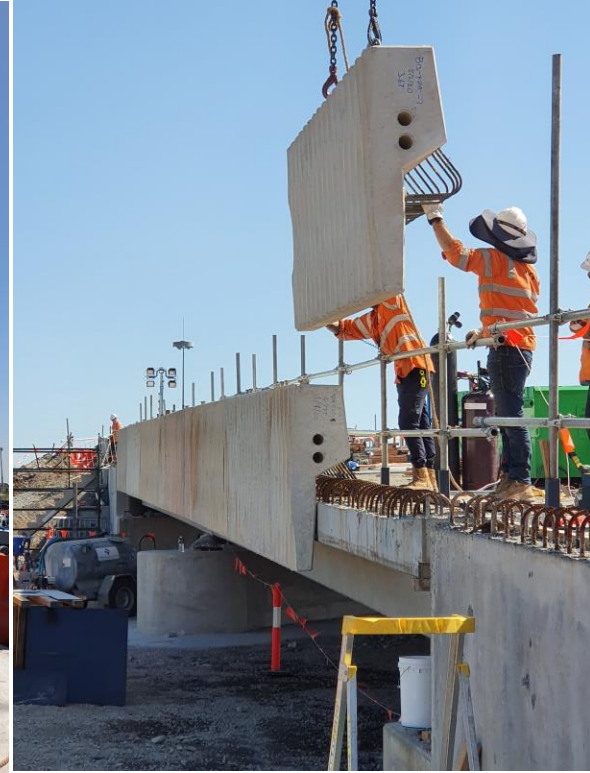
Deck barrier installation
