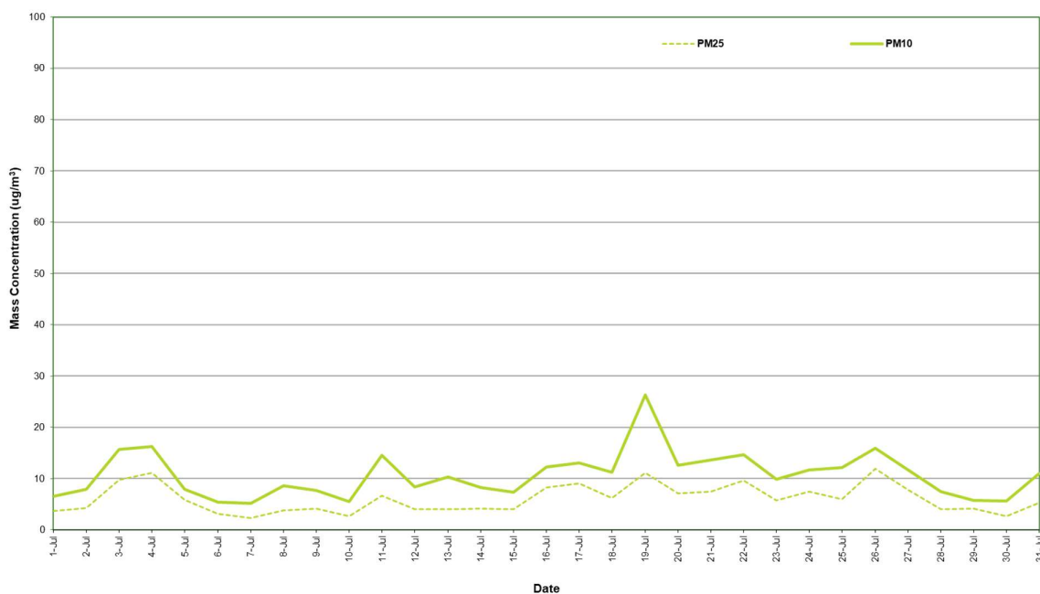
Figure 2: Station 1 PM 2.5 and PM 10 concentration (24 hour average) – July 2023
