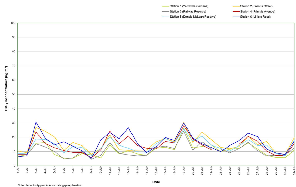
Figure 9: Combined PM 10 concentration (24 hour average) – July 2023
