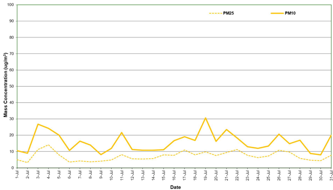
Figure 3: Station 2 PM 2.5 and PM 10 concentration (24 Hour Average) – July 2023
