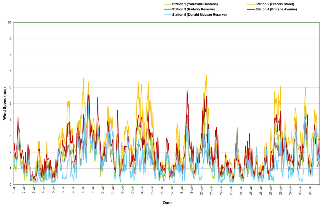
Figure 15: Wind speed (1 hour average) All AAQMs – July 2023
