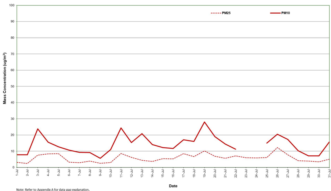
Figure 5: Station 4 PM 2.5 and PM 10 concentration (24 hour average) – July 2023
