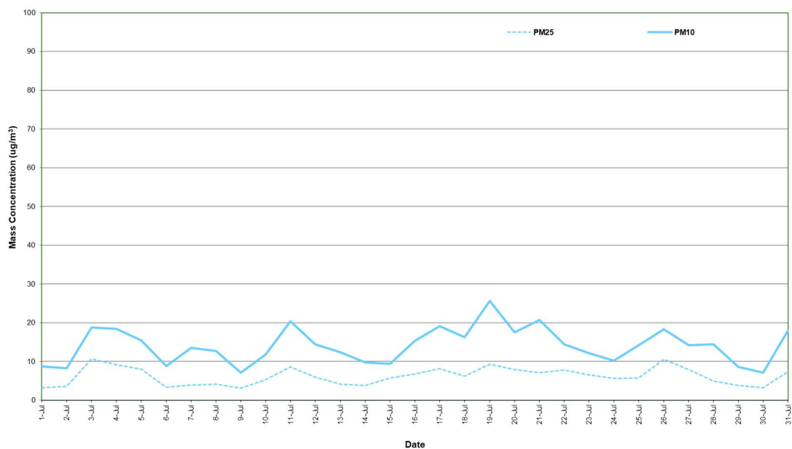
Figure 6: Station 5 PM 2.5 and PM 10 concentration (24 hour average) – July 2023
