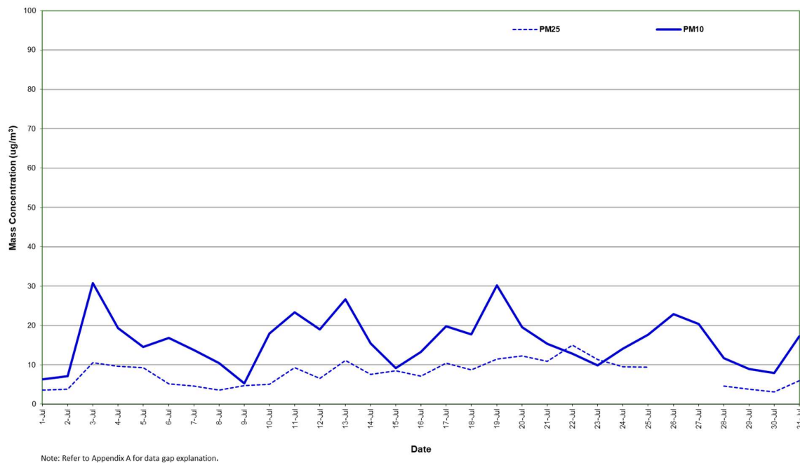
Figure 7: Station 6 PM 2.5 and PM 10 concentration (24 hour average) – July 2023
