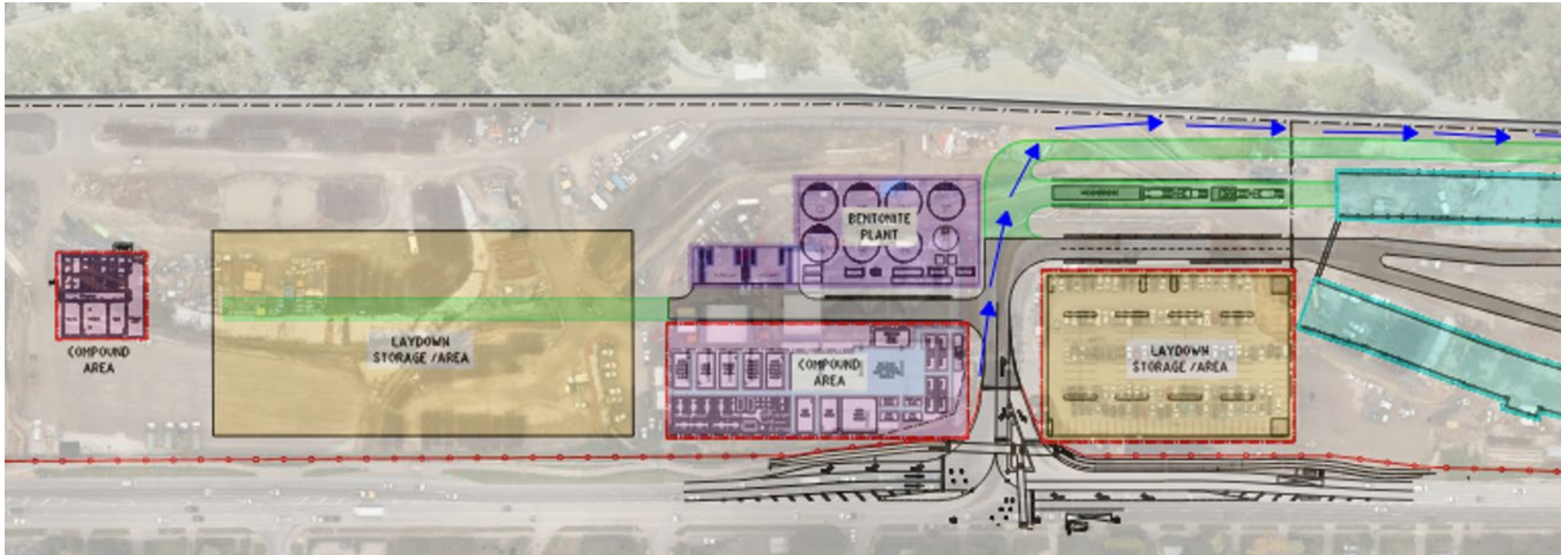
Overall Indicative Site Layout – Inset 1
