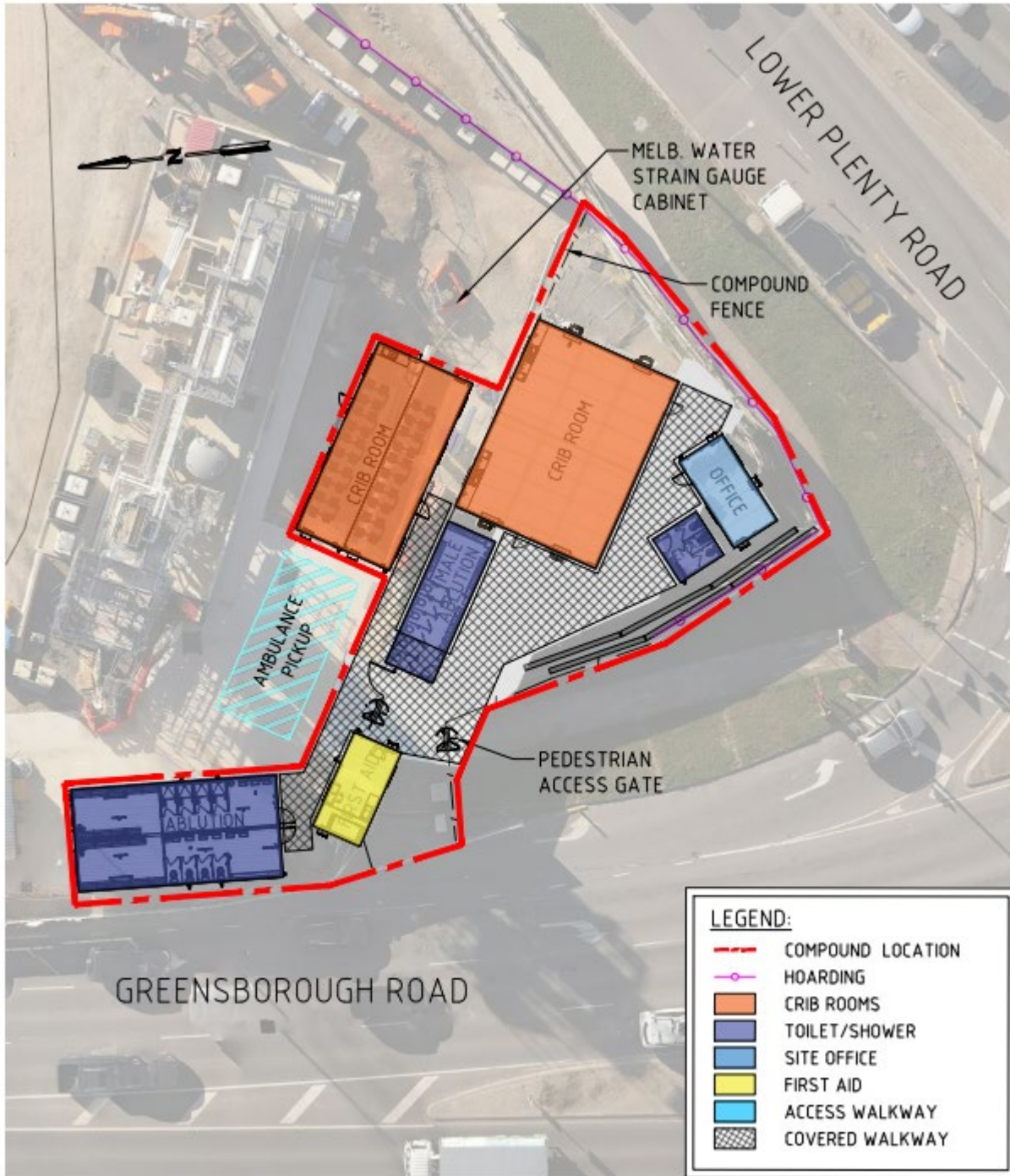
Figure 4 Lower Plenty Structures Southern Mini-Compound
