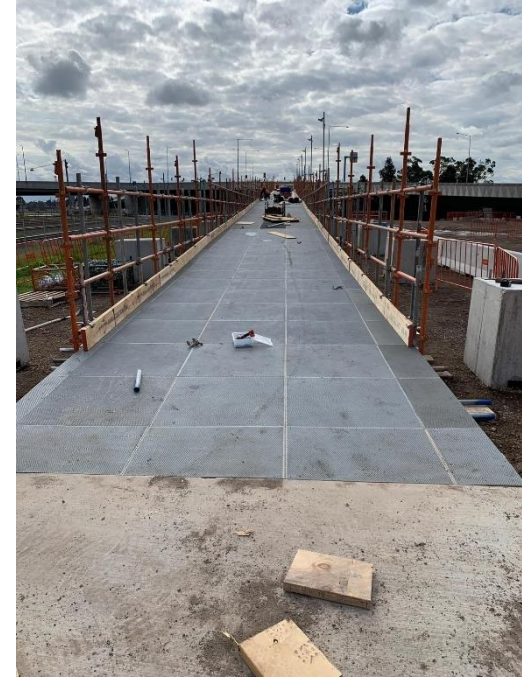
Footscray Road SUP diversion scaffolding (under construction)
