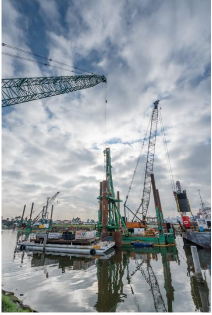
Piling barges
