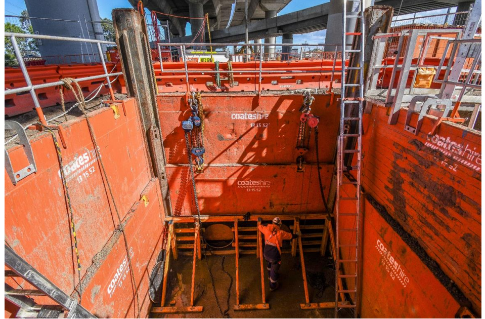
Shaft for pipe-jacking TBM to relocate 66KV power lines
