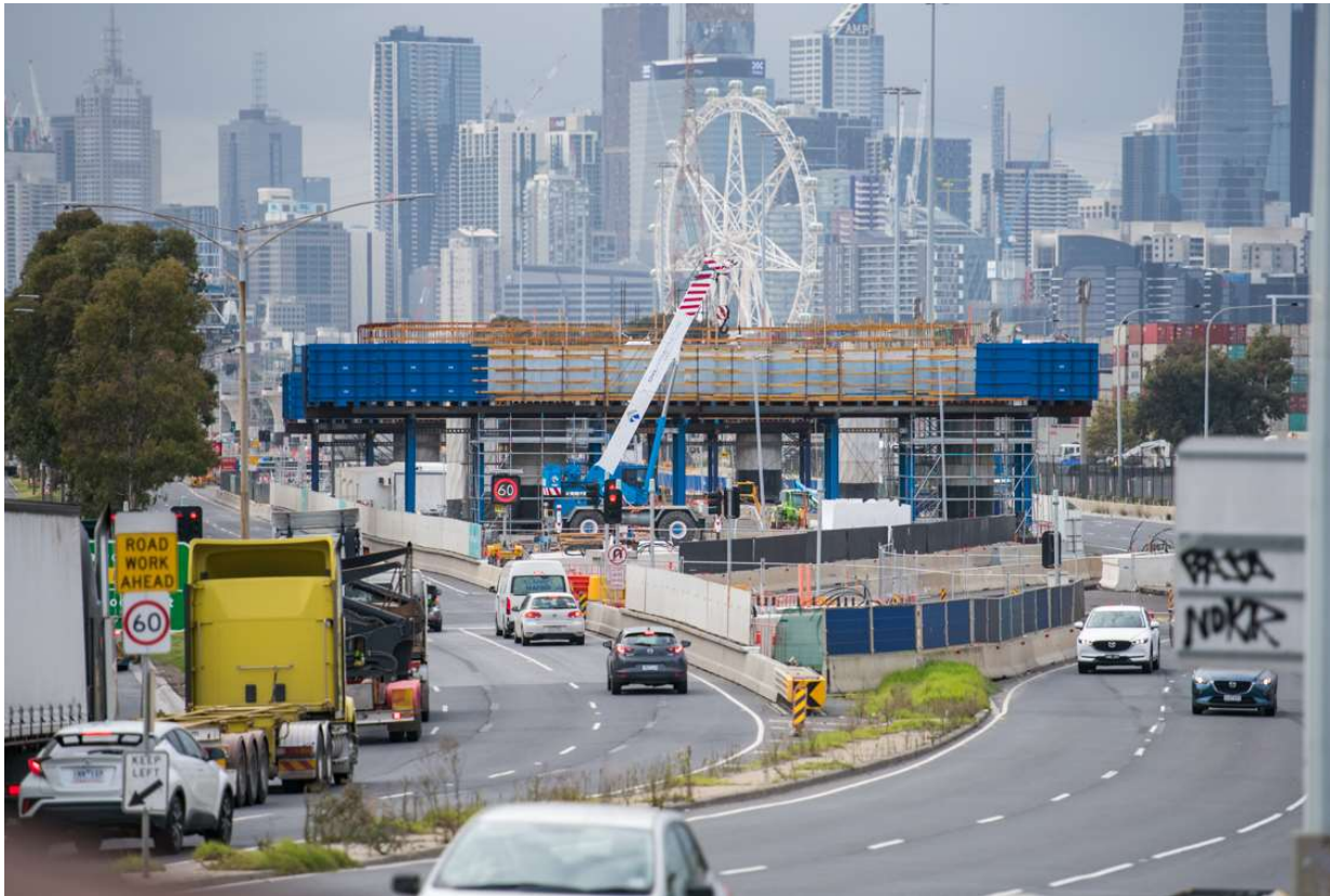
Concrete and steel installation on Footscray Road to support the future elevated roadway
