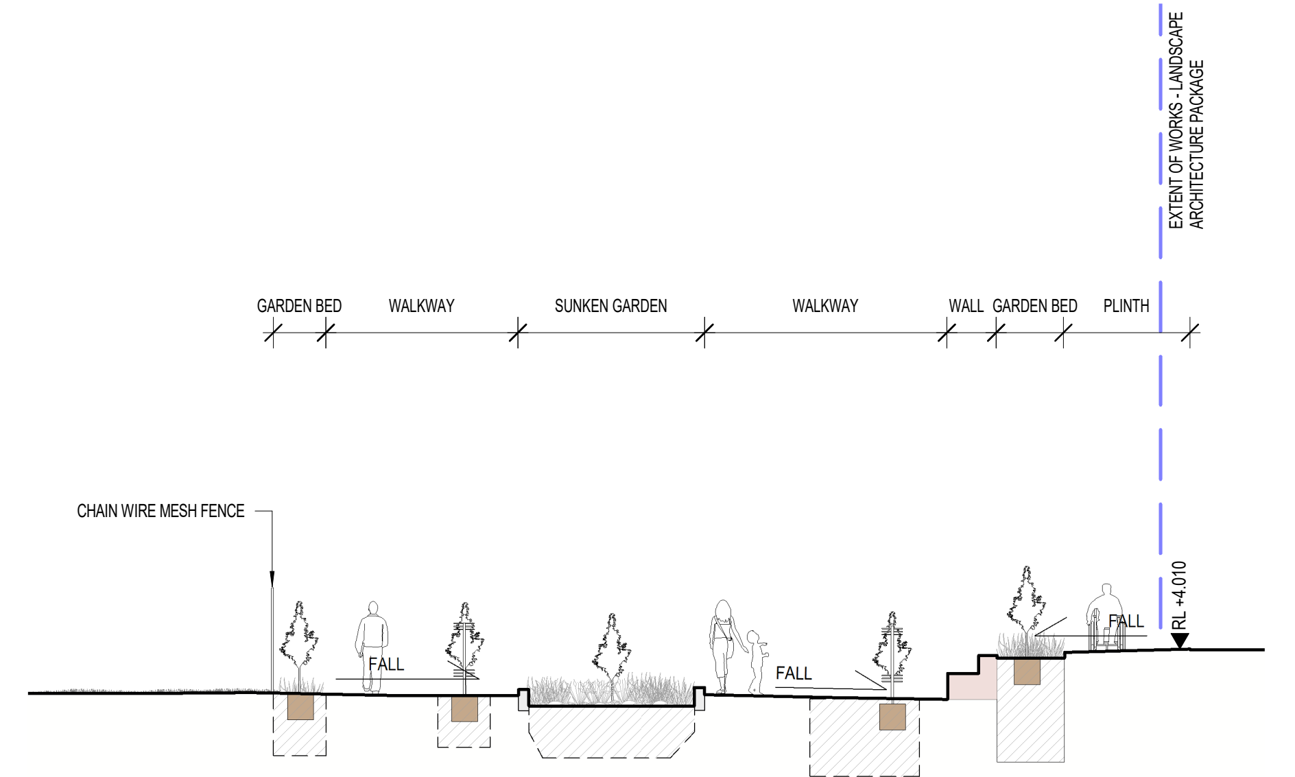
4 SECTION A - LAURENS LANE 1:100
