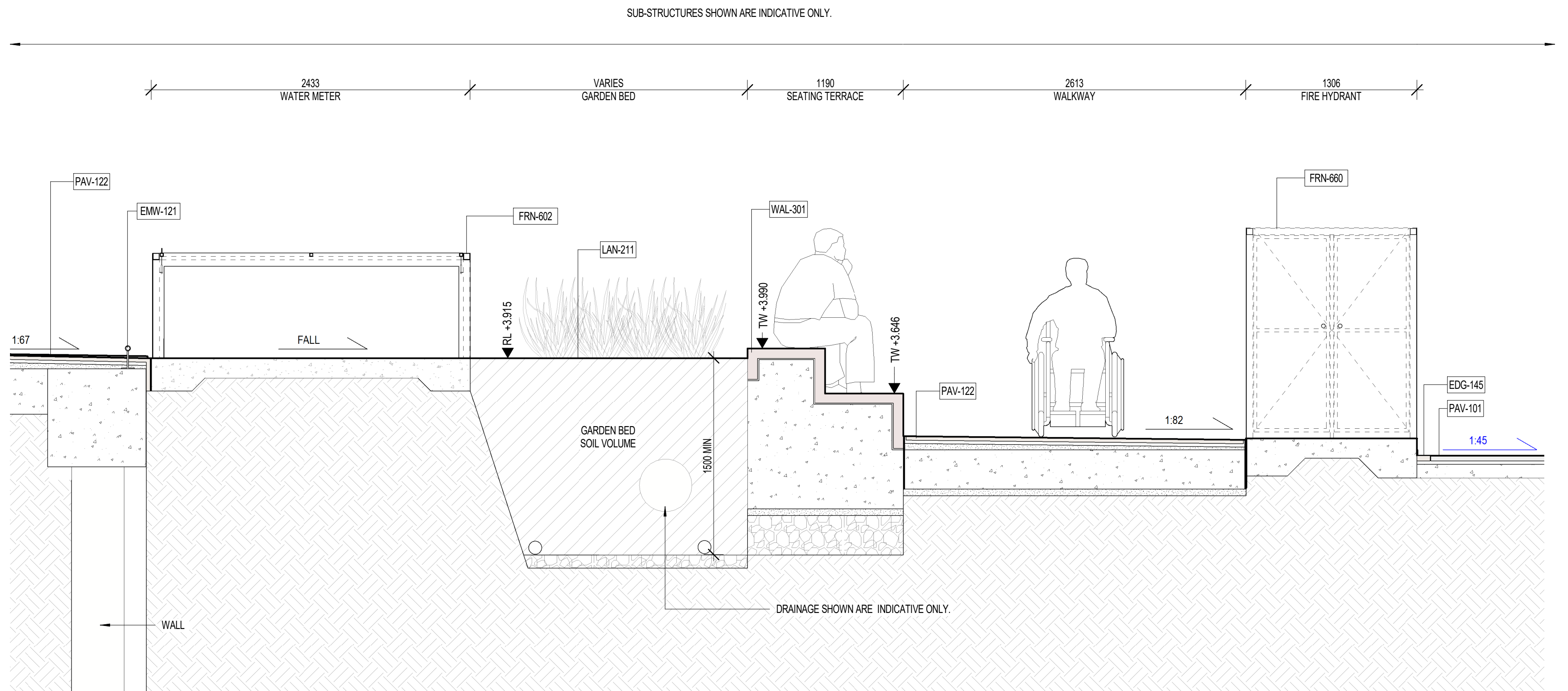
2 SECTION - LAURENS STREET - WATER AND FIRE CABINET 1:25
