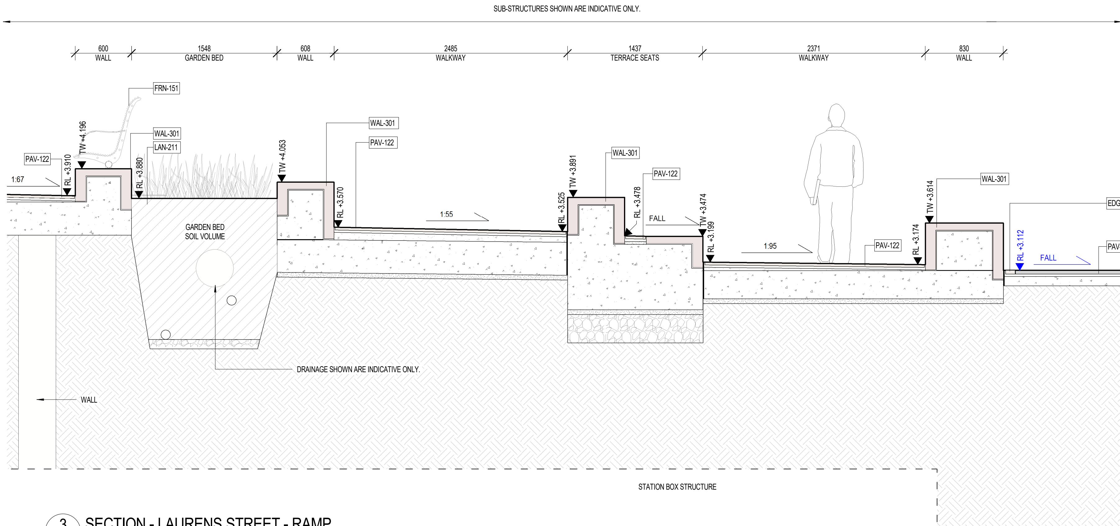
3 SECTION - LAURENS STREET - RAMP 1:25
