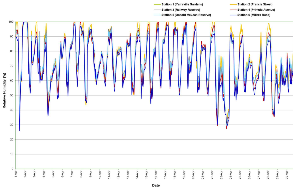
Figure 13: Relative humidity (1 hour average) All AAQMs – April 2024
