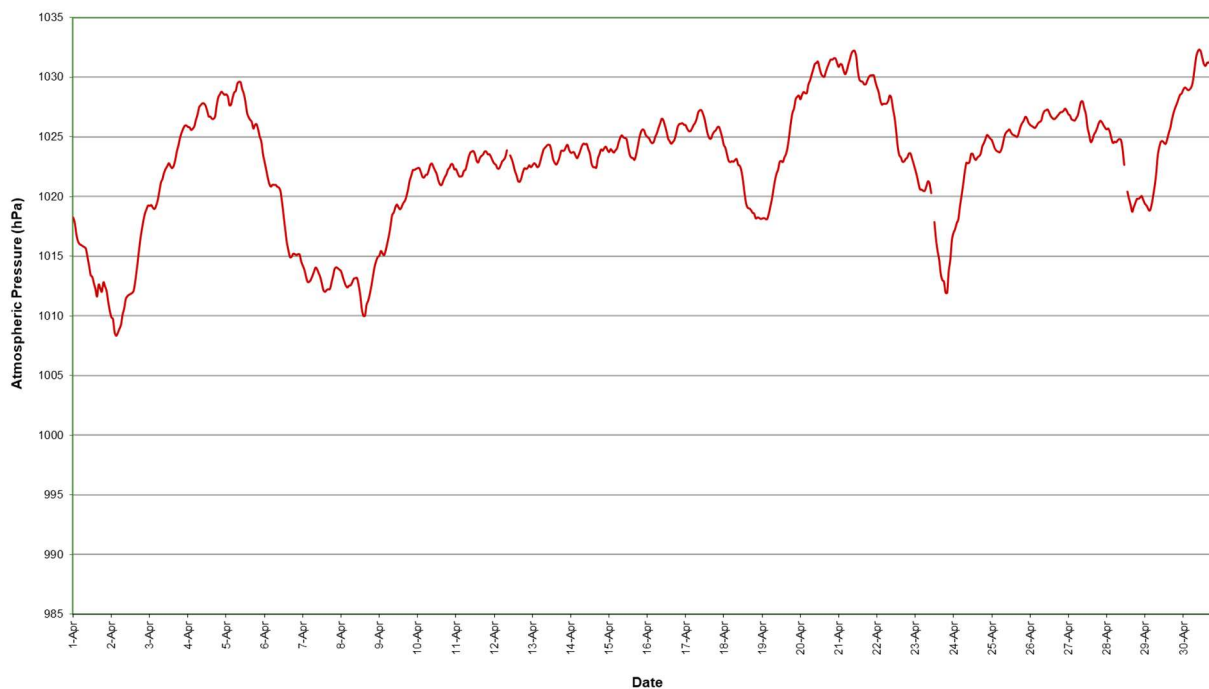
Figure 14: Atmospheric pressure (1 hour average) Station 4 Primula Avenue – April 2024
