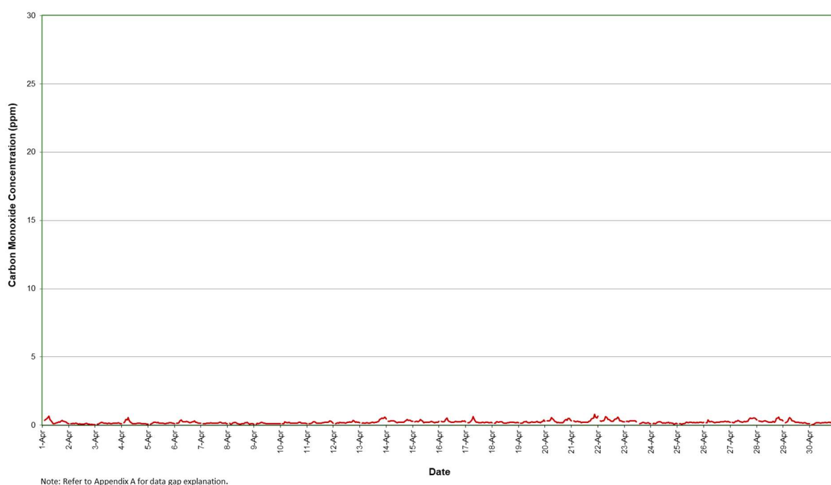
Figure 11: Station 4 CO concentration (1 hour average) – April 2024
