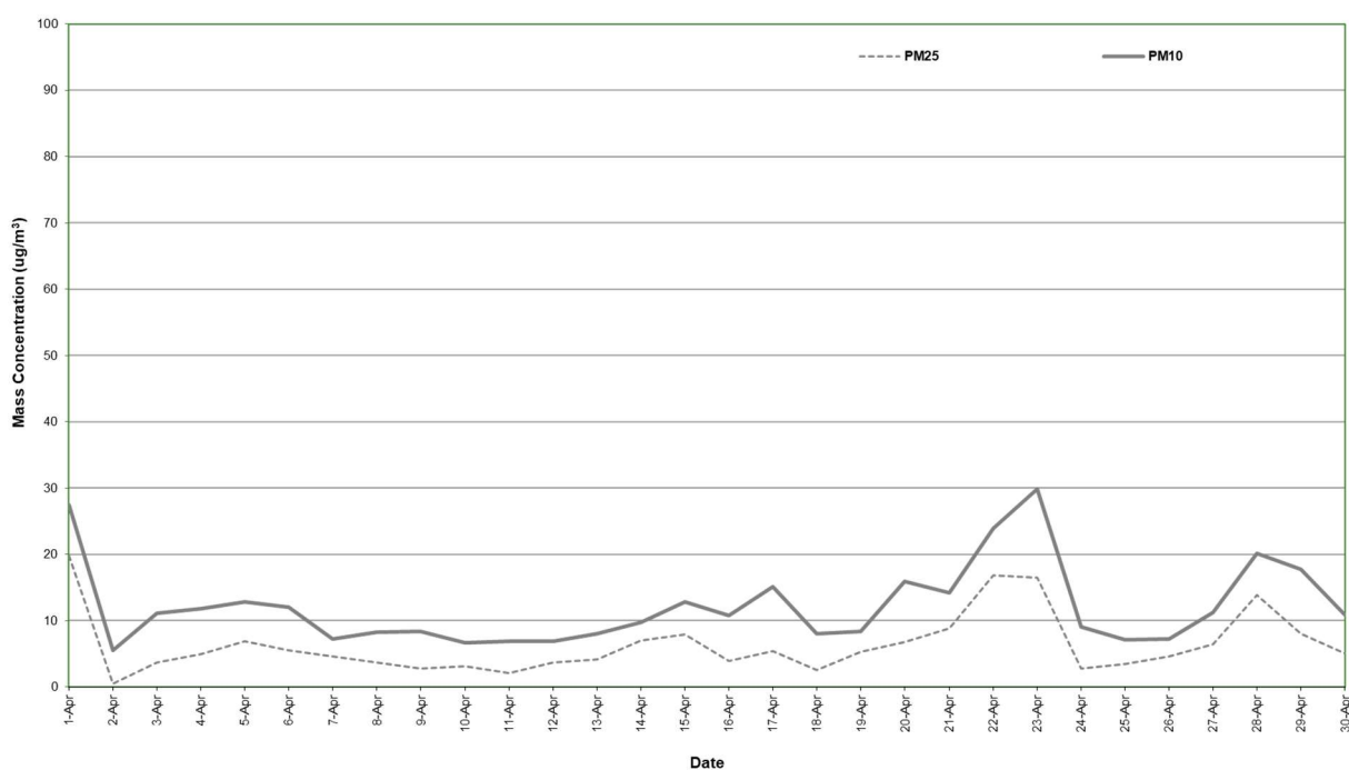
Figure 4: Station 3 PM 2.5 and PM 10 concentration (24 hour average) – April 2024
