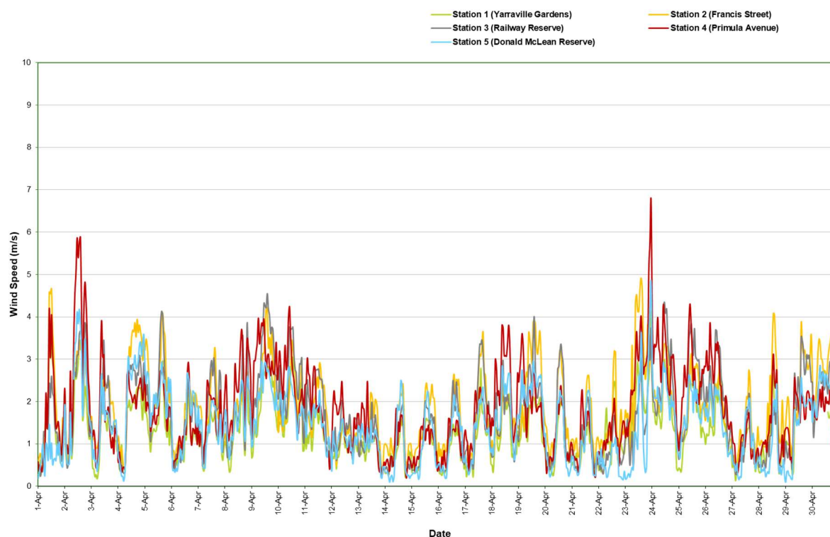
Figure 15: Wind speed (1 hour average) All AAQMs – April 2024
