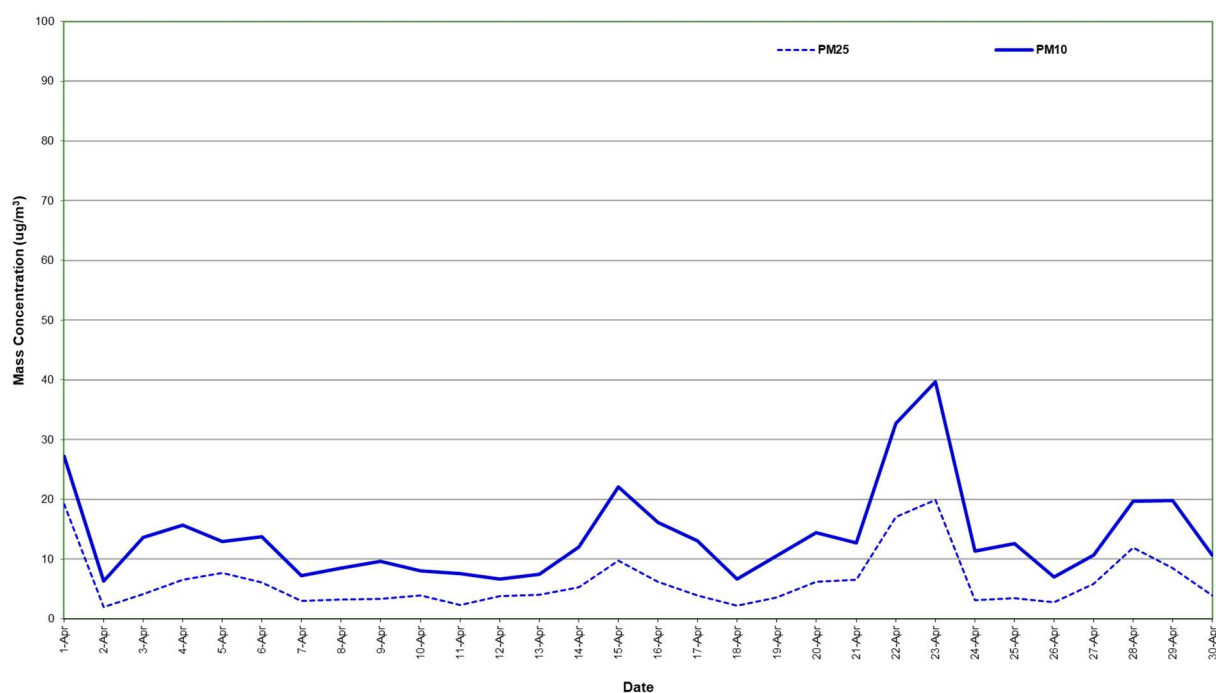
Figure 7: Station 6 PM 2.5 and PM 10 concentration (24 hour average) – April 2024
