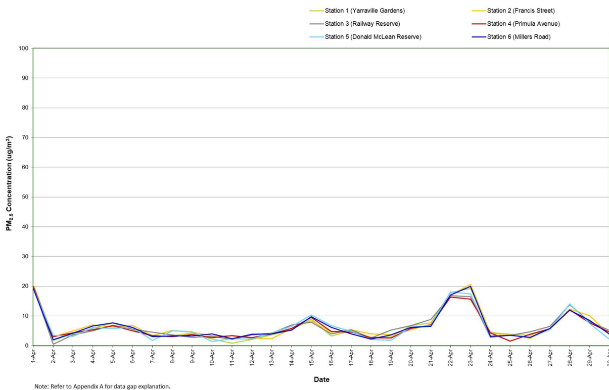
Figure 8: Combined PM 2.5 concentration (24 hour average) – April 2024
