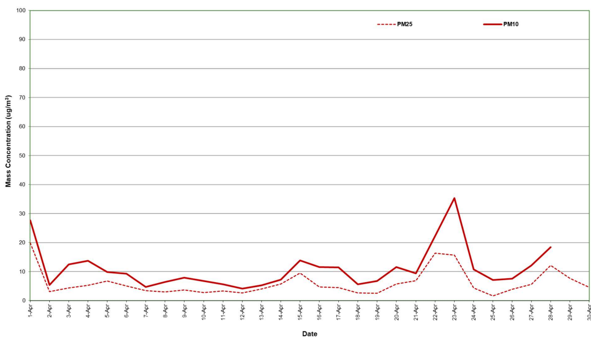
Figure 5: Station 4 PM 2.5 and PM 10 concentration (24 hour average) – April 2024
