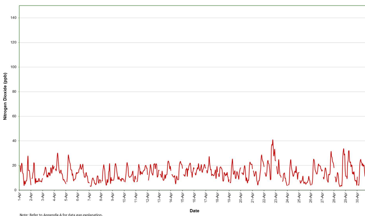
Figure 10: Station 4 NO 2 concentration (1 hour average) – April 2024
