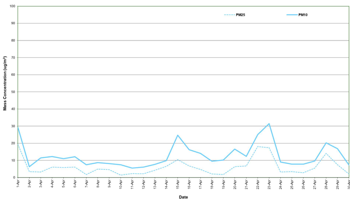
Figure 6: Station 5 PM 2.5 and PM 10 concentration (24 hour average) – April 2024
