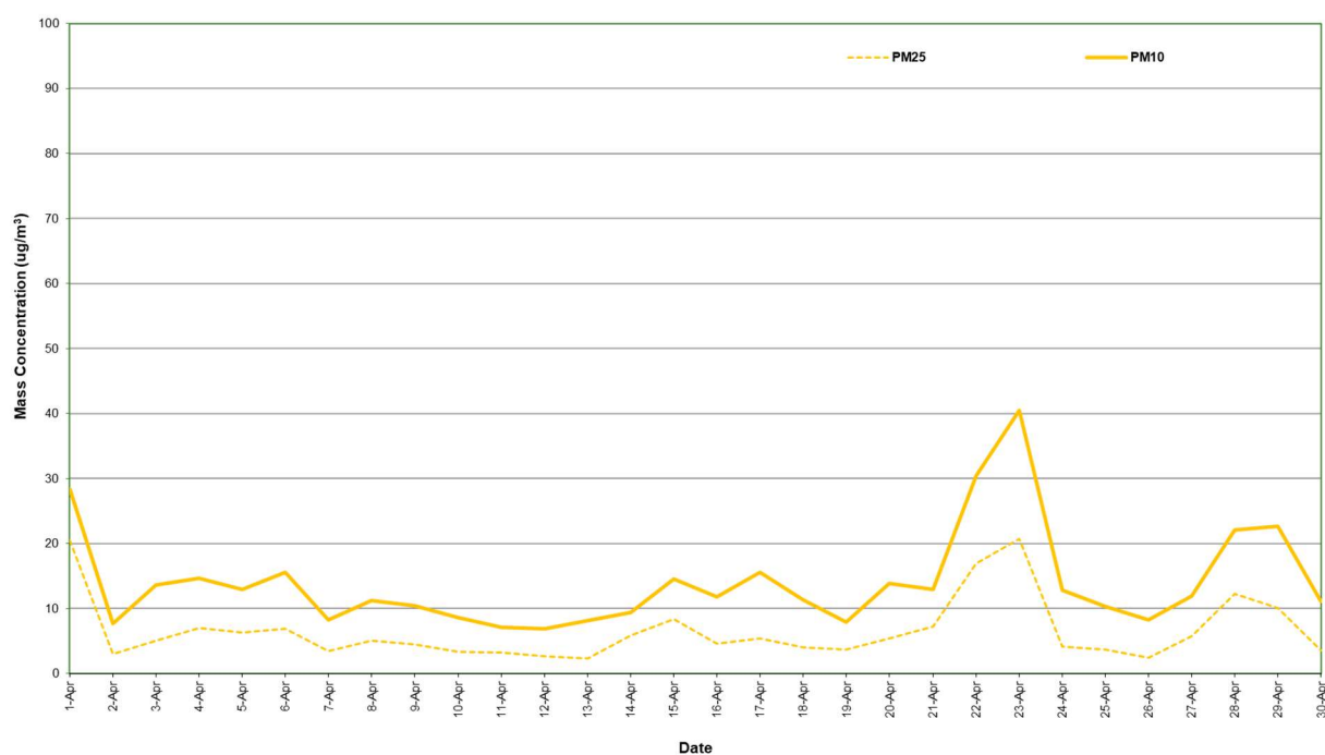
Figure 3: Station 2 PM 2.5 and PM 10 concentration (24 Hour Average) – April 2024
