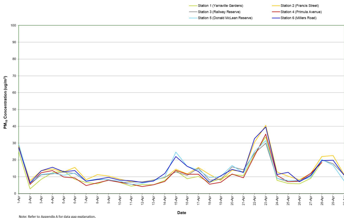
Figure 9: Combined PM 10 concentration (24 hour average) – April 2024
