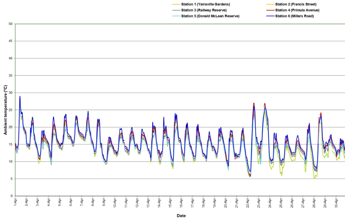
Figure 12: Ambient temperature (1 hour average) All AAQMS – April 2024
