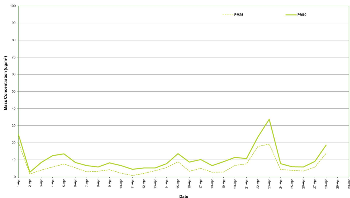
Figure 2: Station 1 PM 2.5 and PM 10 concentration (24 hour average) – April 2024
