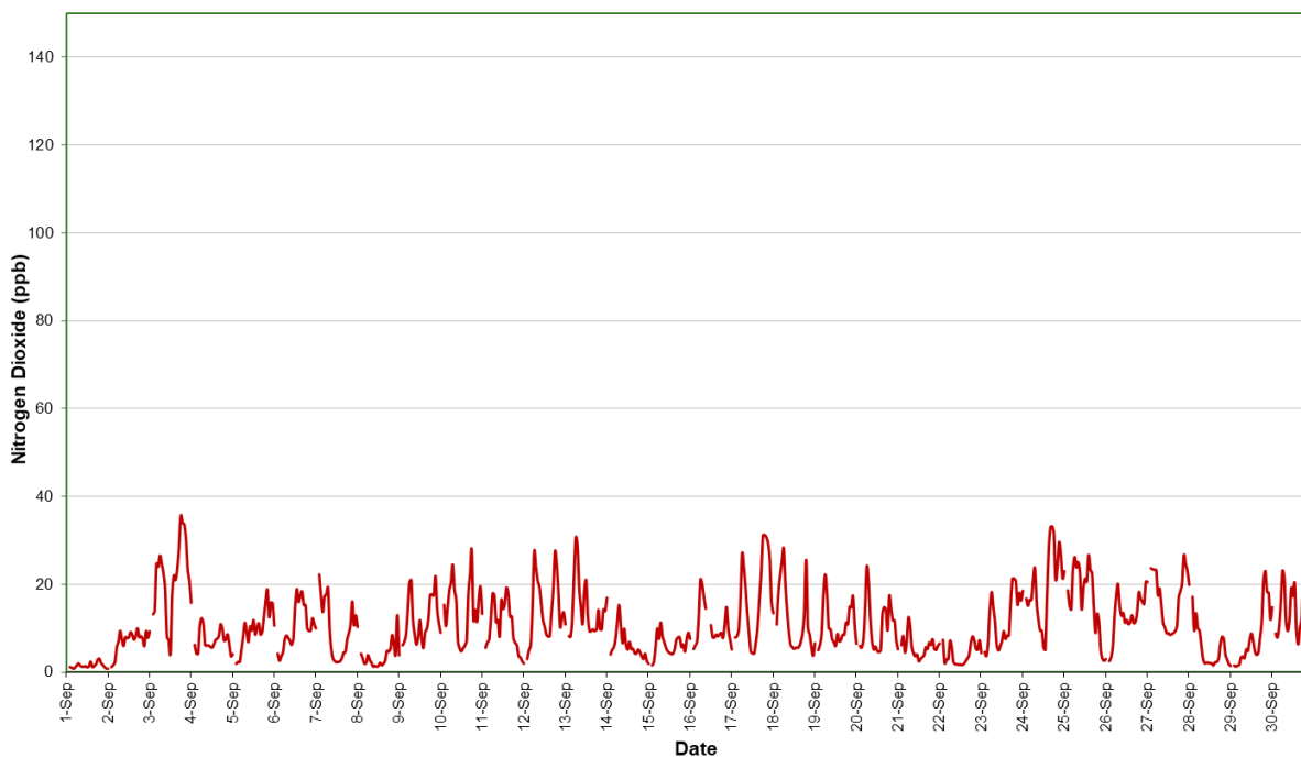
Figure 10: Station 4 NO 2 concentration (1 hour average) – September 2024
