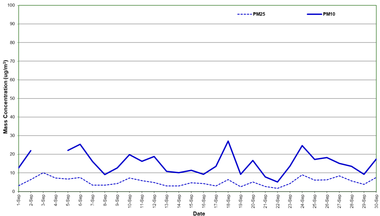
Figure 7: Station 6 PM 2.5 and PM 10 concentration (24 hour average) – September 2024
