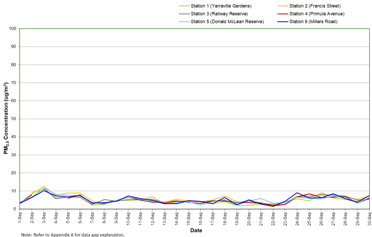
Figure 8: Combined PM 2.5 concentration (24 hour average) – September 2024
