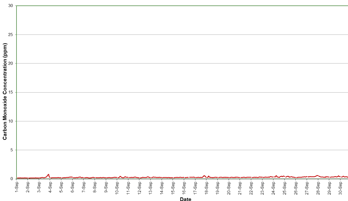
Figure 11: Station 4 CO concentration (1 hour average) – September 2024
