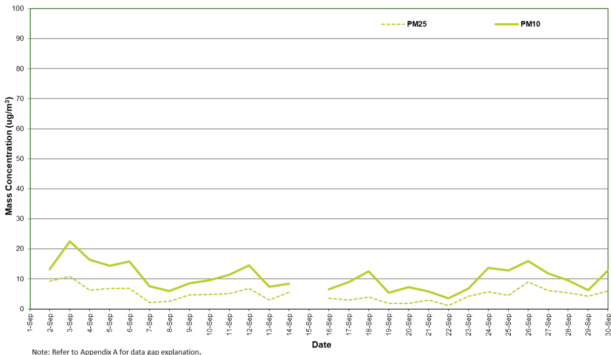
Figure 2: Station 1 PM 2.5 and PM 10 concentration (24 hour average) – September 2024
