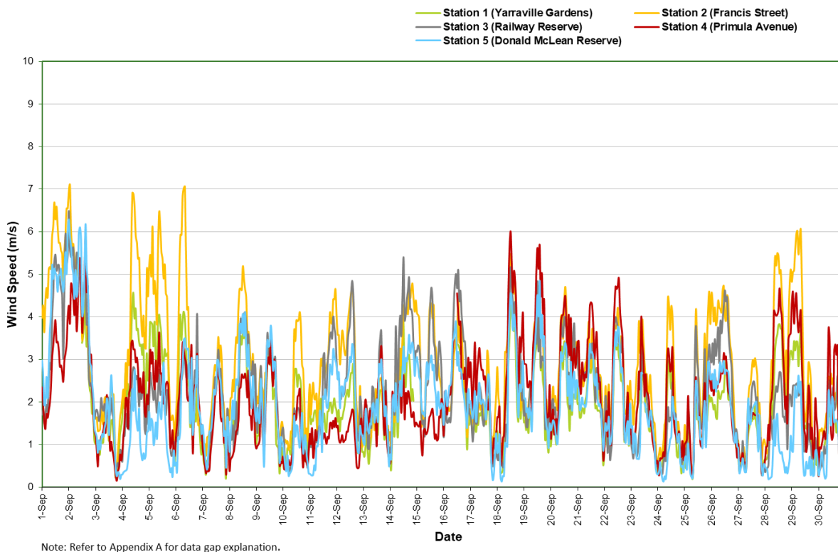
Figure 15: Wind speed (1 hour average) All AAQMs – September 2024
