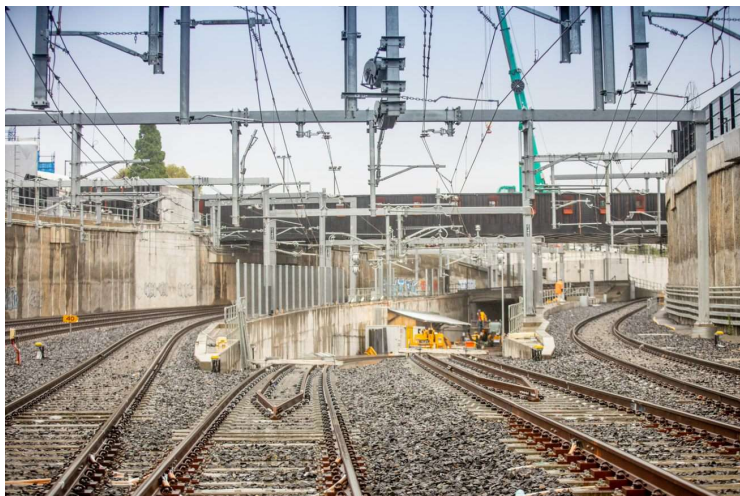
Newly installed rail tracks
