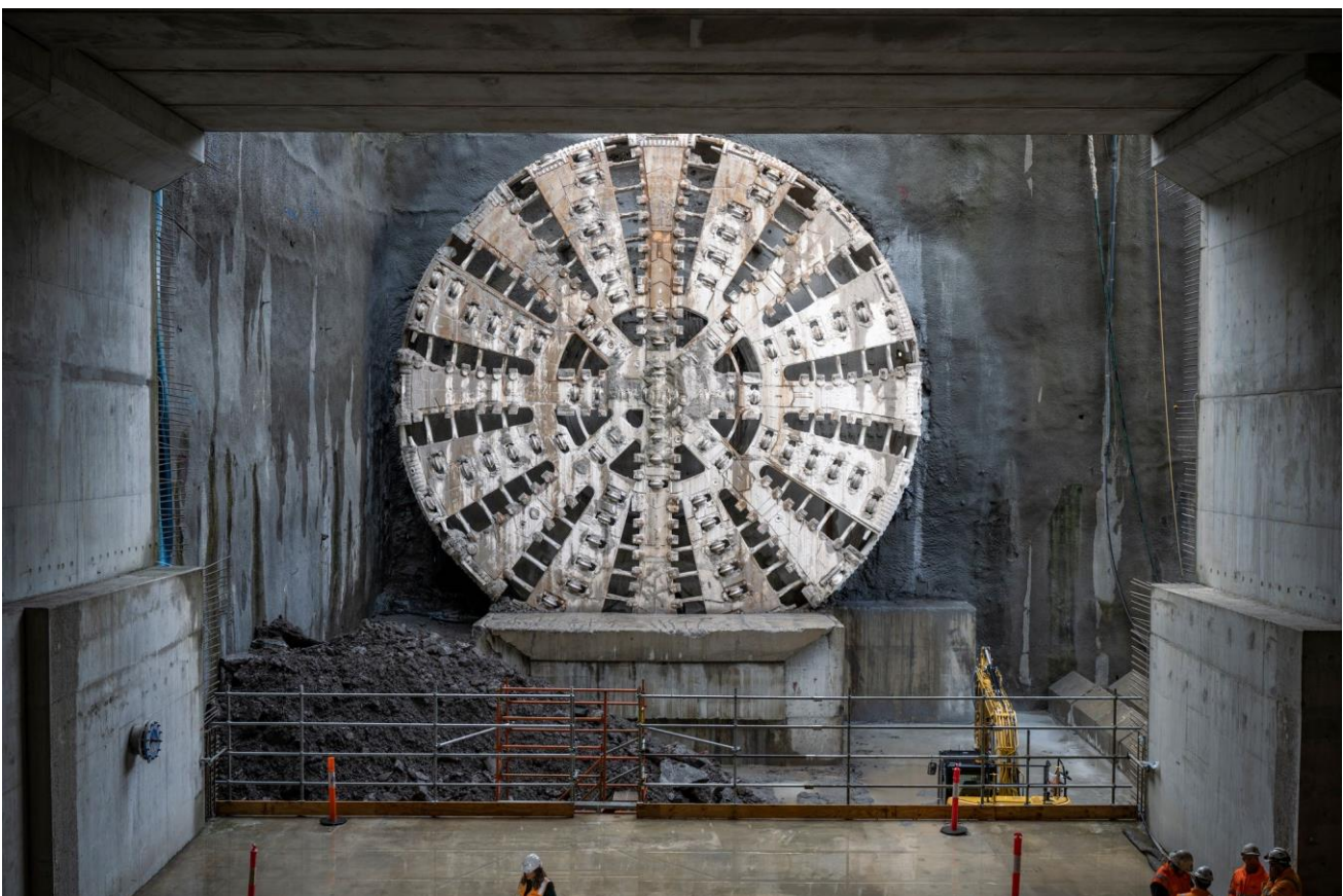
Photo 6 – TBM Bella – Tunnel Zone (Source: WGTP MTIA, 8 May 2023)
