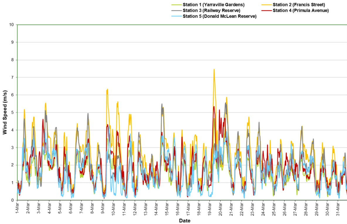
Figure 15: Wind speed (1 hour average) All AAQMs – March 2024
