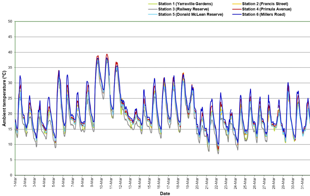
Figure 12: Ambient temperature (1 hour average) All AAQMS – March 2024
