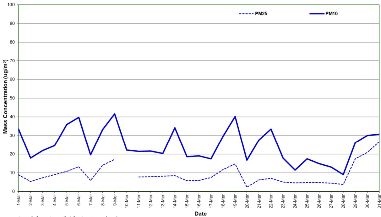
Figure 7: Station 6 PM 2.5 and PM 10 concentration (24 hour average) – March 2024
