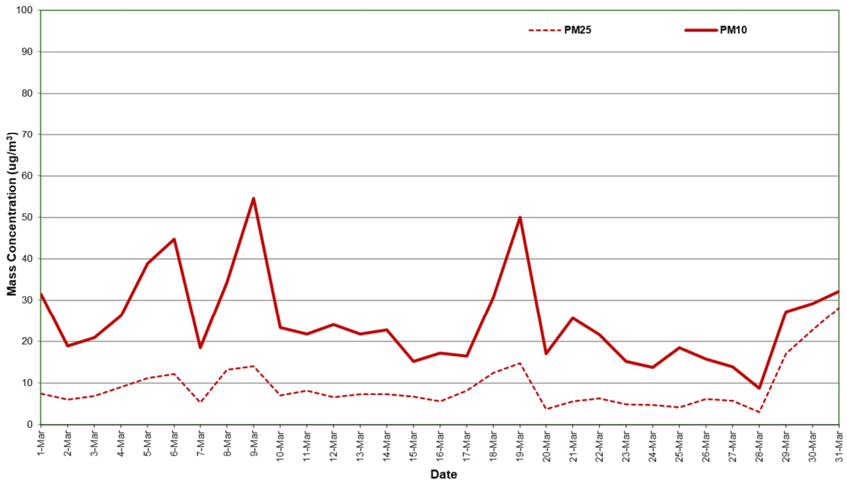
Figure 5: Station 4 PM 2.5 and PM 10 concentration (24 hour average) – March 2024
