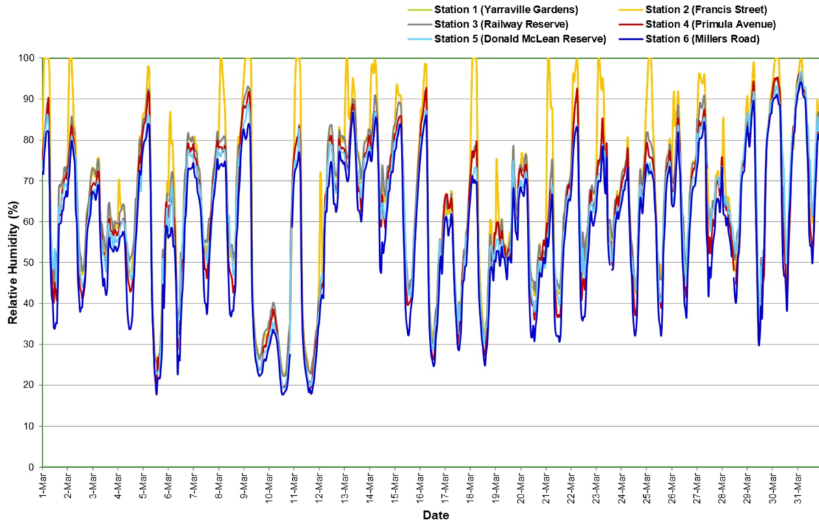
Figure 13: Relative humidity (1 hour average) All AAQMs – March 2024
