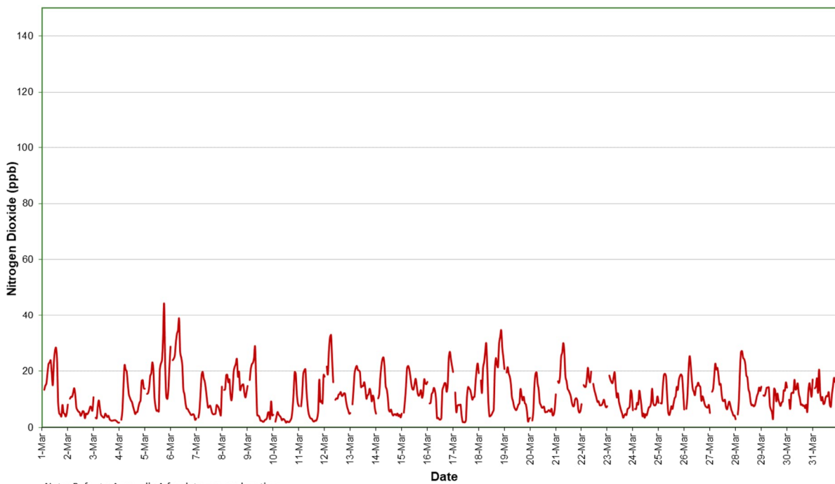
Figure 10: Station 4 NO 2 concentration (1 hour average) – March 2024
