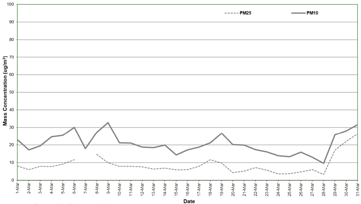
Figure 4: Station 3 PM 2.5 and PM 10 concentration (24 hour average) – March 2024
