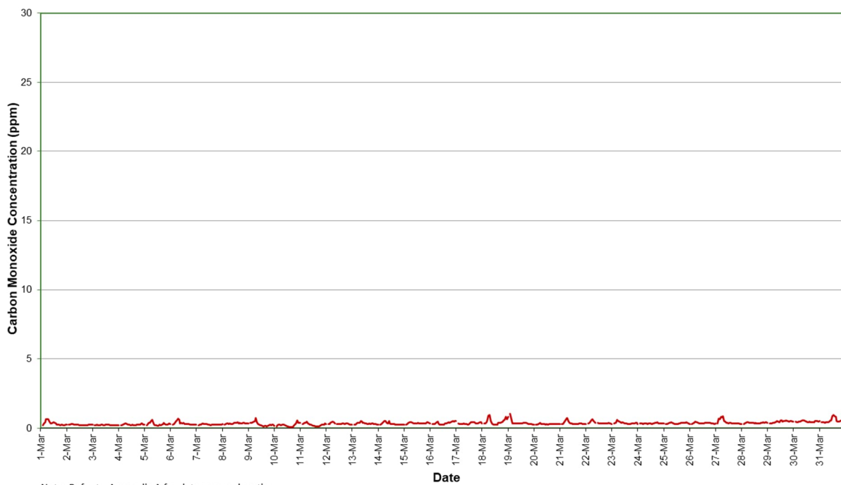
Figure 11: Station 4 CO concentration (1 hour average) – March 2024
