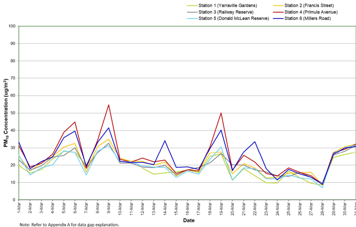
Figure 9: Combined PM 10 concentration (24 hour average) – March 2024
