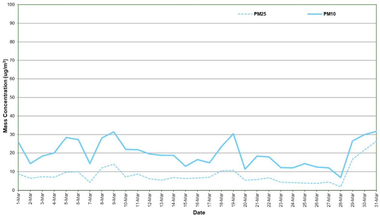
Figure 6: Station 5 PM 2.5 and PM 10 concentration (24 hour average) – March 2024
