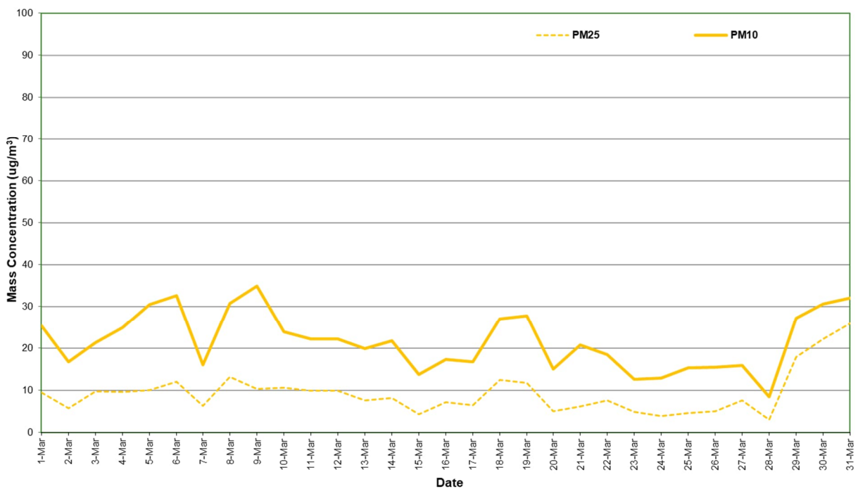
Figure 3: Station 2 PM 2.5 and PM 10 concentration (24 Hour Average) – March 2024
