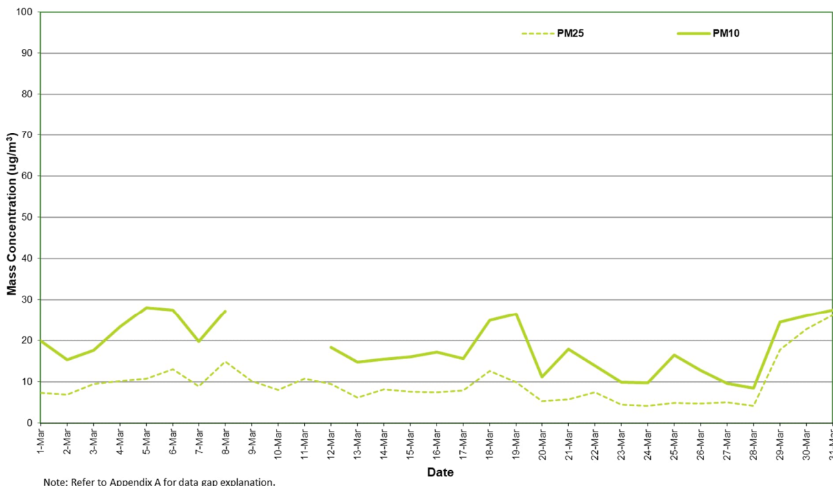
Figure 2: Station 1 PM 2.5 and PM 10 concentration (24 hour average) – March 2024
