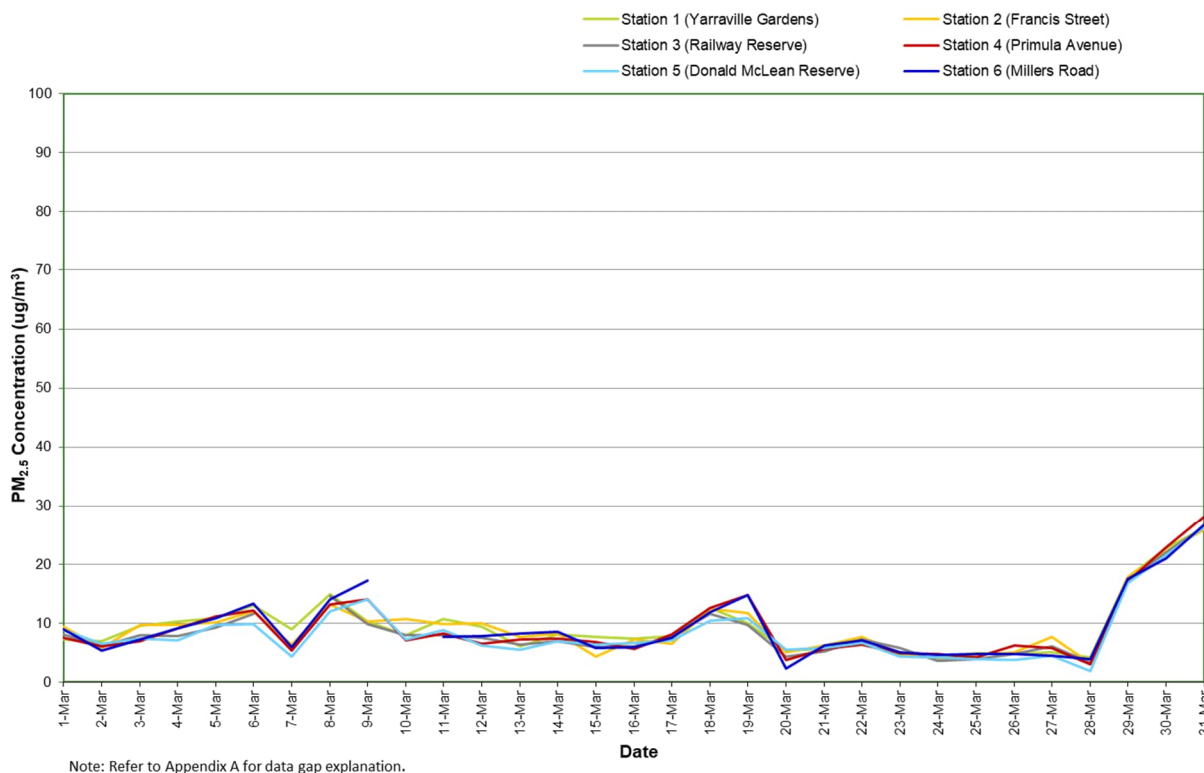
Figure 8: Combined PM 2.5 concentration (24 hour average) – March 2024
