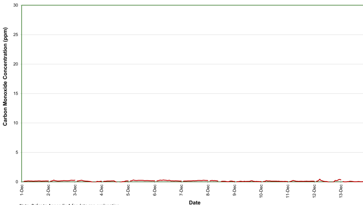
Figure 11: Station 4 CO concentration (1 hour average) – December 2025
