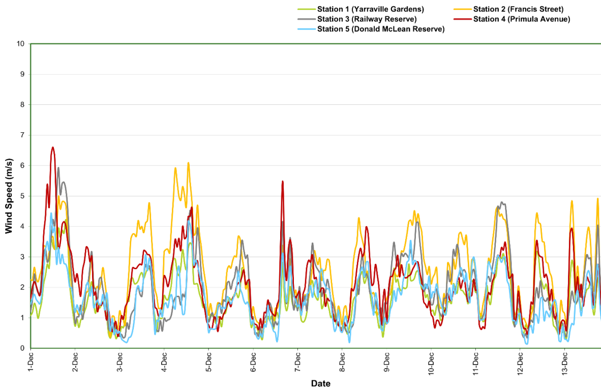
Figure 16: Wind speed (1 hour average) All AAQMs – December 2025
