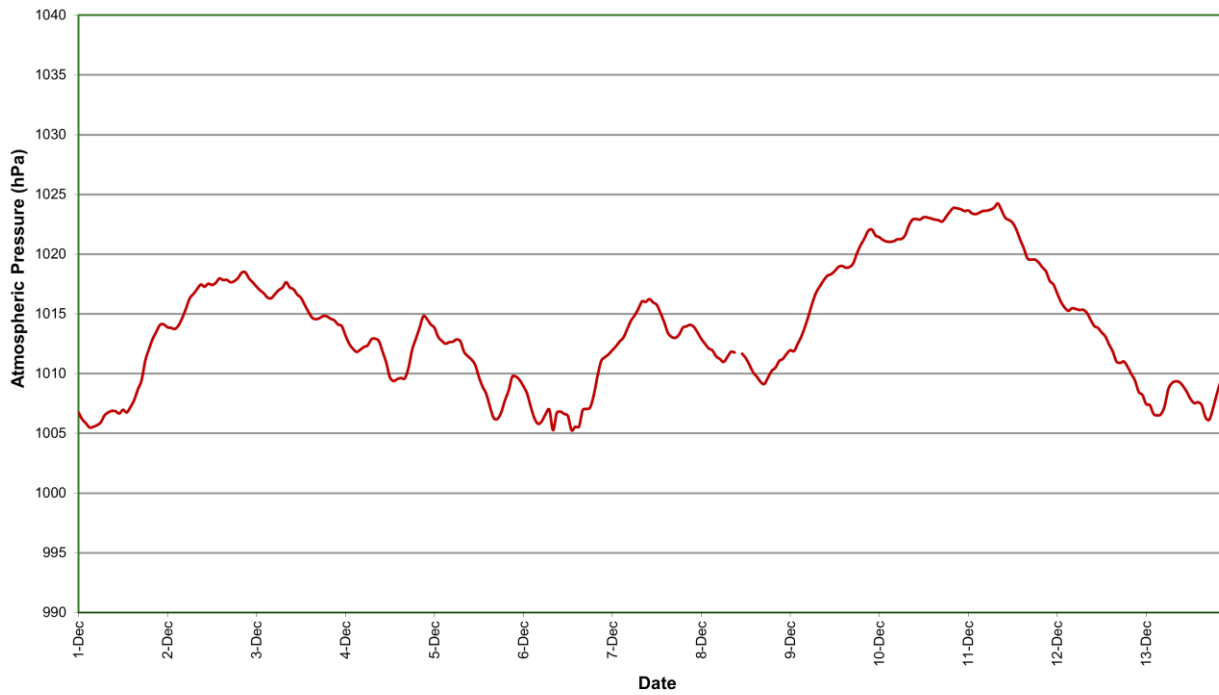
Figure 15: Atmospheric pressure (1 hour average) Station 4 Primula Avenue – December 2025
