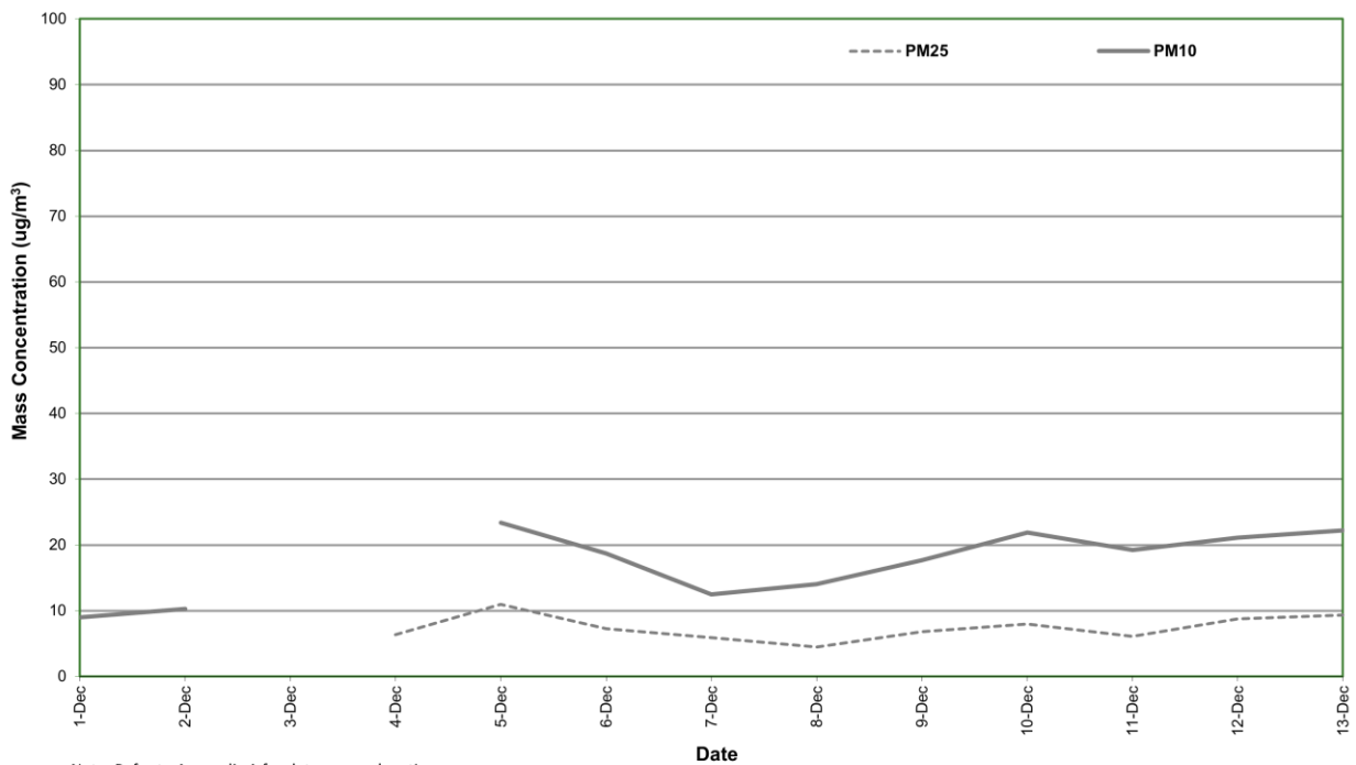
Figure 4: Station 3 PM 2.5 and PM 10 concentration (24 hour average) – December 2025
