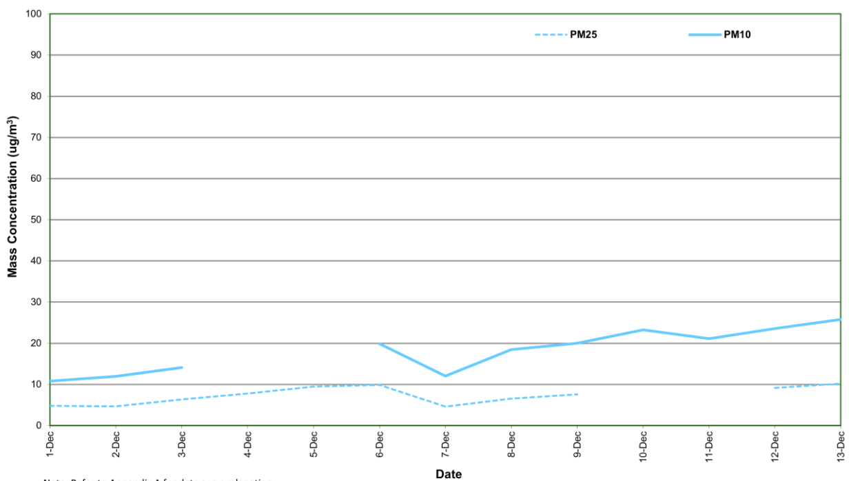
Figure 6: Station 5 PM 2.5 and PM 10 concentration (24 hour average) – December 2025
