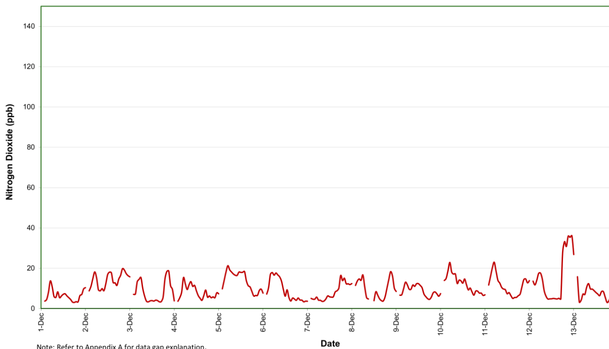
Figure 10: Station 4 NO 2 concentration (1 hour average) – December 2025
