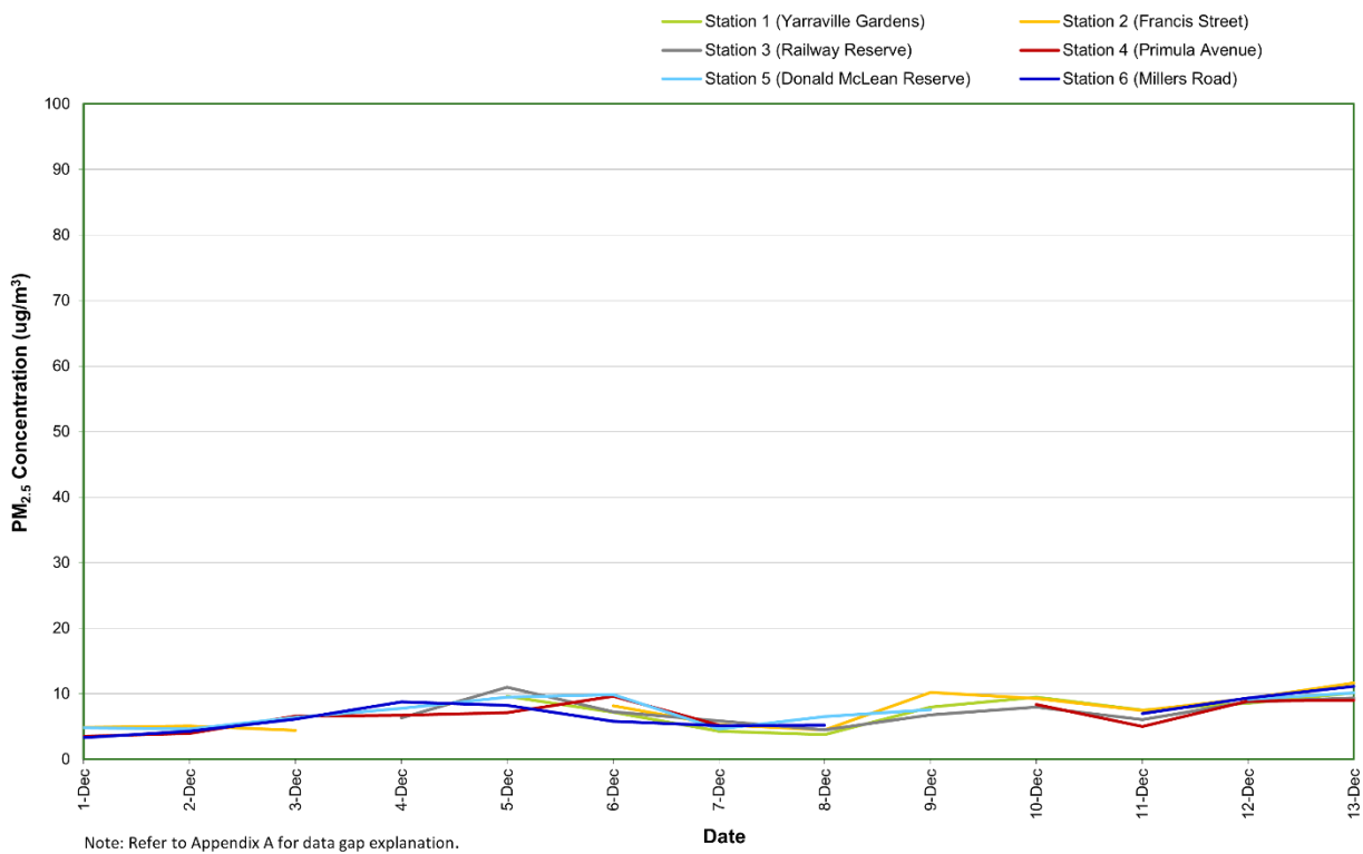
Figure 8: Combined PM 2.5 concentration (24 hour average) – December 2025
