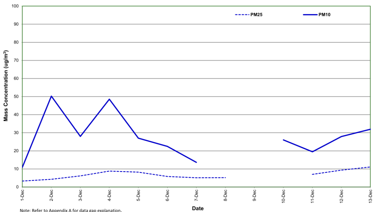
Figure 7: Station 6 PM 2.5 and PM 10 concentration (24 hour average) – December 2025
