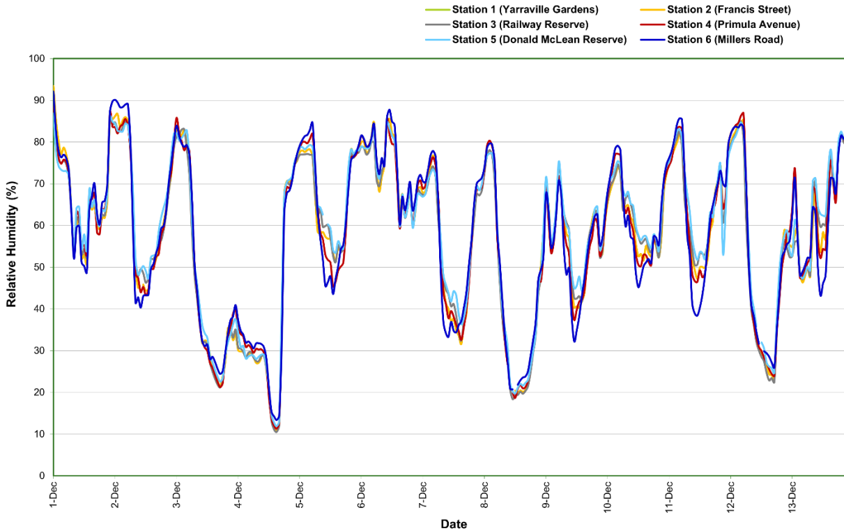
Figure 14: Relative humidity (1 hour average) All AAQMs – December 2025
