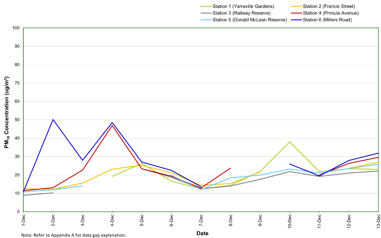
Figure 9: Combined PM 10 concentration (24 hour average) – December 2025
