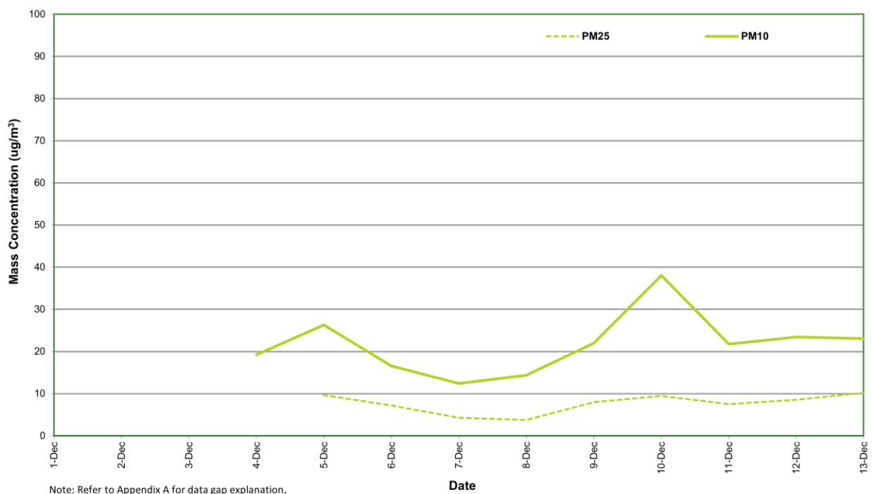
Figure 2: Station 1 PM 2.5 and PM 10 concentration (24 hour average) – December 2025
