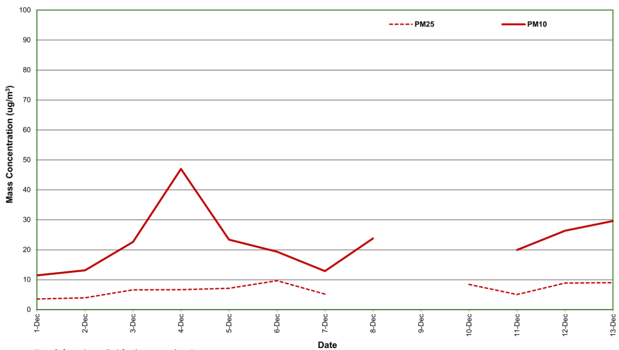
Figure 5: Station 4 PM 2.5 and PM 10 concentration (24 hour average) – December 2025
