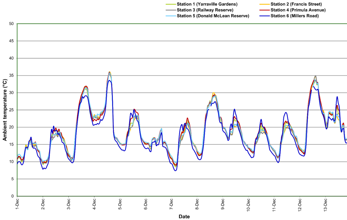
Figure 13: Ambient temperature (1 hour average) All AAQMS – December 2025
