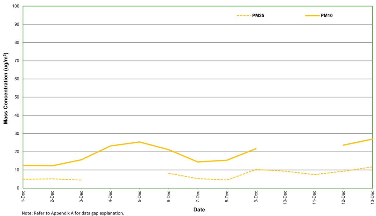
Figure 3: Station 2 PM 2.5 and PM 10 concentration (24 Hour Average) – December 2025
