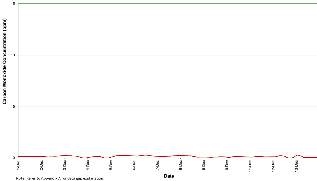
Figure 12: Station 4 CO concentration (8 hour rolling average) – December 2025
