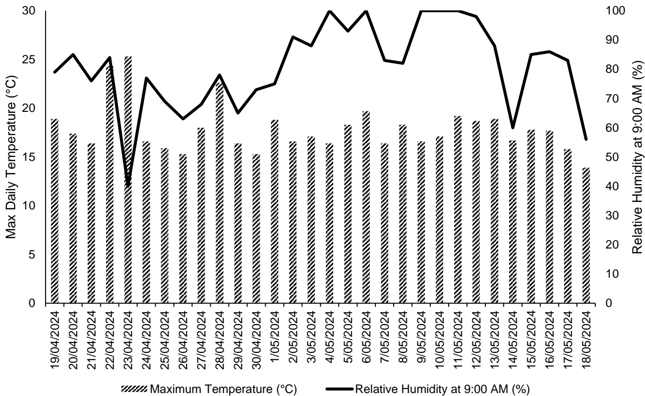
Figure 15: Daily relative humidity and temperature observations for Melbourne (Olympic Park), Victoria 19 April 2024 –18 May 2024. Data Source BOM.
