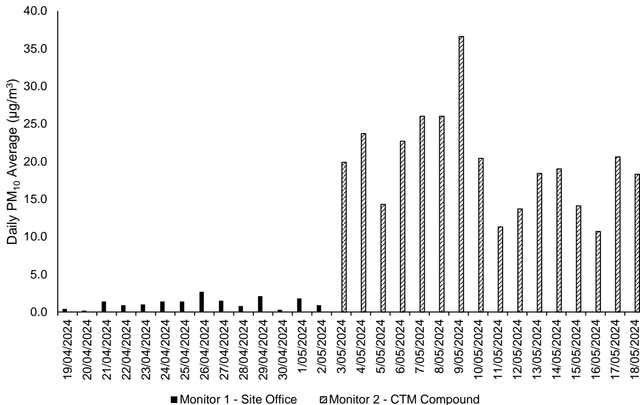
Figure 14: Cheltenham PM 10 daily averages
