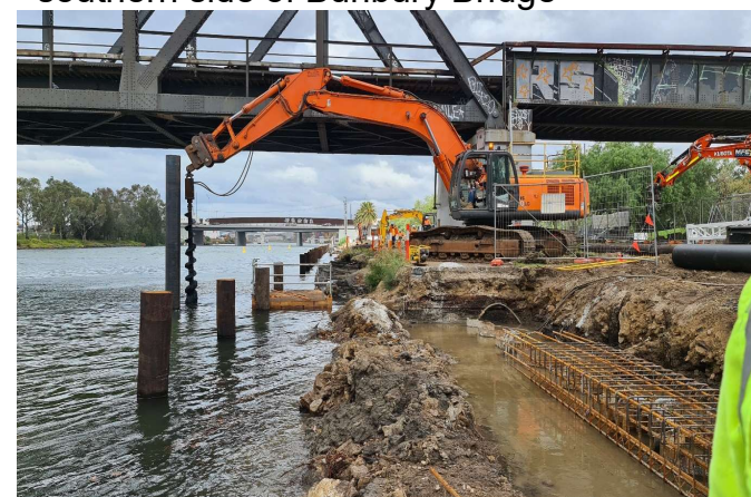
Steel Piling works and abutment reinforcement on southern side of Bunbury Bridge
