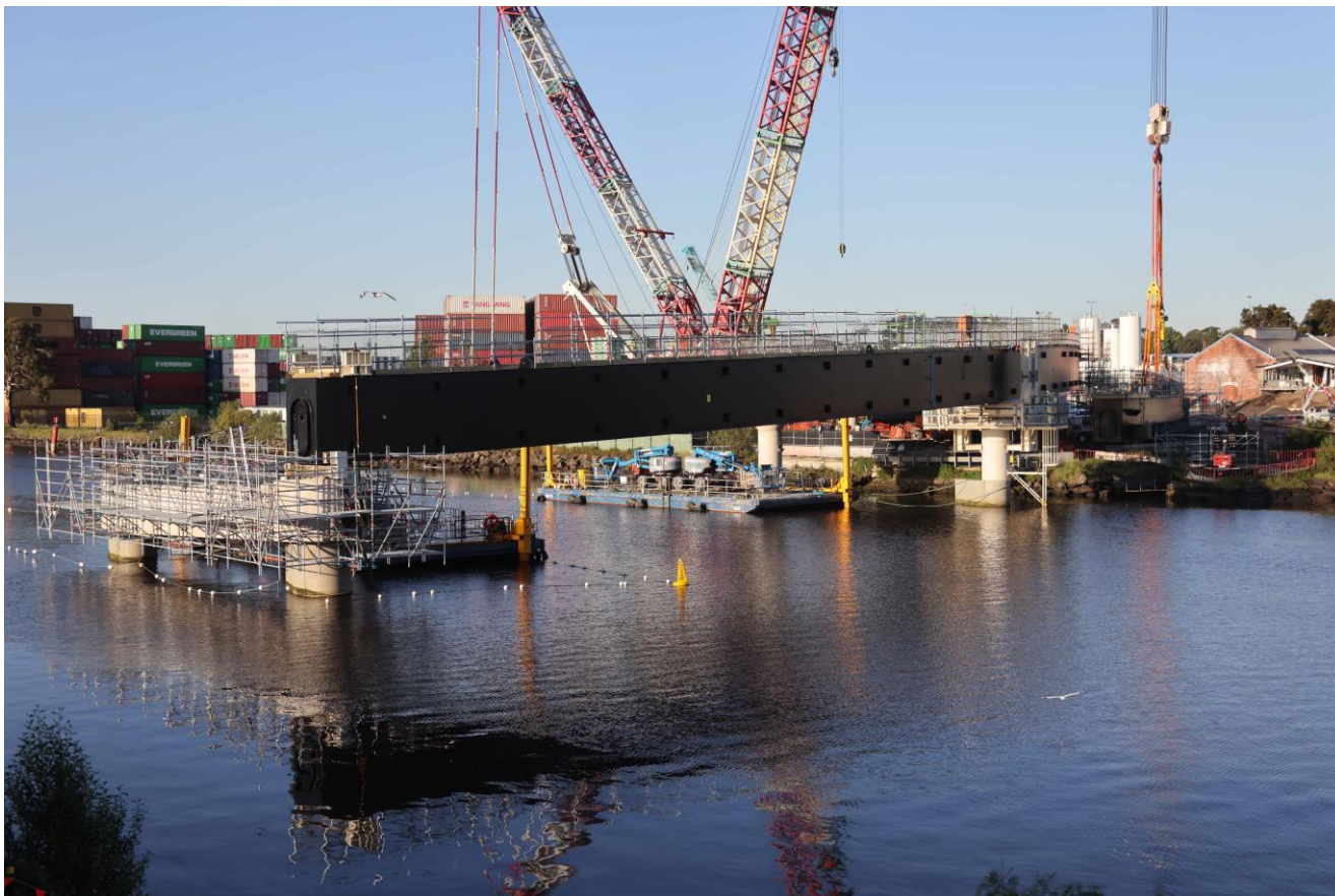
Steel beam lift – Bridge 50
