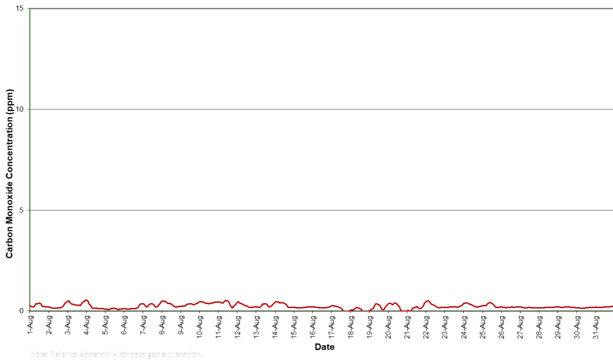
Figure 12: Station 4 CO concentration (8 hour rolling average) – August 2025
