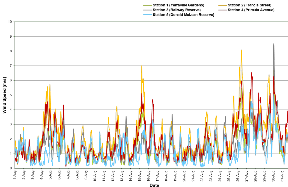
Figure 16: Wind speed (1 hour average) All AAQMs – August 2025
