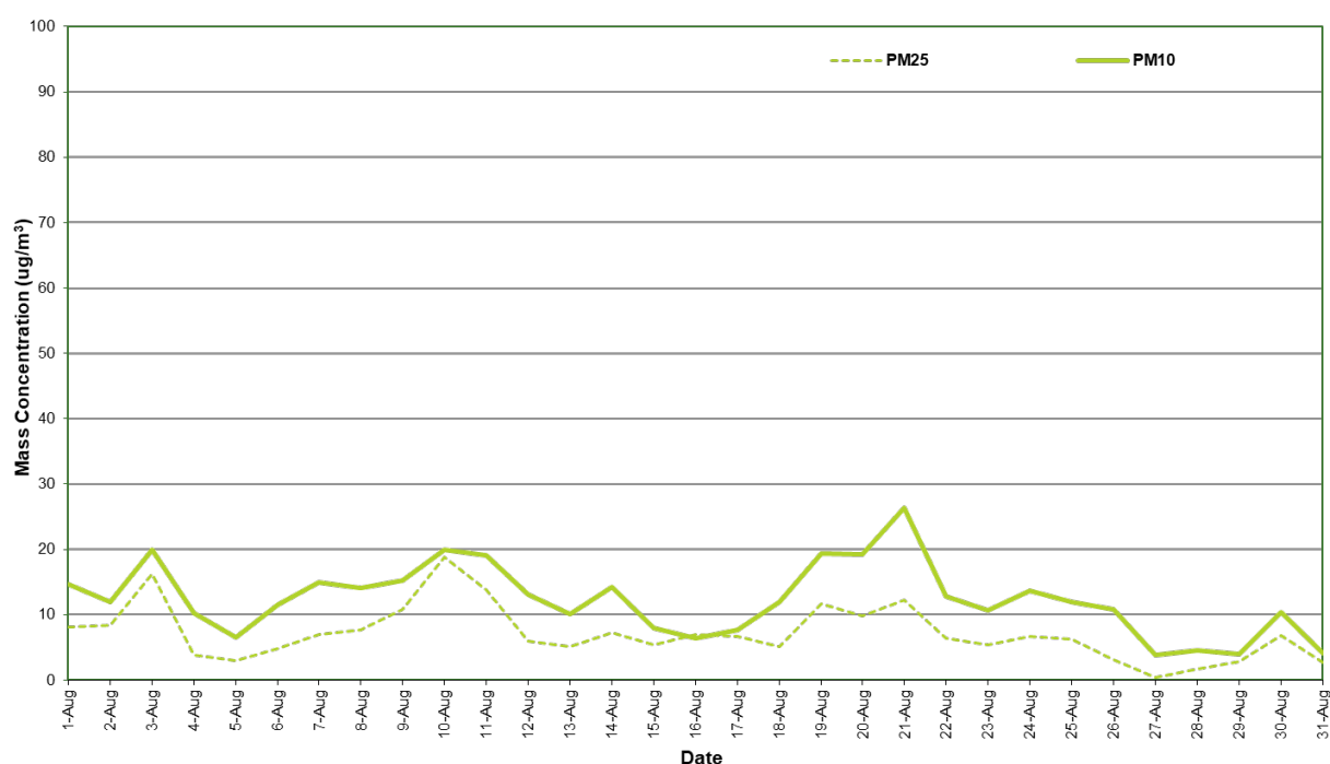
Figure 2: Station 1 PM 2.5 and PM 10 concentration (24 hour average) – August 2025
