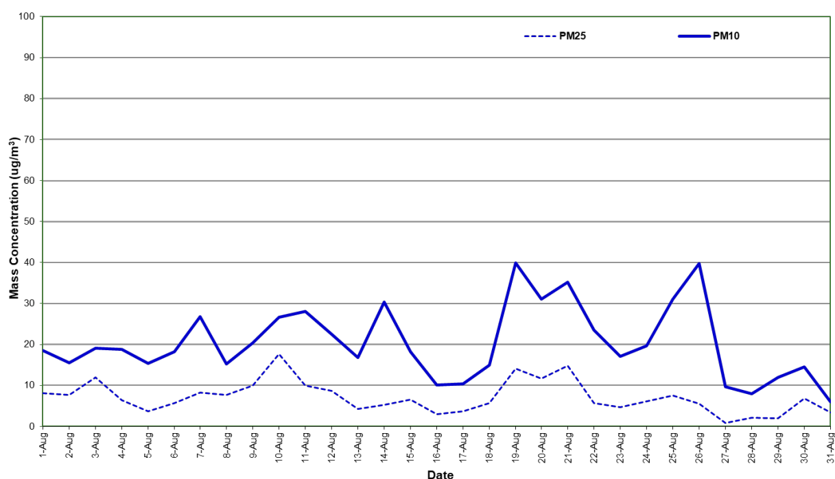
Figure 7: Station 6 PM 2.5 and PM 10 concentration (24 hour average) – August 2025
