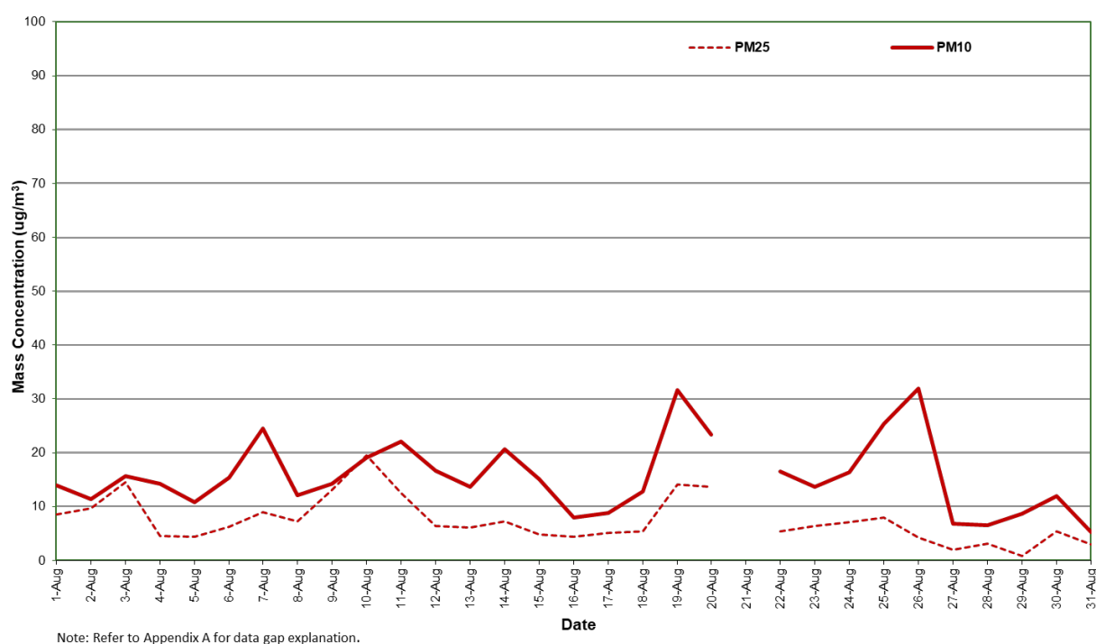
Figure 5: Station 4 PM 2.5 and PM 10 concentration (24 hour average) – August 2025
