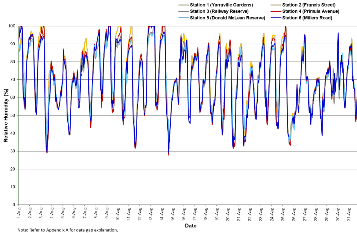
Figure 14: Relative humidity (1 hour average) All AAQMs – August 2025
