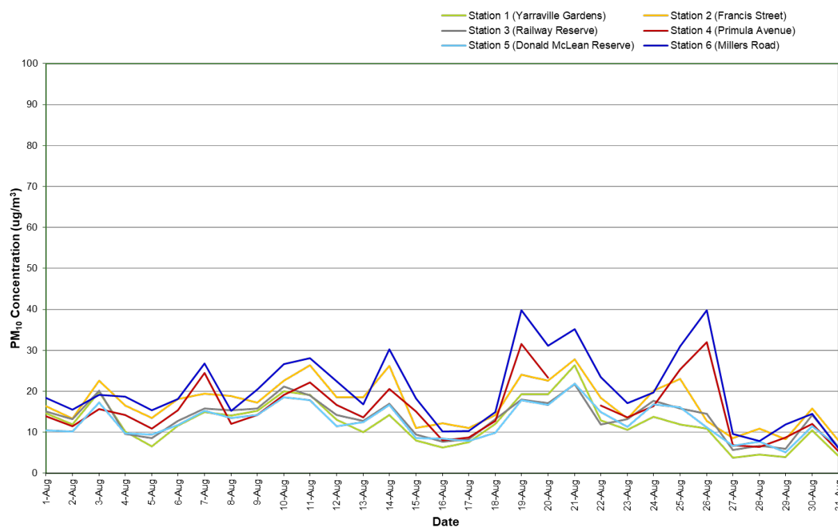
Figure 9: Combined PM 10 concentration (24 hour average) – August 2025
