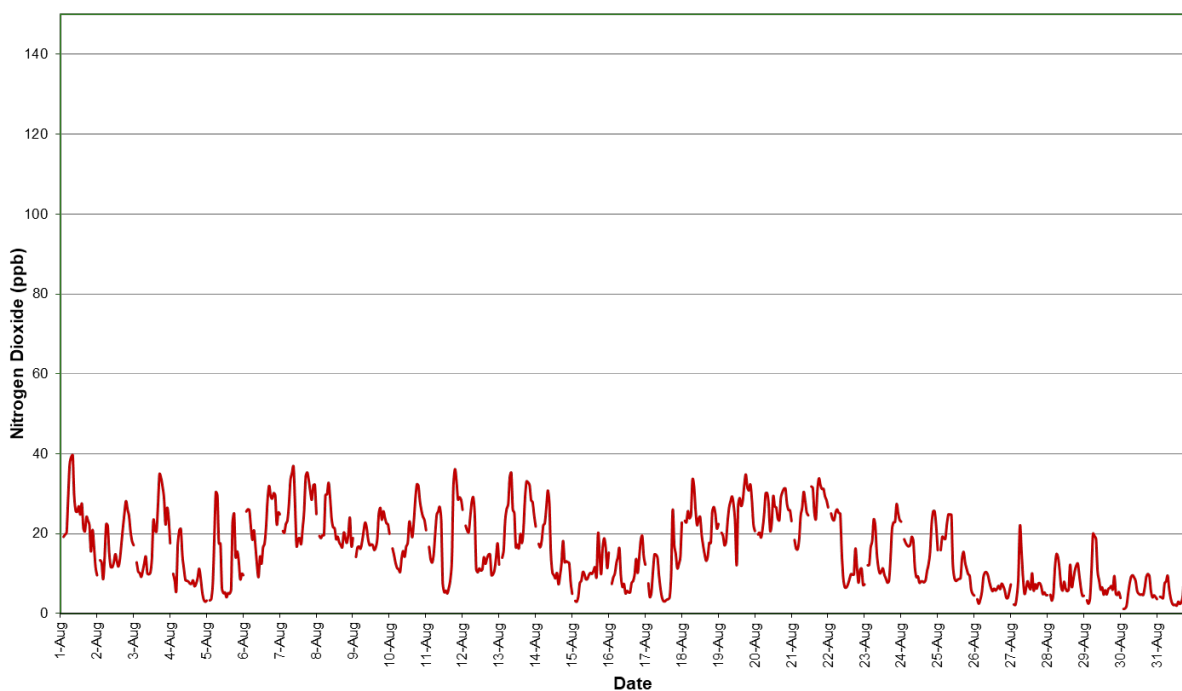
Figure 10: Station 4 NO 2 concentration (1 hour average) – August 2025
