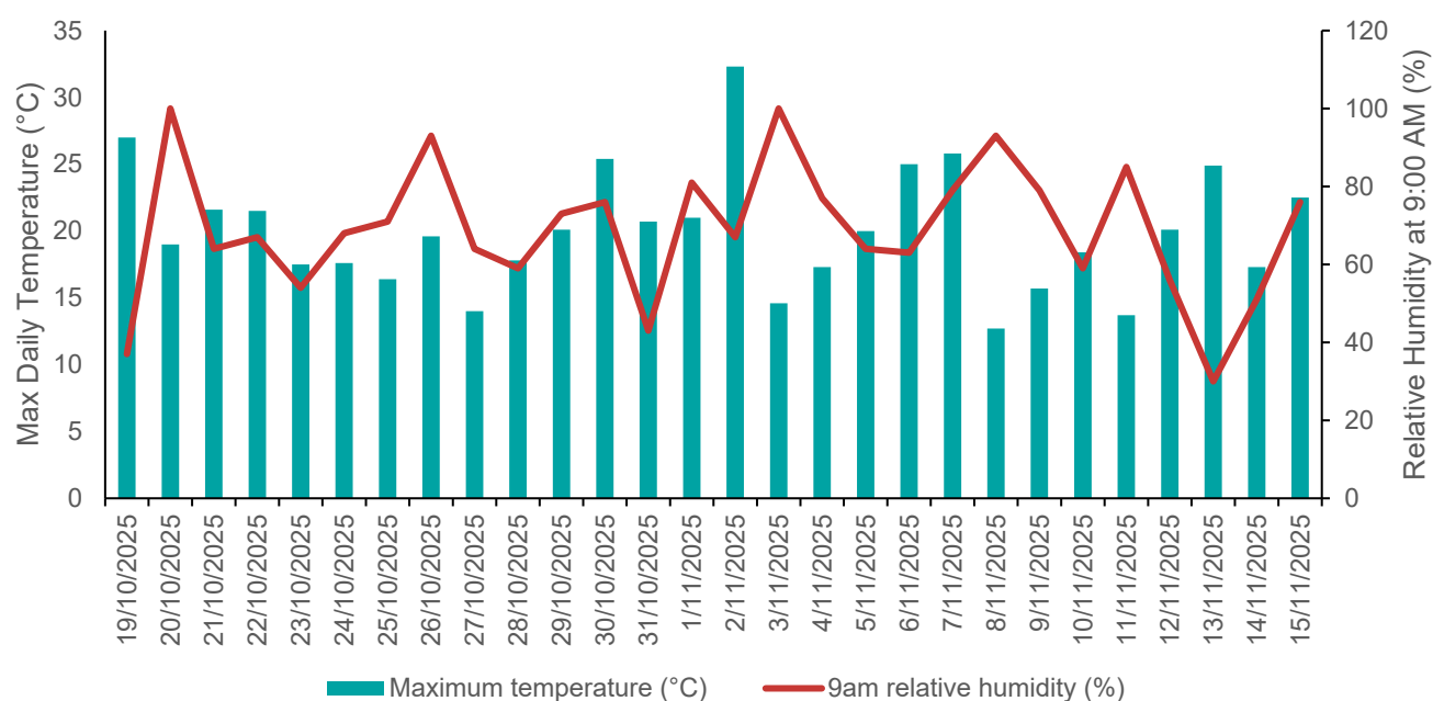
Figure 5: Daily relative humidity and temperature observations for Melbourne (Olympic Park), Victoria 19/10/2025 – 15/11/2025. Data Source BOM.
