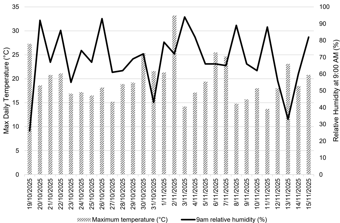
Figure 8: Daily relative humidity and temperature observations for Melbourne (Moorabbin), Victoria 19 October 2025 – 15 November 2025. Data Source BOM.
