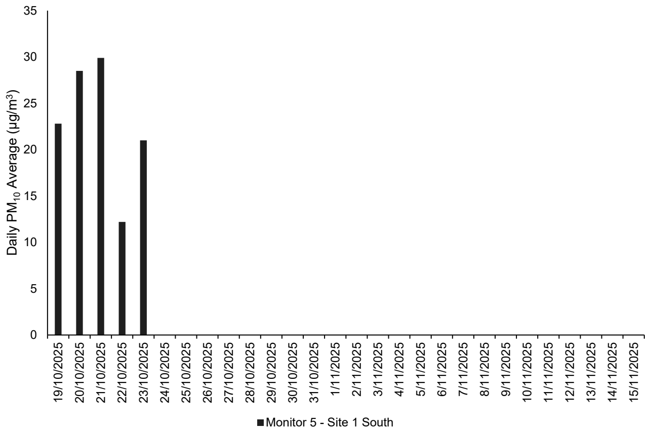
Figure 2: Burwood PM 10 daily averages.
