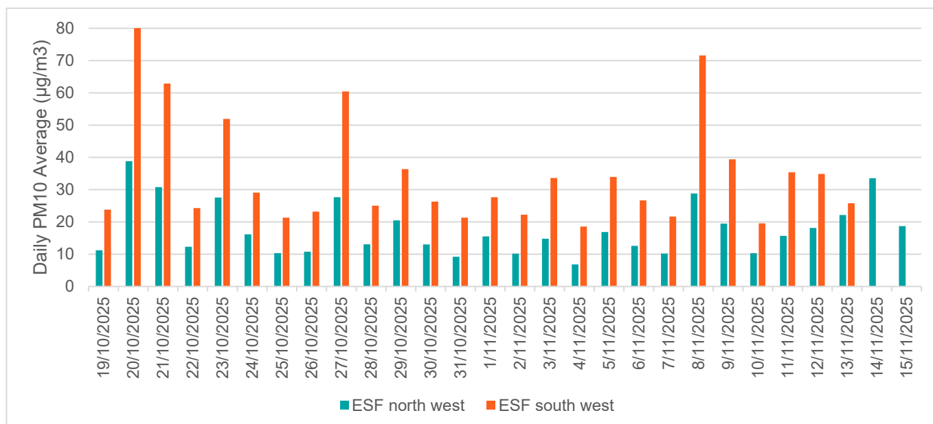
Figure 2: ESF PM 10 daily averages from 19 October to 15 November
