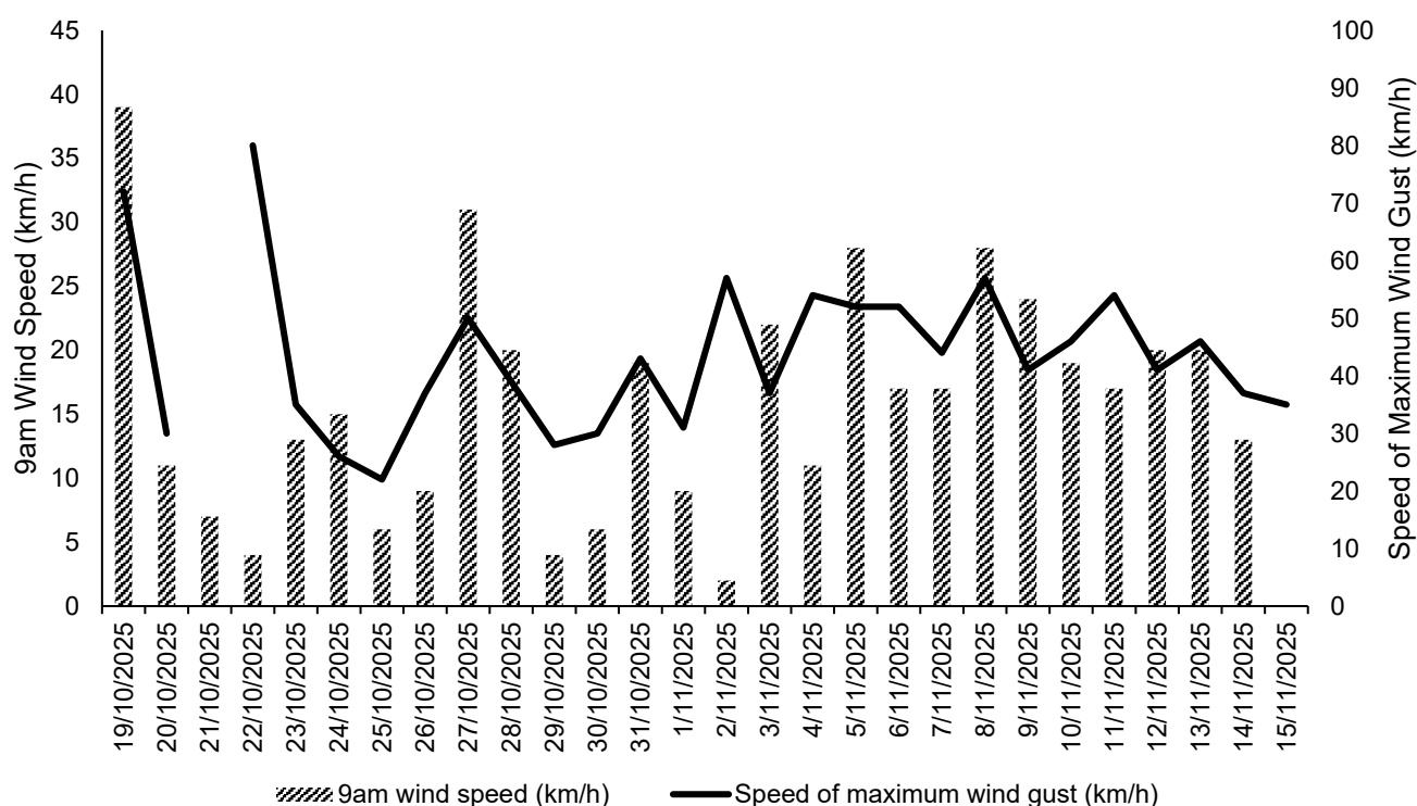
Figure 10: Daily wind speed observations for Melbourne (Moorabbin), Victoria 19 October 2025 – 15 November 2025. Data Source BOM.
