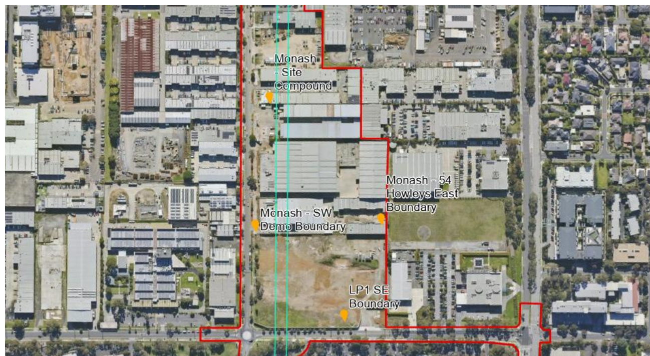
Figure 7: Monash air quality monitoring stations
