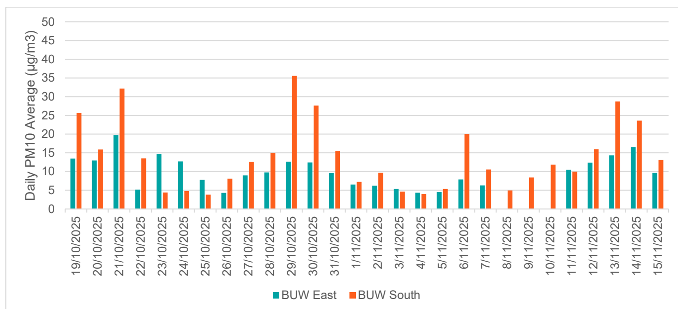
Figure 4. Burwood PM 10 daily averages from 19 October to 15 November
