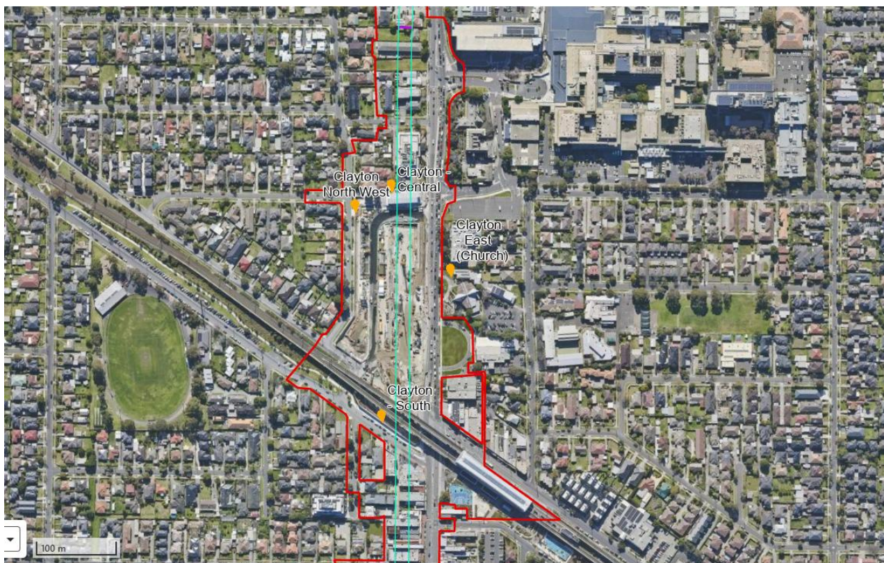
Figure 5: Clayton air quality monitoring stations
