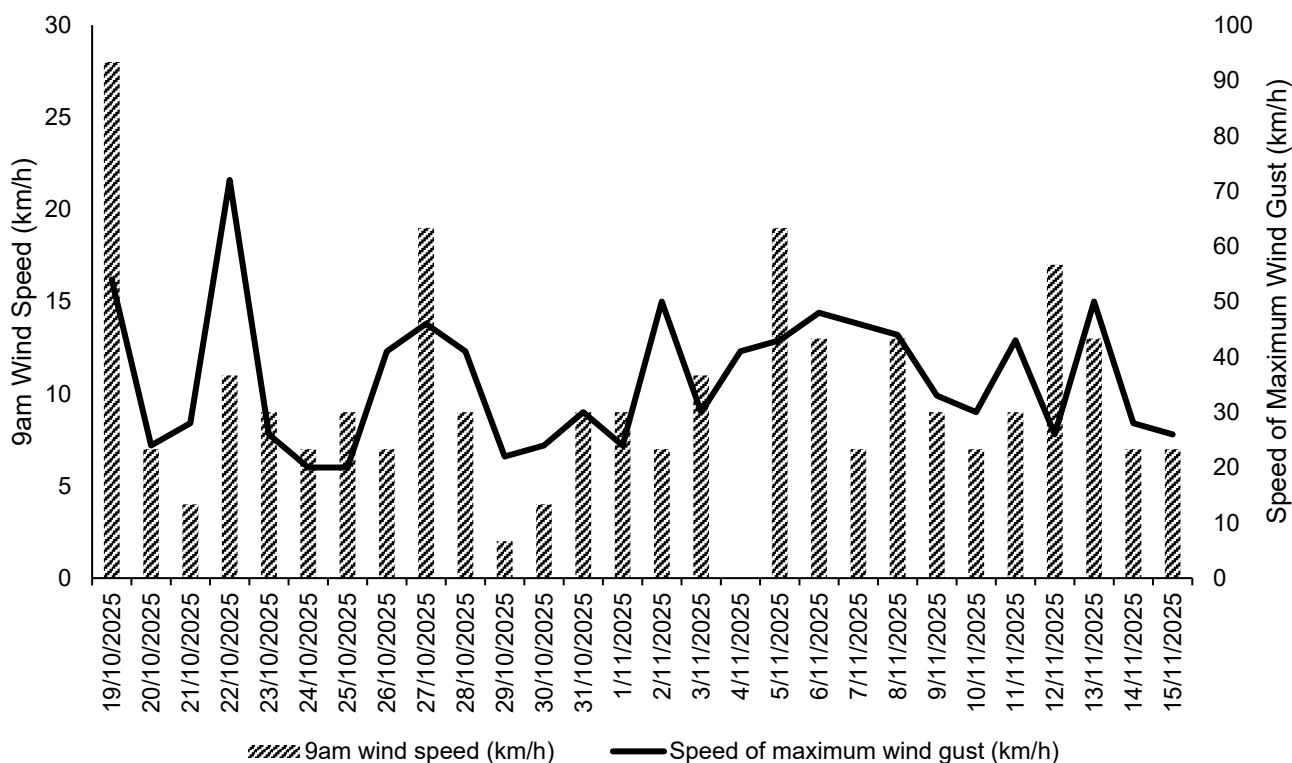
Figure 9: Daily wind speed observations for Melbourne (Olympic Park), Victoria 19 October 2025 – 15 November 2025. Data Source BOM.
