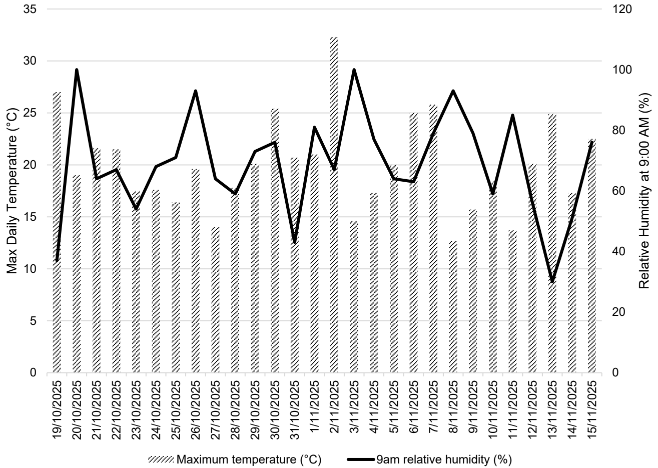
Figure 7: Daily relative humidity and temperature observations for Melbourne (Olympic Park), Victoria 19 October 2025 – 15 November 2025. Data Source BOM.
