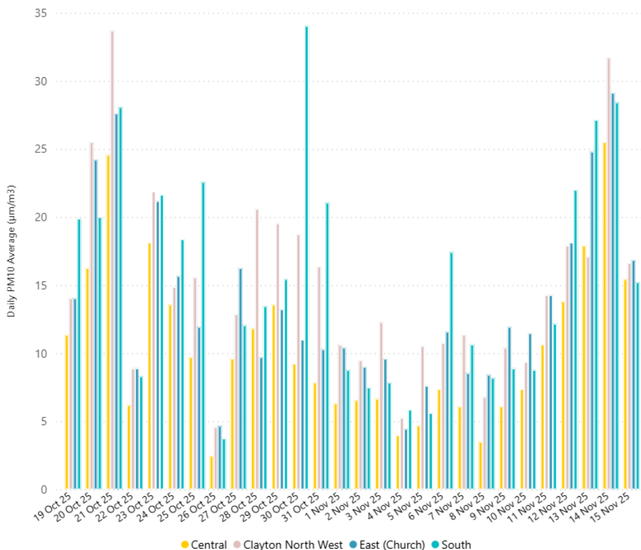
Figure 6: Daily Averages PM10 Results at Clayton Site
