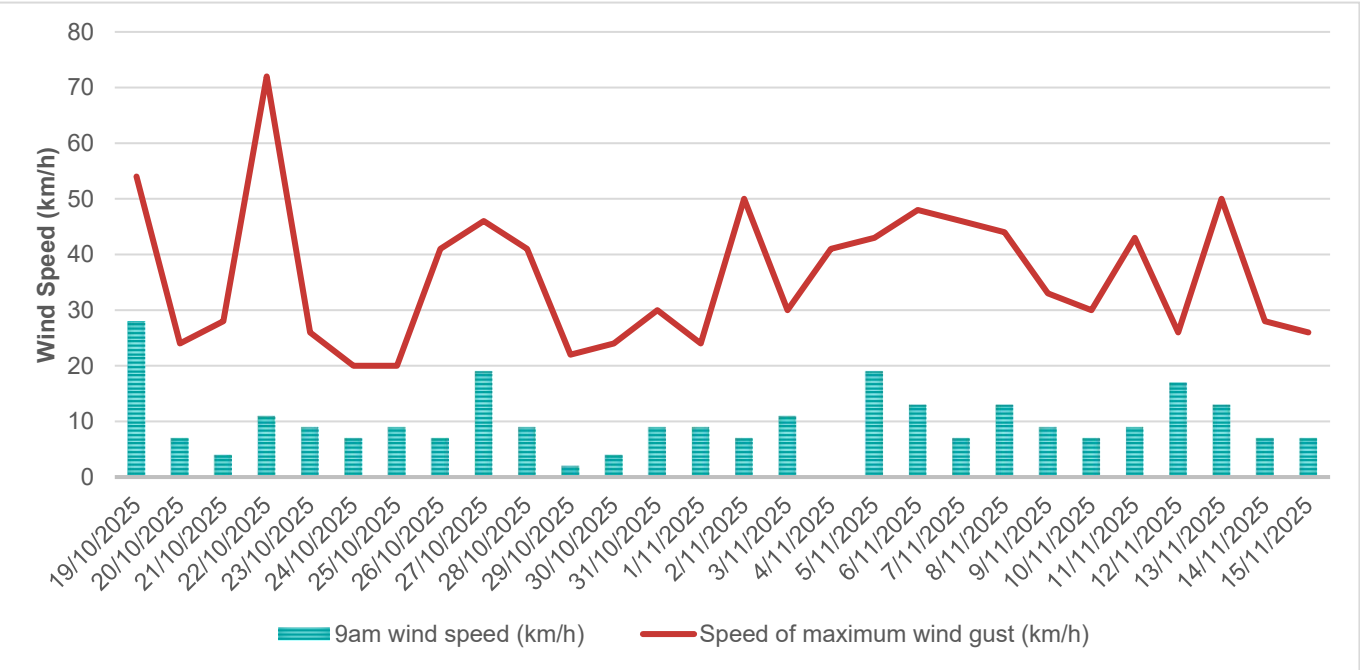
Figure 6. Daily wind speed observations for Melbourne (Olympic Park), Victoria 19/10/2025 – 15/11/2025. Data Source BOM
