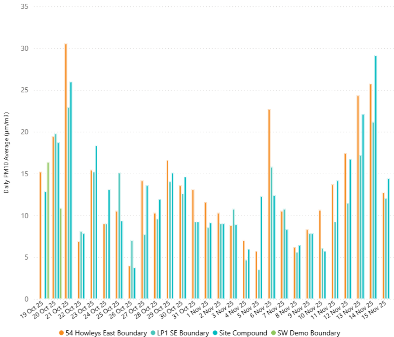
Figure 8: Daily Averages PM10 Results at Monash
