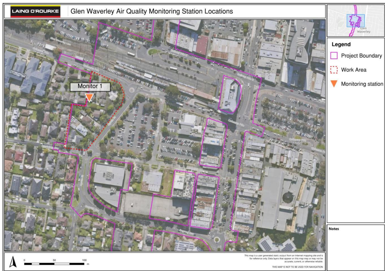
Figure 3: Glen Waverley air quality monitoring stations.
