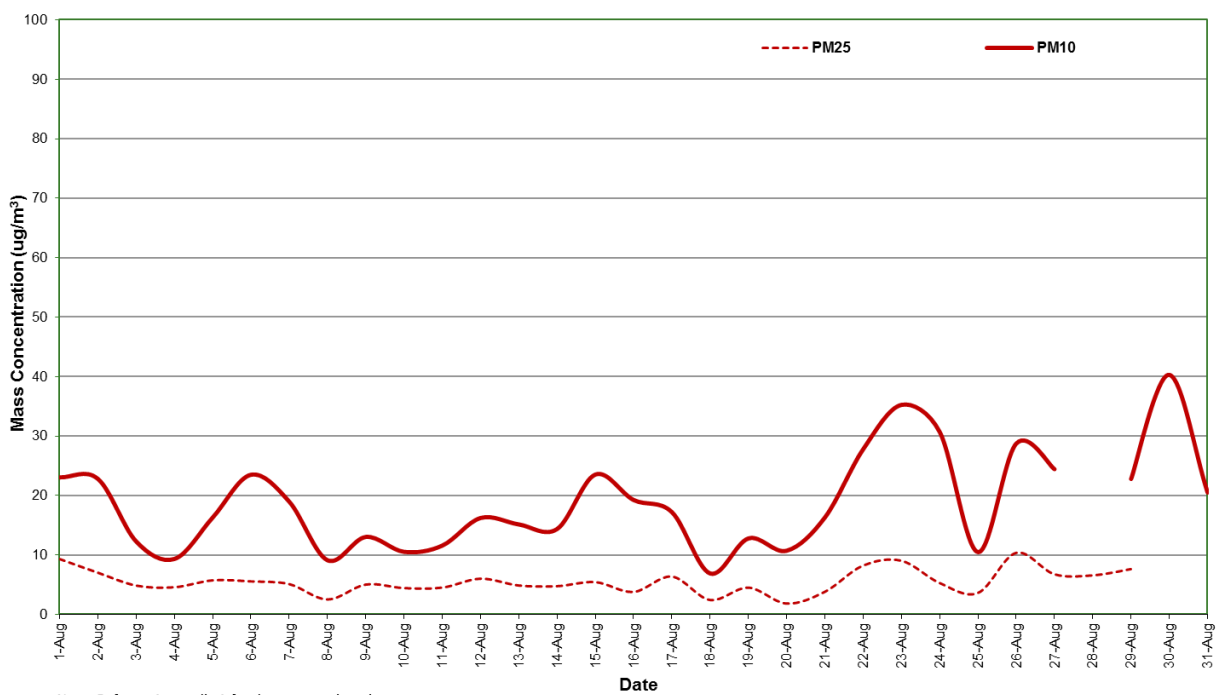
Figure 5: Station 4 PM 2.5 and PM 10 concentration (24 hour average) – August 2019
