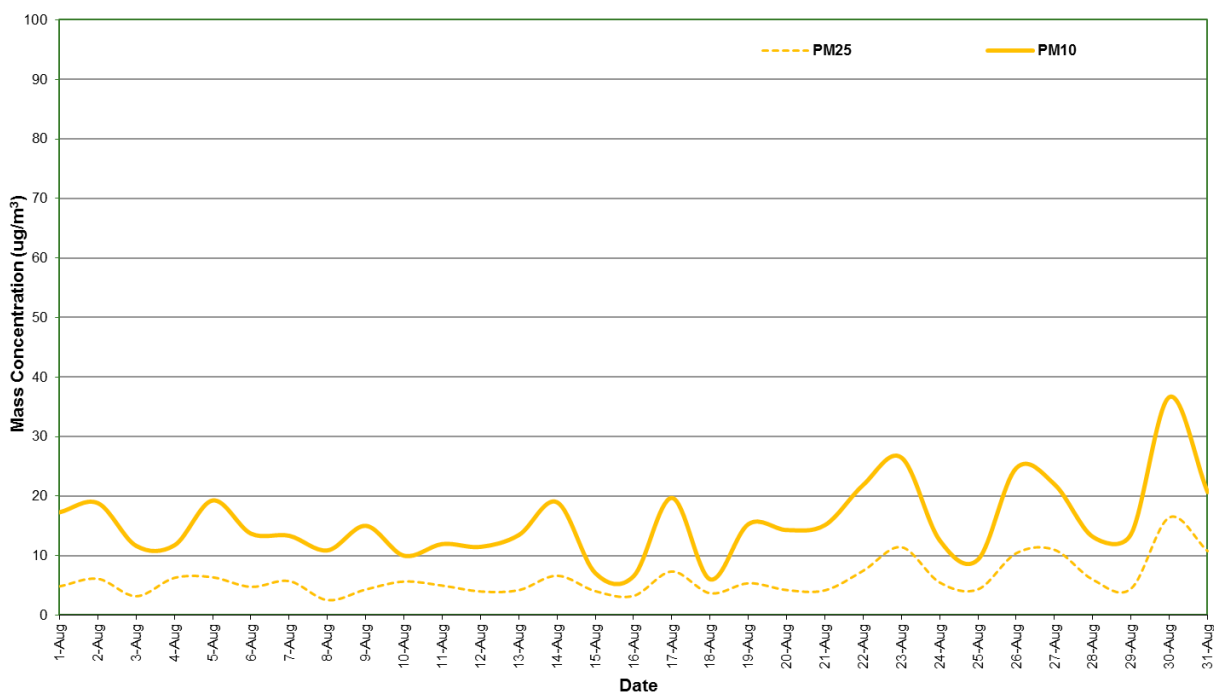
Figure 3: Station 2 PM 2.5 and PM 10 concentration (24 Hour Average) – August 2019
