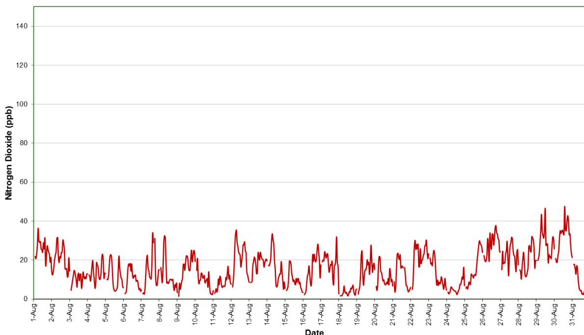
Figure 10: Station 4 NO 2 concentration (1 hour average) – August 2019
