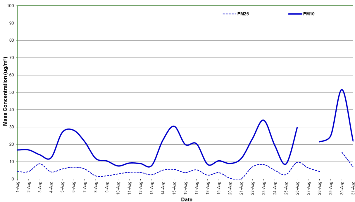
Figure 7: Station 6 PM 2.5 and PM 10 concentration (24 hour average) – August 2019
