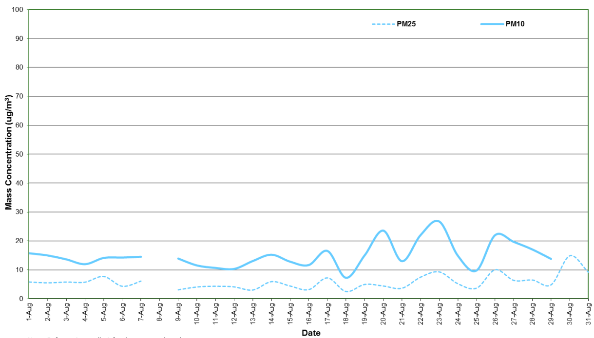
Figure 6: Station 5 PM 2.5 and PM 10 concentration (24 hour average) – August 2019
