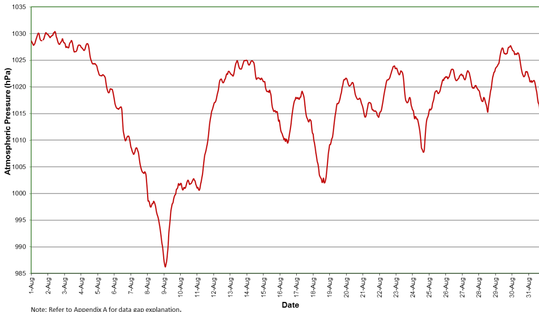
Figure 14: Atmospheric pressure (1 hour average) Station 4 Primula Avenue - August 2019
