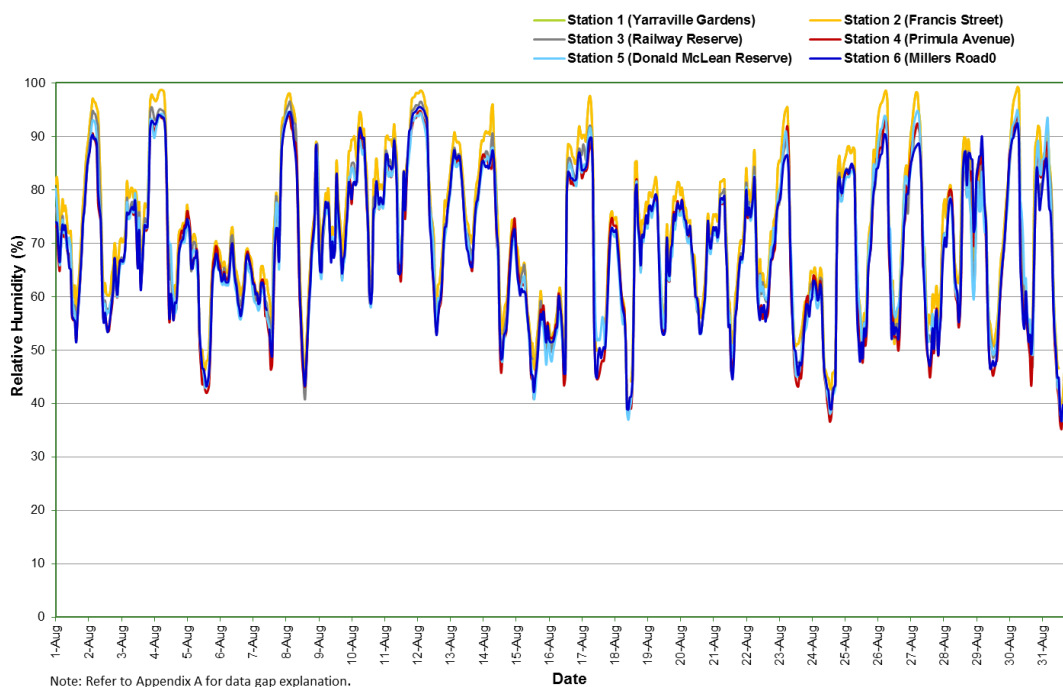
Figure 13: Relative humidity (1 hour average) All AAQMs – August 2019
