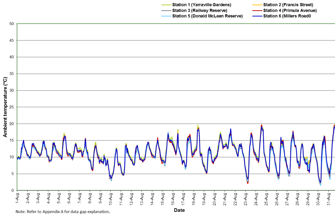
Figure 12: Ambient temperature (1 hour average) All AAQMS – August 2019
