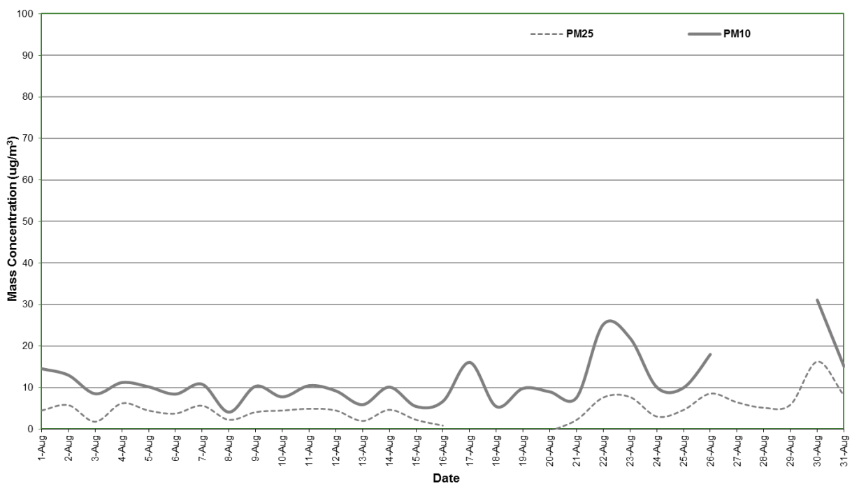
Figure 4: Station 3 PM 2.5 and PM 10 concentration (24 hour average) – August 2019
