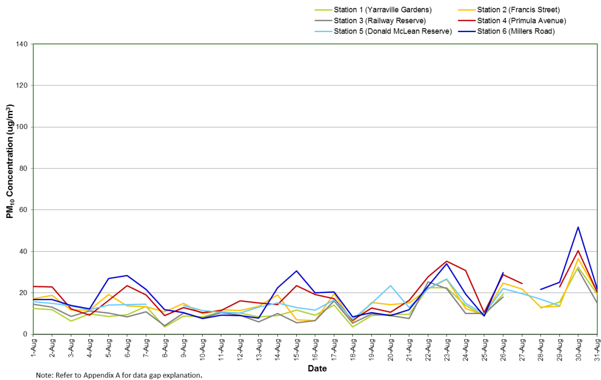
Figure 9: Combined PM 10 concentration (24 hour average) – August 2019
