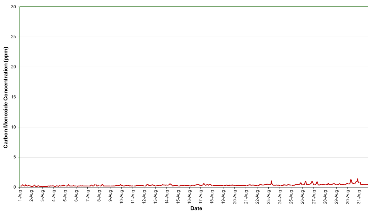
Figure 11: Station 4 CO concentration (1 hour average) – August 2019
