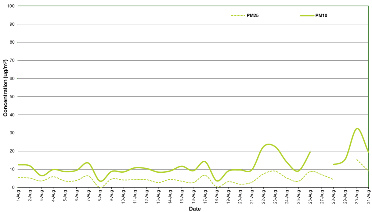
Figure 2: Station 1 PM 2.5 and PM 10 concentration (24 hour average) – August 2019
