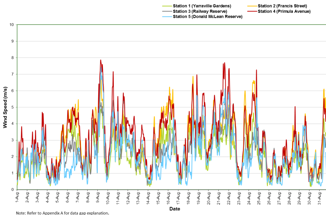
Figure 15: Wind speed (1 hour average) All AAQMs – August 2019
