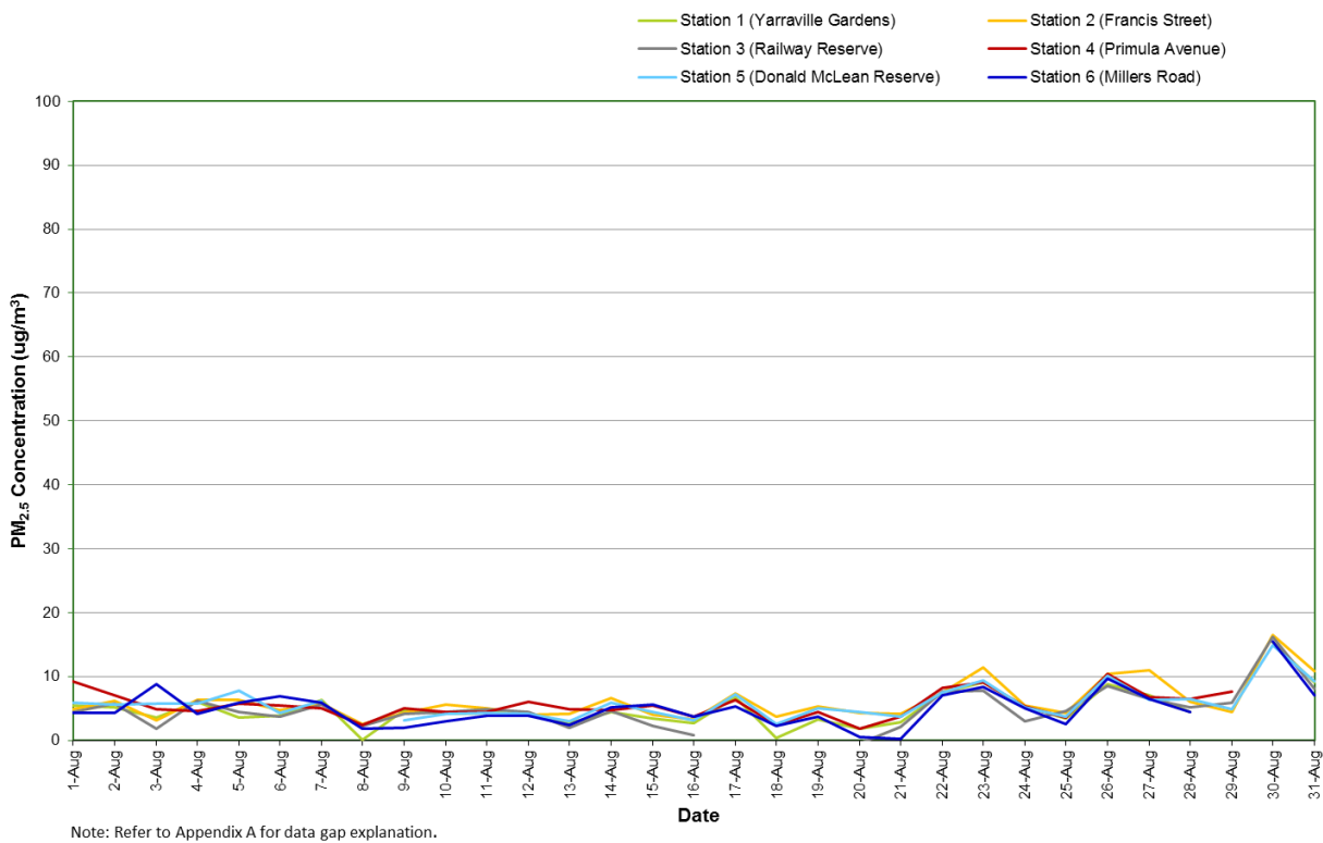
Figure 8: Combined PM 2.5 concentration (24 hour average) – August 2019
