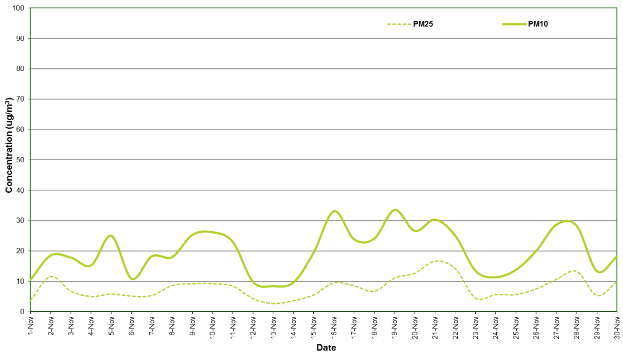
Figure 2: Station 1 PM 2.5 and PM 10 concentration (24 hour average) – November 2020
