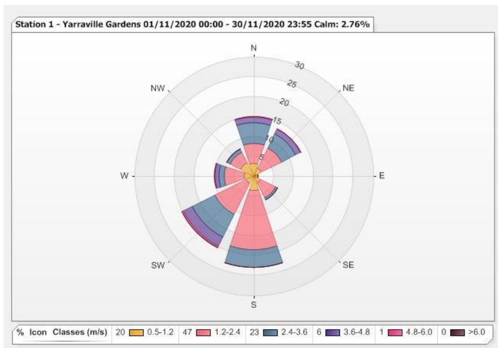
Figure 16: Wind speed (1 hour average) Station 1 - Yarrville Gardens
