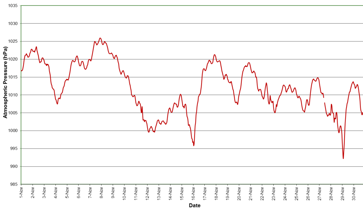
Figure 14: Atmospheric pressure (1 hour average) Station 4 Primula Avenue – November 2020
