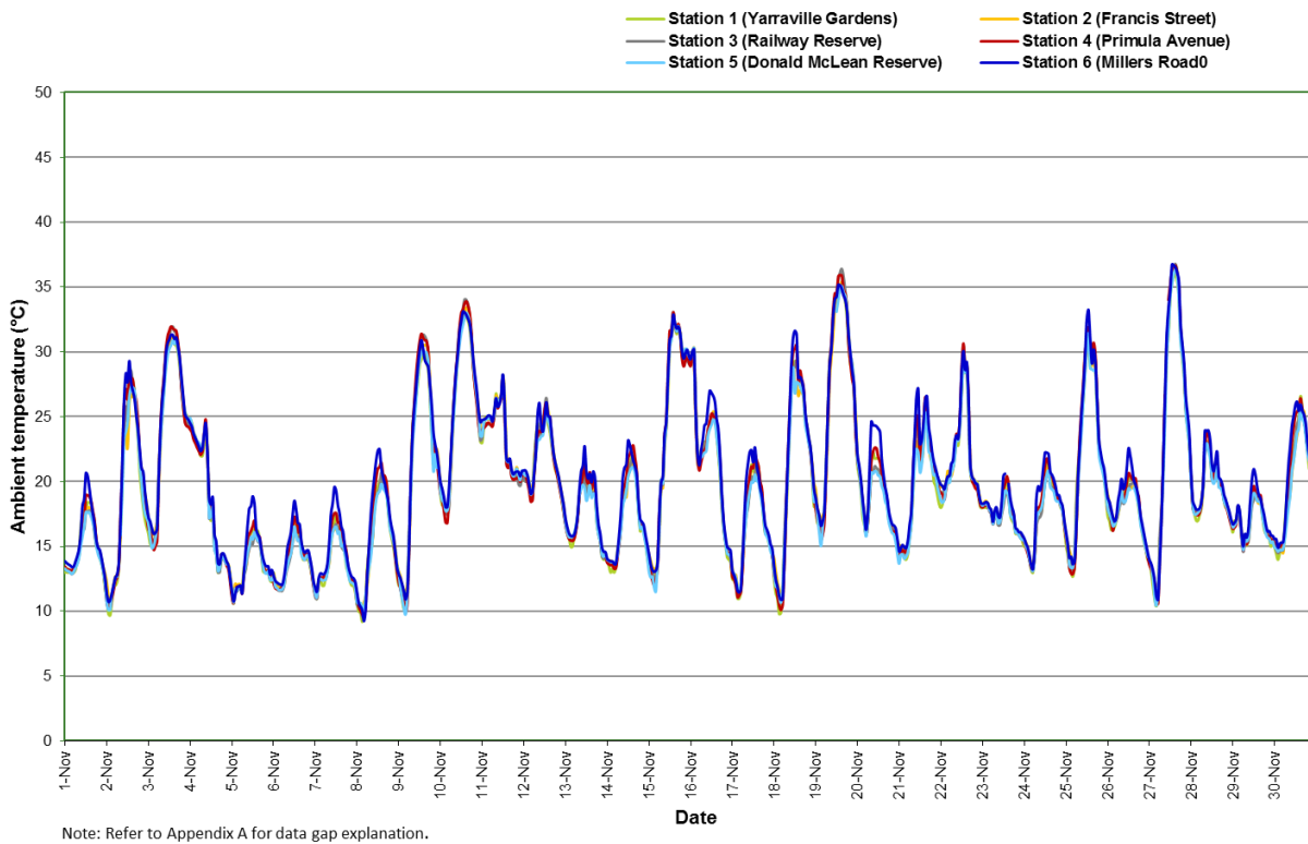
Figure 12: Ambient temperature (1 hour average) All AAQMS – November 2020
