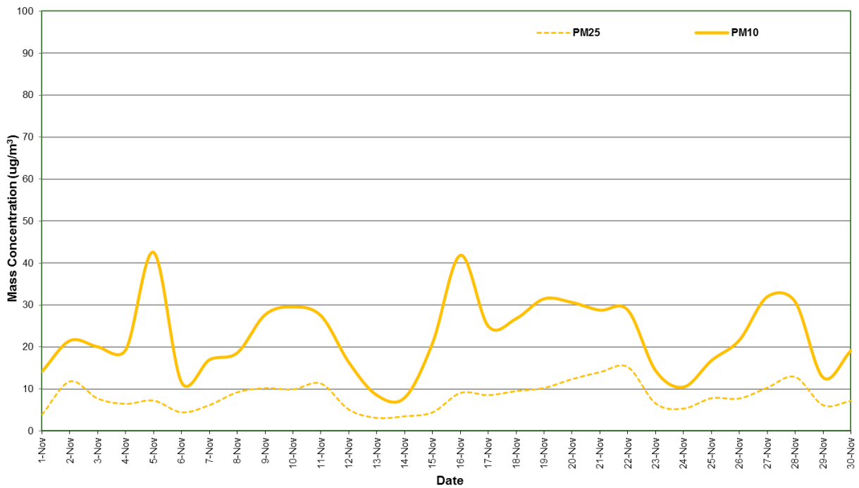
Figure 3: Station 2 PM 2.5 and PM 10 concentration (24 Hour Average) – November 2020
