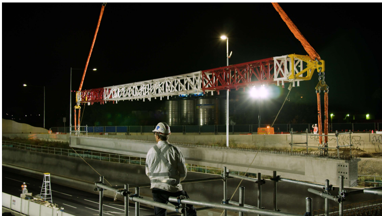
Installing the new concrete beams that will become the new bridge at Grieve Parade – end of January 2021
