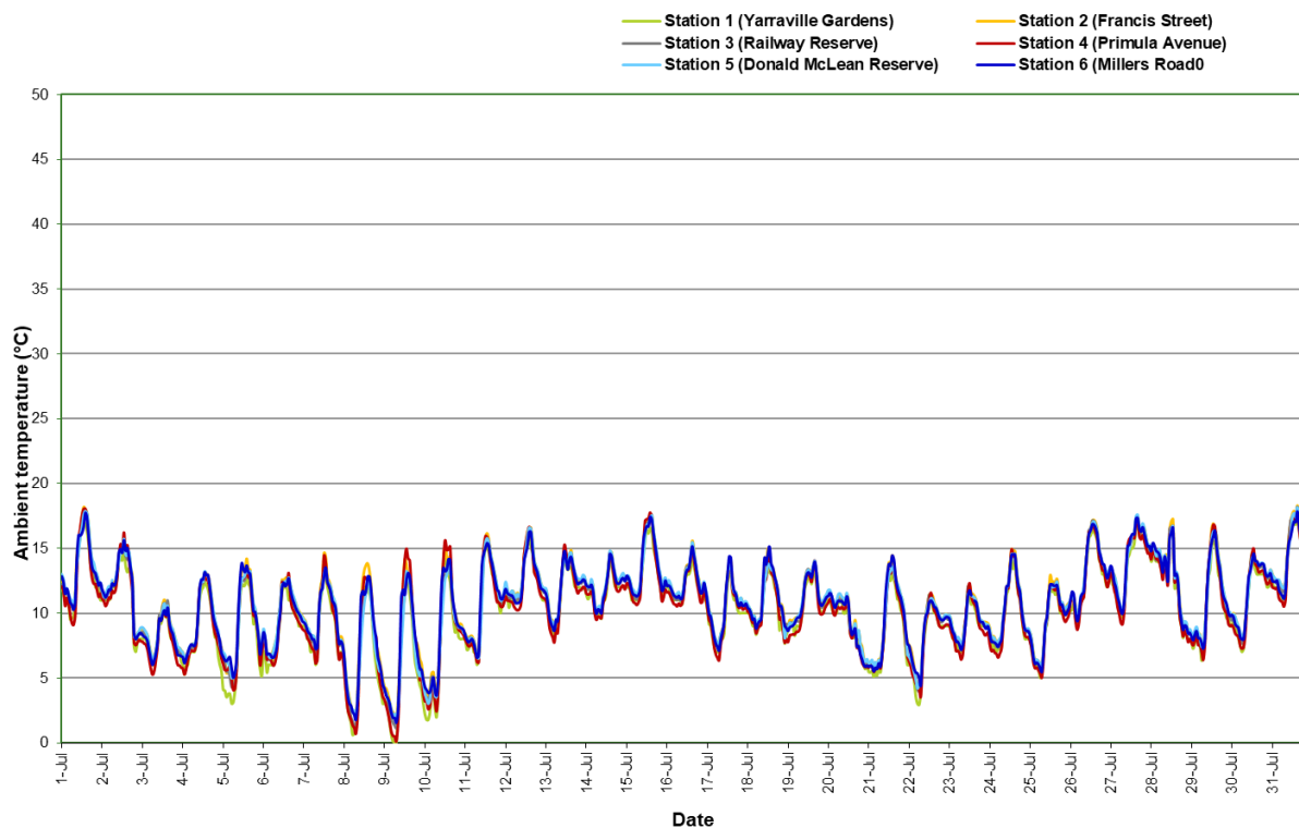
Figure 12: Ambient temperature (1 hour average) All AAQMS – July 2021
