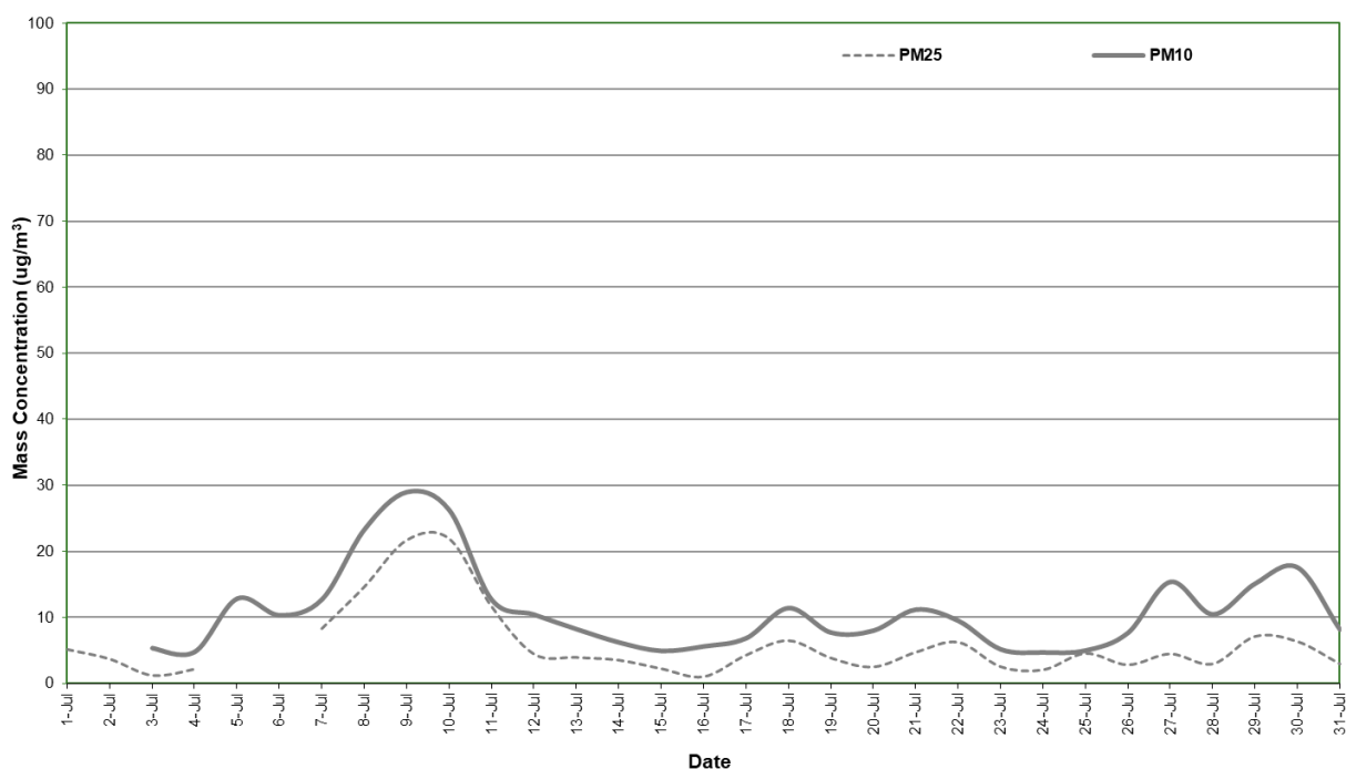
Figure 4: Station 3 PM 2.5 and PM 10 concentration (24 hour average) – July 2021
