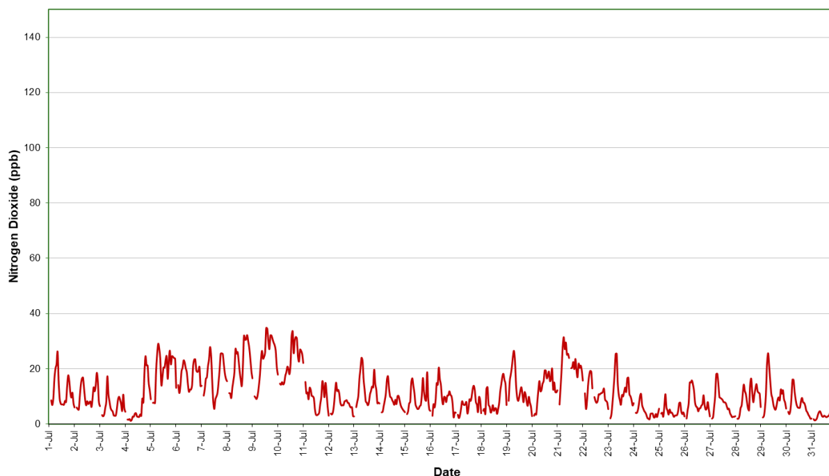
Figure 10: Station 4 NO 2 concentration (1 hour average) – July 2021
