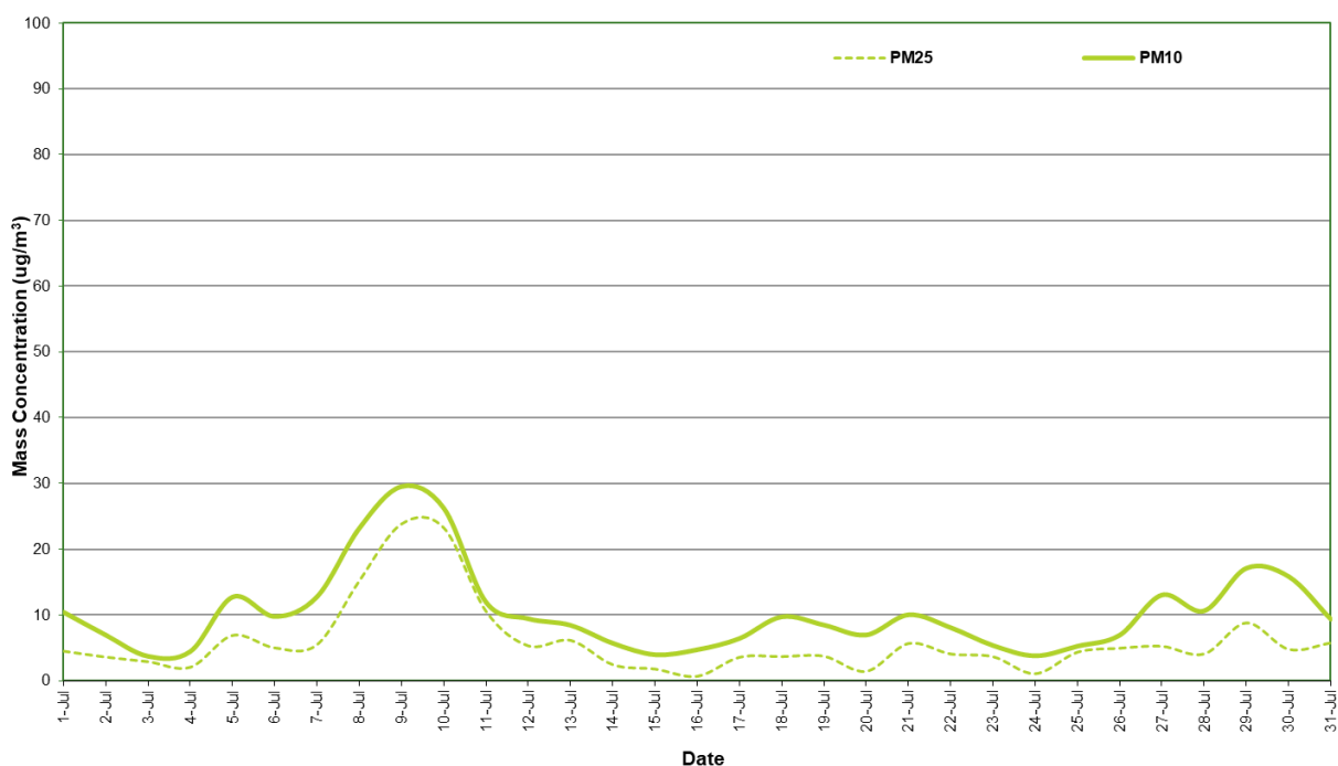
Figure 2: Station 1 PM 2.5 and PM 10 concentration (24 hour average) – July 2021
