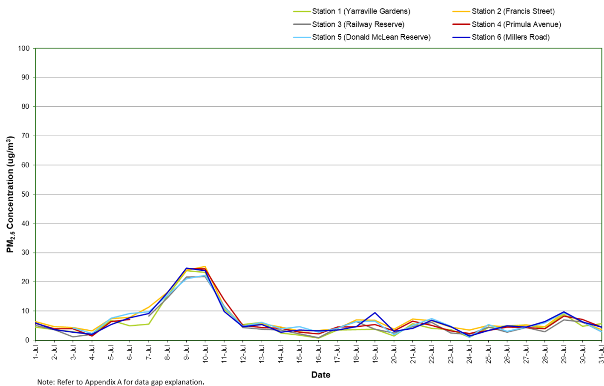
Figure 8: Combined PM 2.5 concentration (24 hour average) – July 2021
