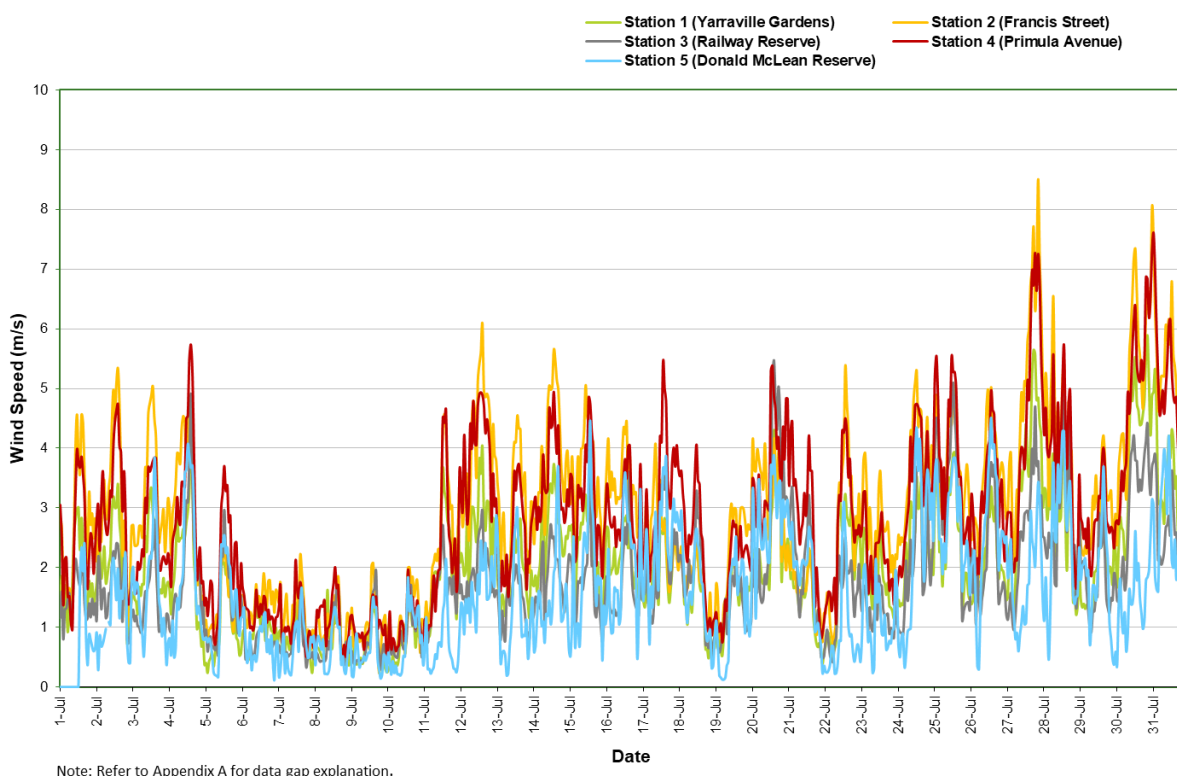
Figure 15: Wind speed (1 hour average) All AAQMs – July 2021
