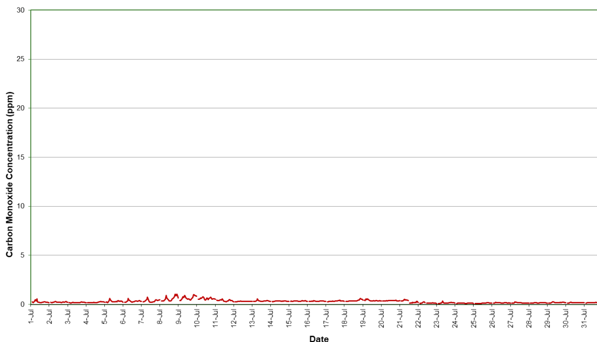
Figure 11: Station 4 CO concentration (1 hour average) – July 2021
