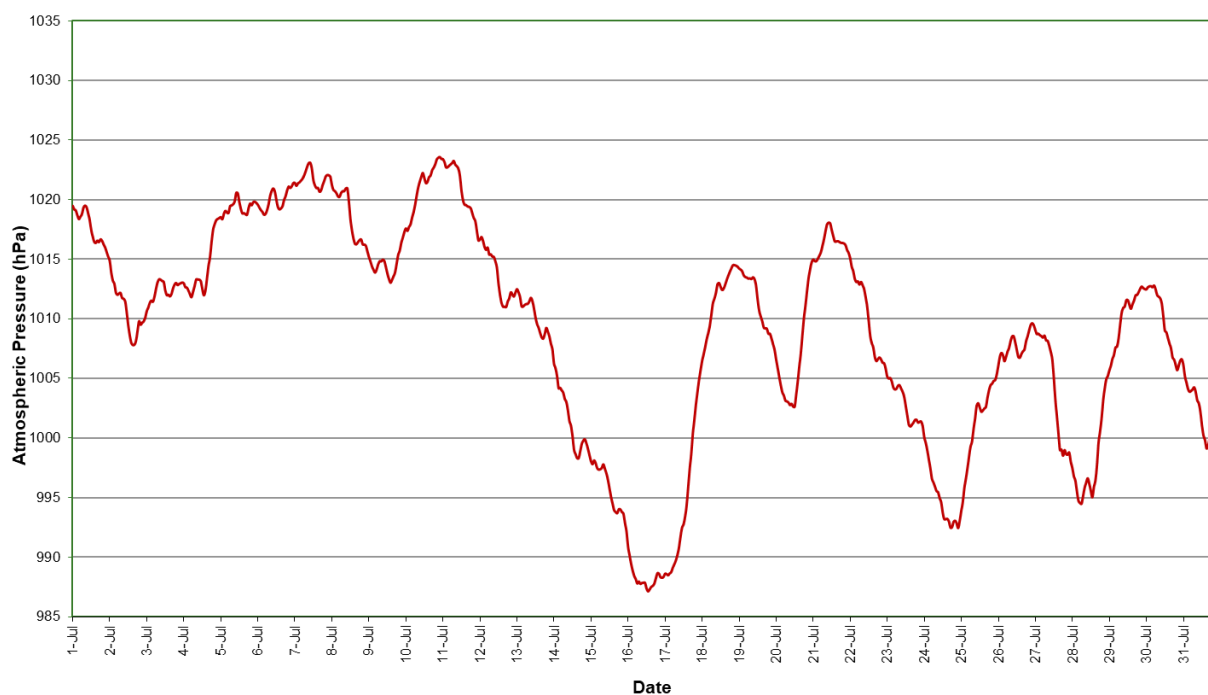
Figure 14: Atmospheric pressure (1 hour average) Station 4 Primula Avenue – July 2021
