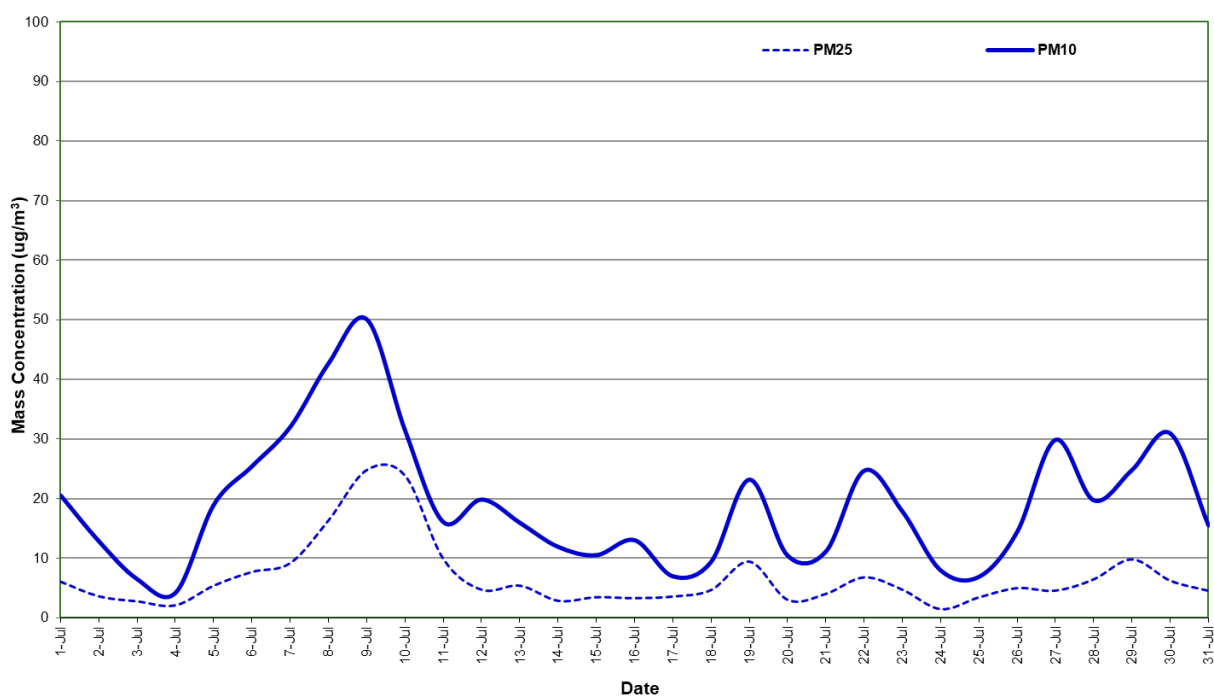
Figure 7: Station 6 PM 2.5 and PM 10 concentration (24 hour average) – July 2021
