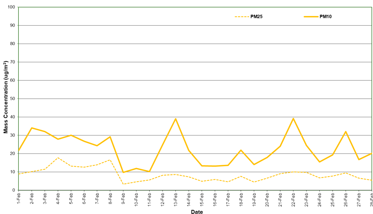
Figure 3: Station 2 PM 2.5 and PM 10 concentration (24 Hour Average) – February 2025
