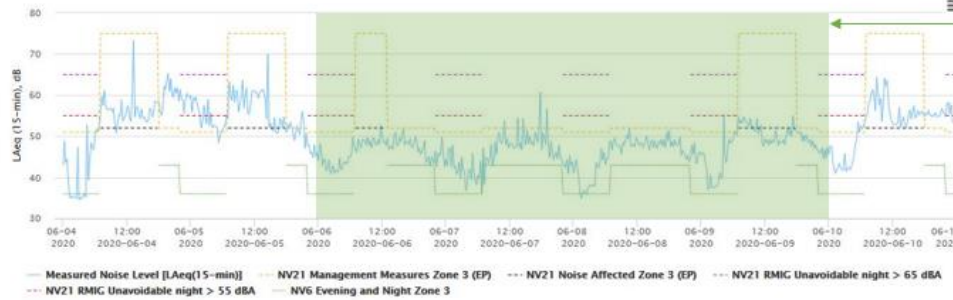
8 William Street, South Yarra: Measured Noise Levels
