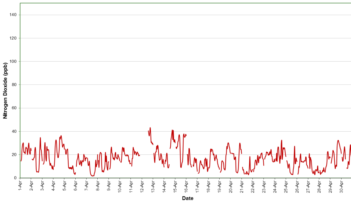
Figure 10: Station 4 NO 2 concentration (1 hour average) – April 2019
