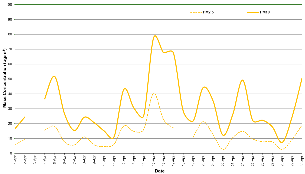
Figure 3: Station 2 PM 2.5 and PM 10 concentration (24 Hour Average) – April 2019
