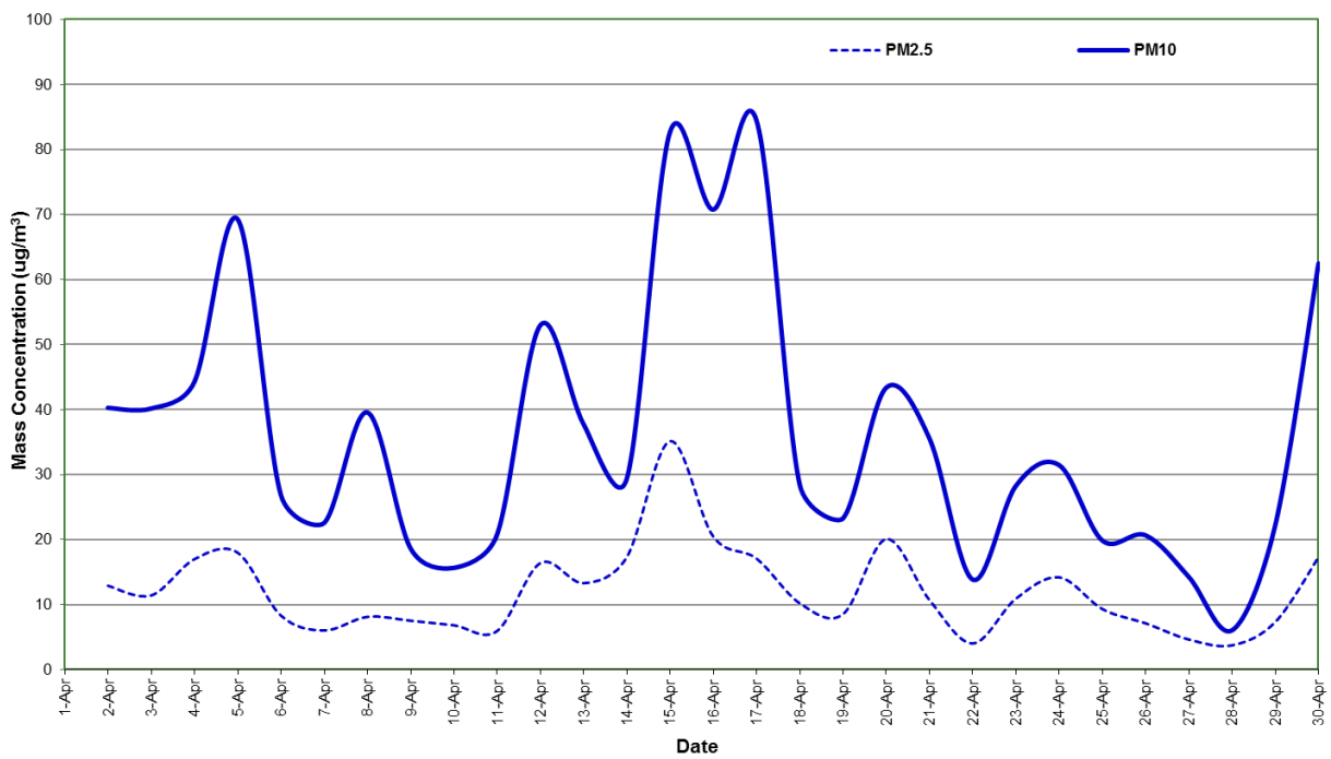
Figure 7: Station 6 PM 2.5 and PM 10 concentration (24 hour average) – April 2019
