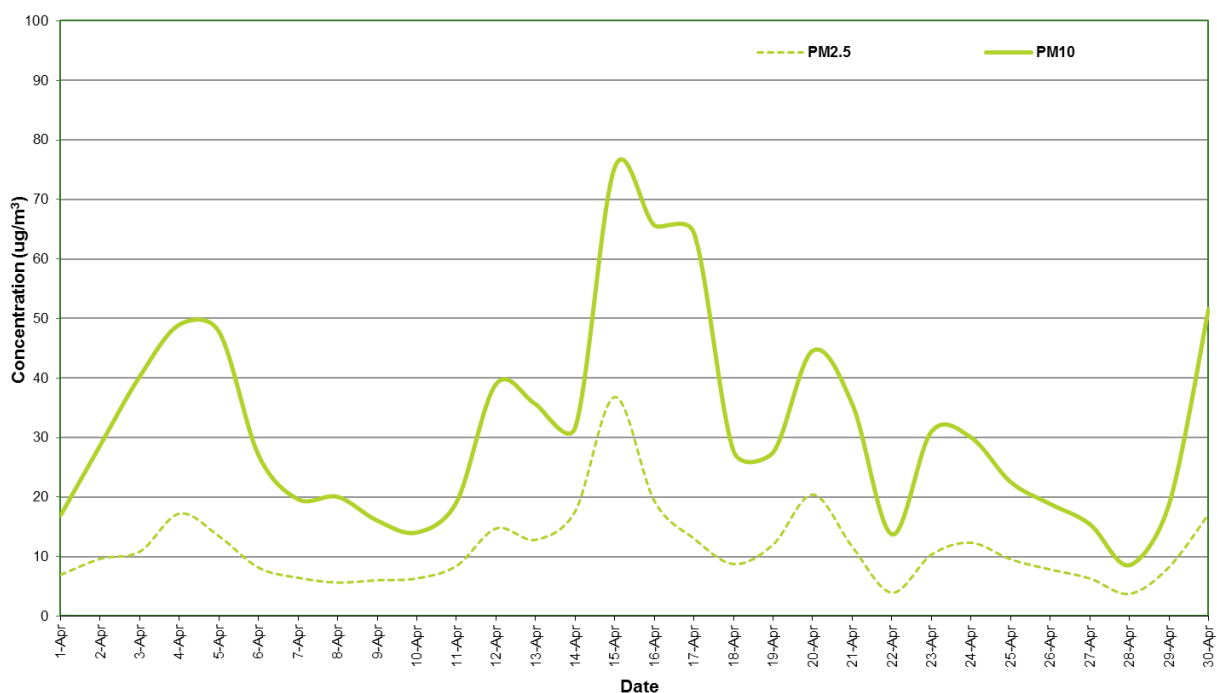
Figure 2: Station 1 PM 2.5 and PM 10 concentration (24 hour average) – April 2019
