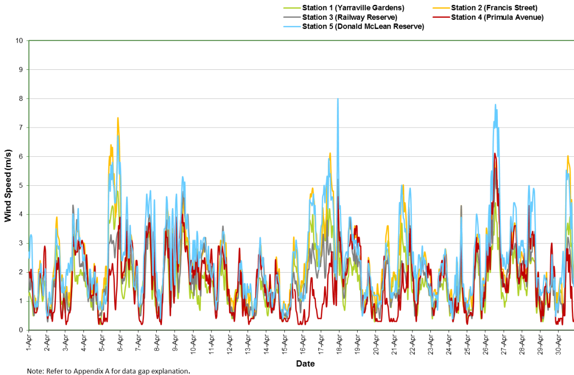
Figure 15: Wind speed (1 hour average) All AAQMS – April 2019
