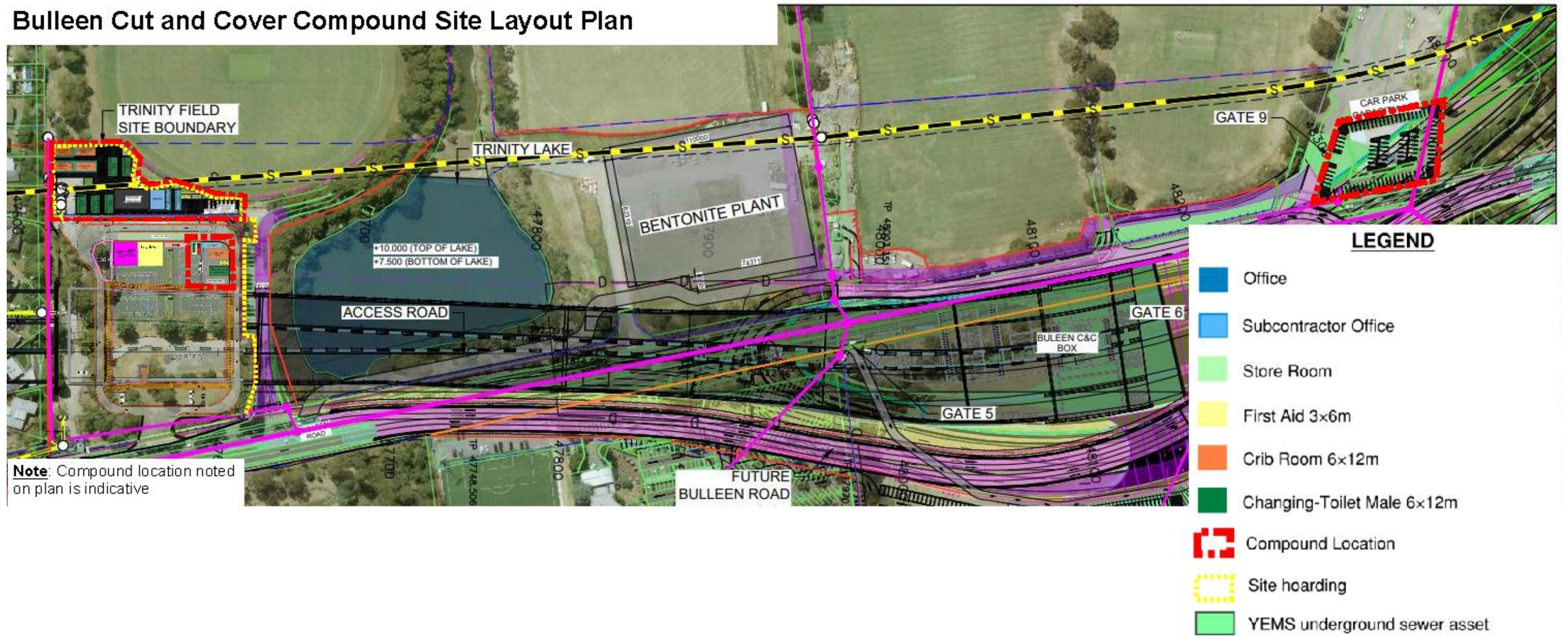
Figure 3: Bulleen Construction Compound Site Layout, Inclusive of Compound Car Park
