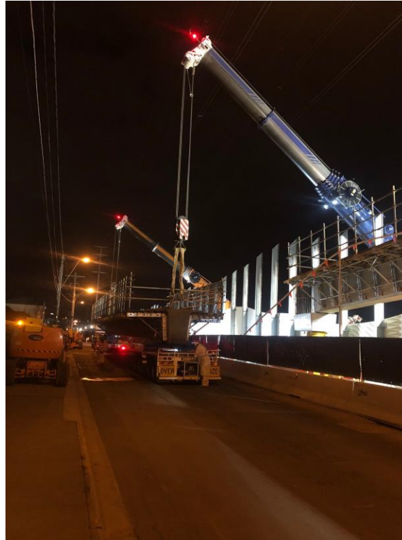
The new overpass ramp sections being lifted into position
