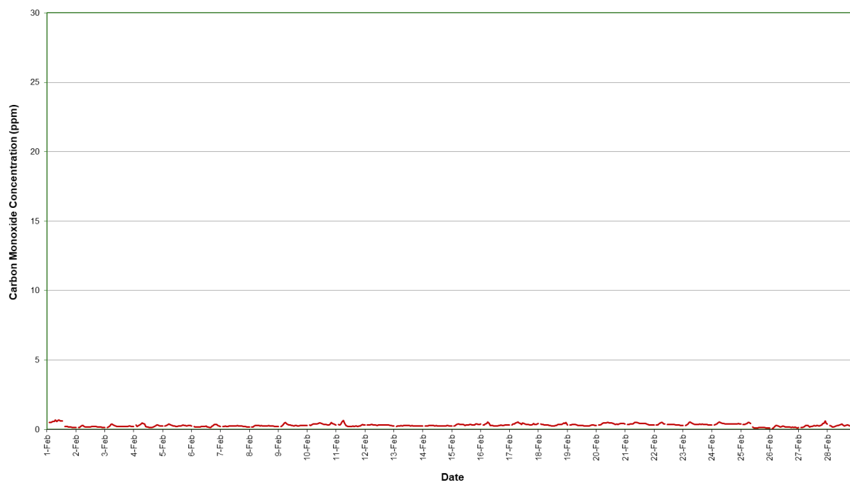
Figure 11: Station 4 CO concentration (1 hour average) – February 2021
