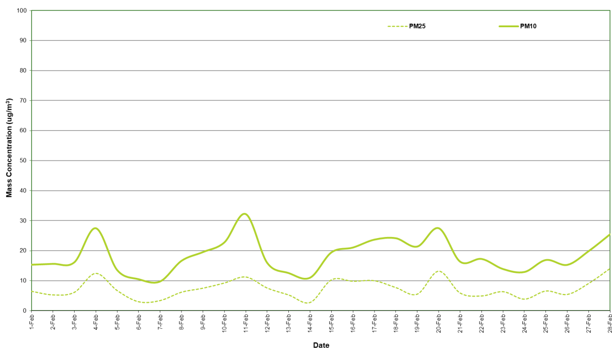
Figure 2: Station 1 PM 2.5 and PM 10 concentration (24 hour average) – February 2021
