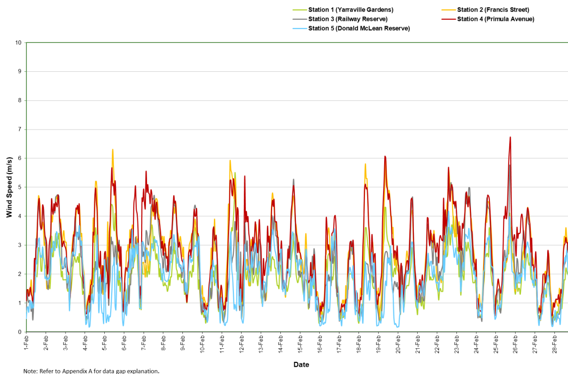
Figure 15: Wind speed (1 hour average) All AAQMs – February 2021
