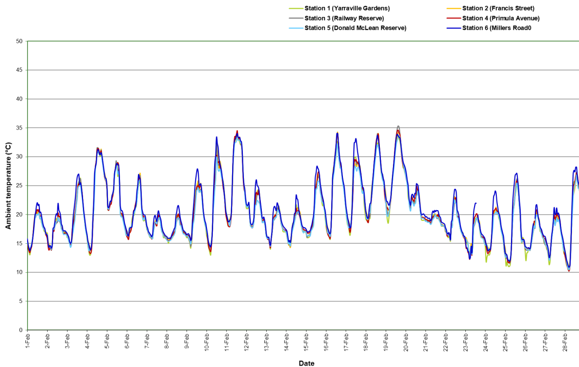
Figure 12: Ambient temperature (1 hour average) All AAQMS – February 2021
