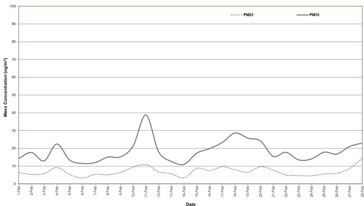
Figure 4: Station 3 PM 2.5 and PM 10 concentration (24 hour average) – February 2021
