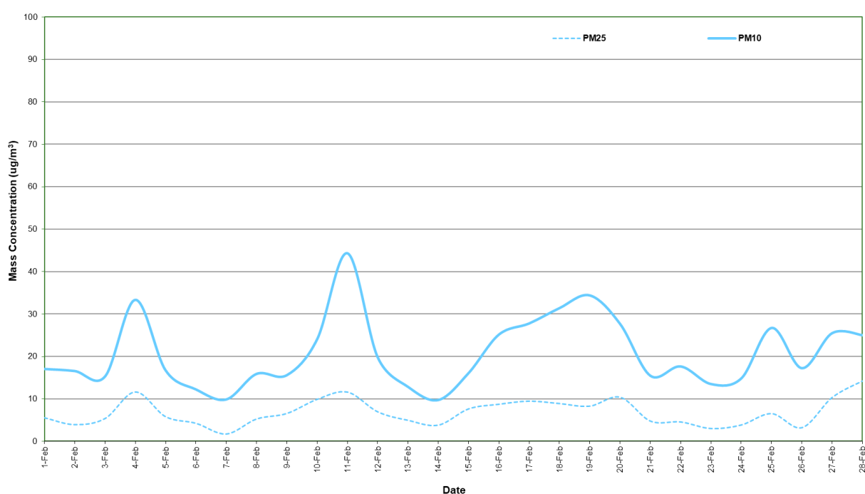
Figure 6: Station 5 PM 2.5 and PM 10 concentration (24 hour average) – February 2021
