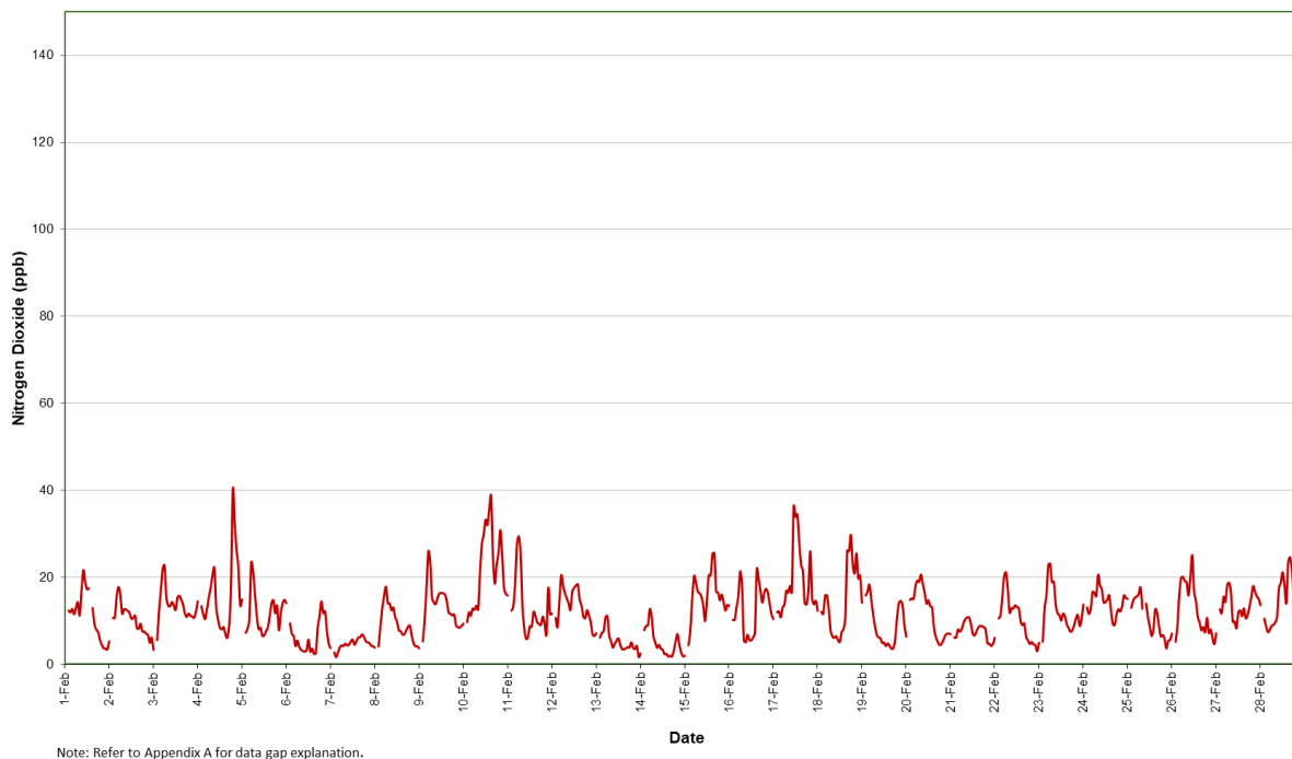
Figure 10: Station 4 NO 2 concentration (1 hour average) – February 2021
