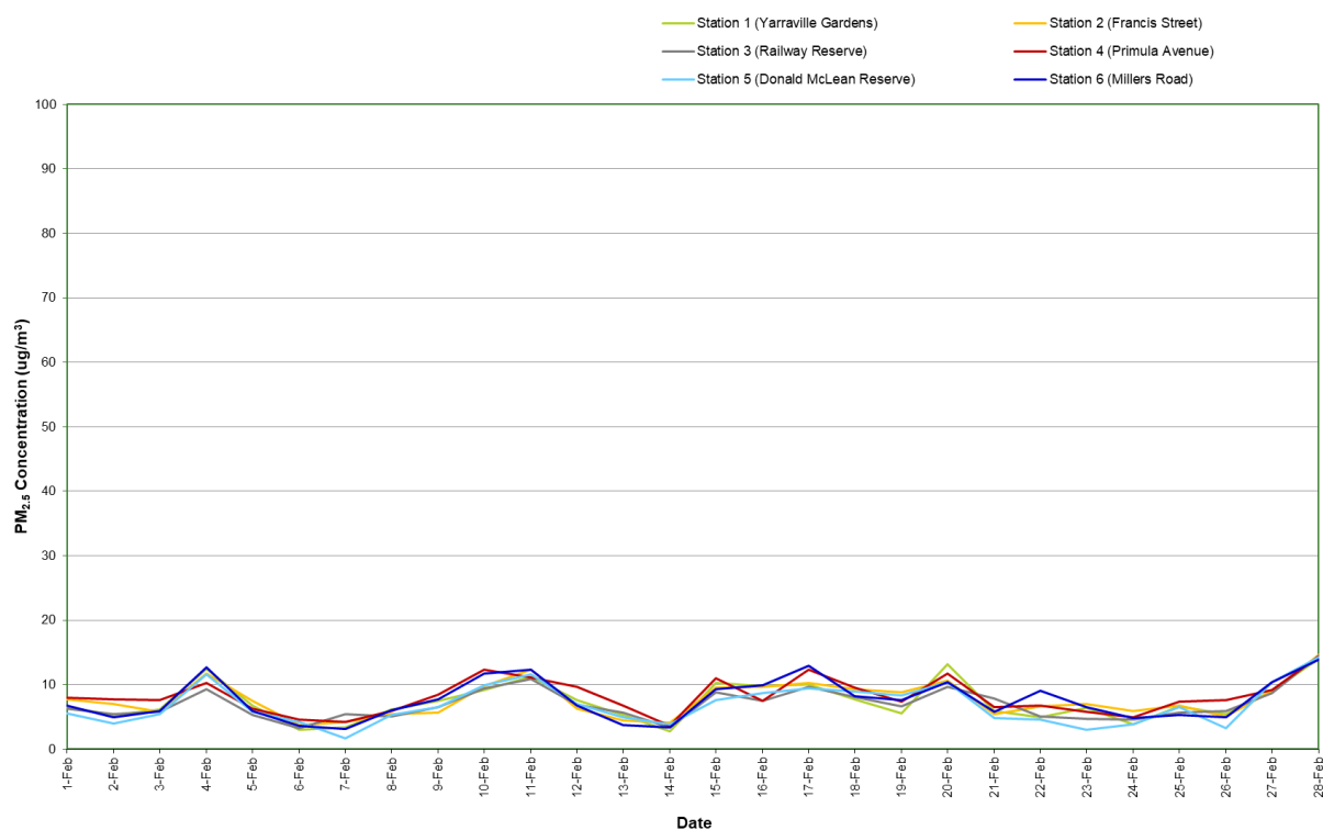
Figure 8: Combined PM 2.5 concentration (24 hour average) – February 2021
