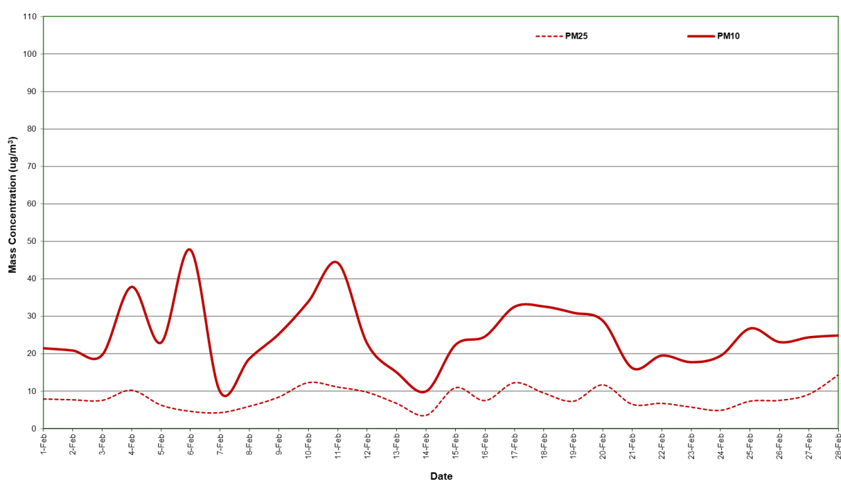
Figure 5: Station 4 PM 2.5 and PM 10 concentration (24 hour average) – February 2021
