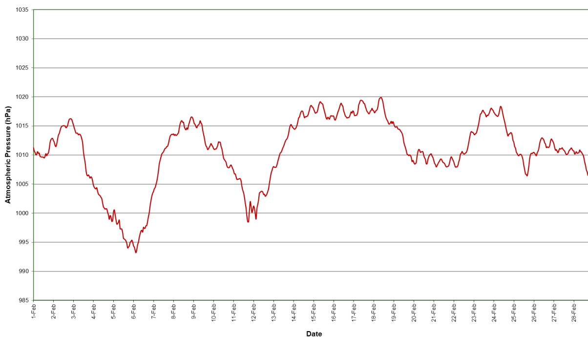
Figure 14: Atmospheric pressure (1 hour average) Station 4 Primula Avenue – February 2021
