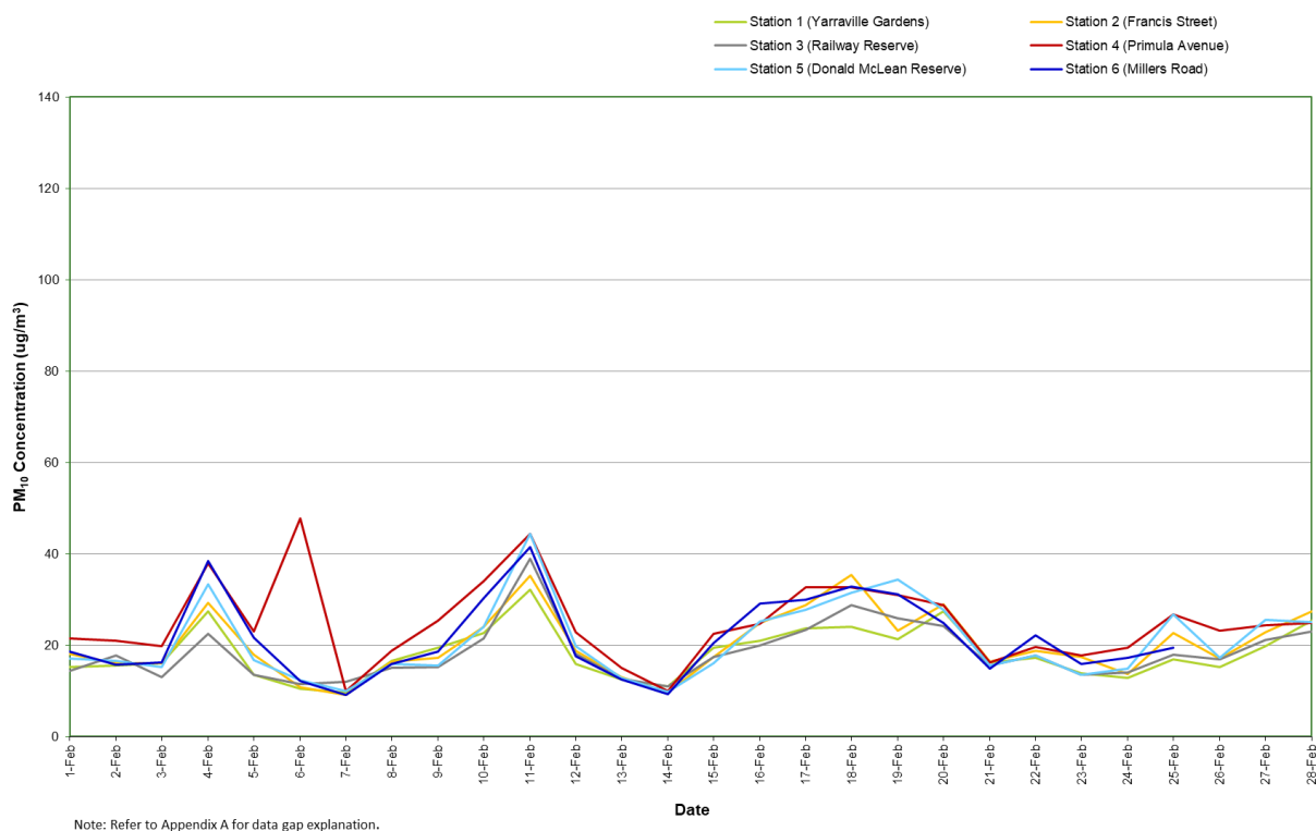
Figure 9: Combined PM 10 concentration (24 hour average) – February 2021
