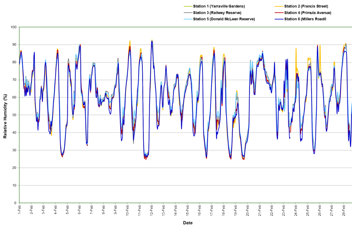
Figure 13: Relative humidity (1 hour average) All AAQMs – February 2021
