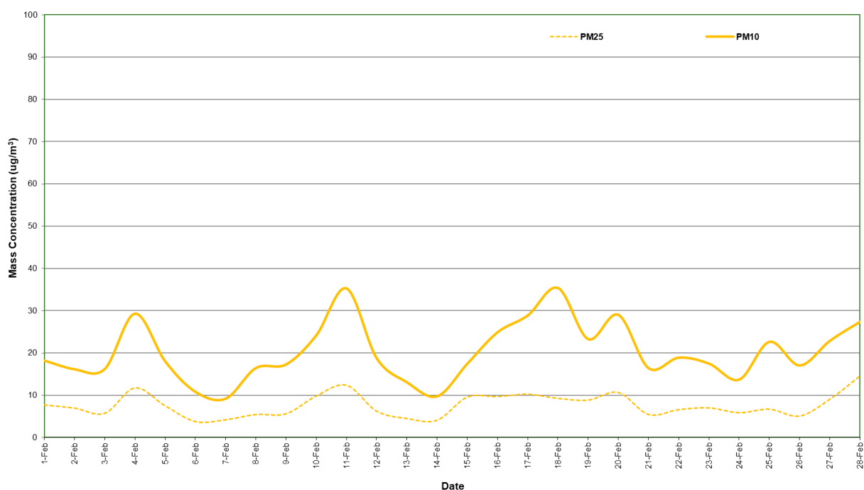
Figure 3: Station 2 PM 2.5 and PM 10 concentration (24 Hour Average) – February 2021
