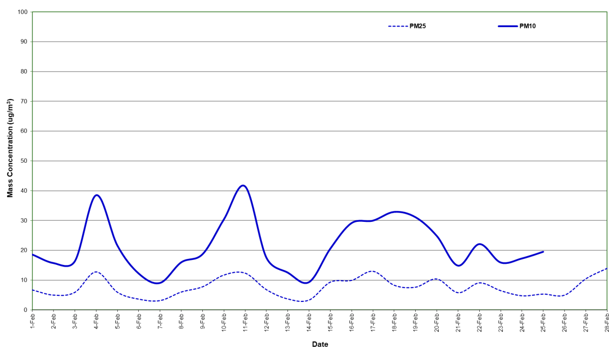
Figure 7: Station 6 PM 2.5 and PM 10 concentration (24 hour average) – February 2021
